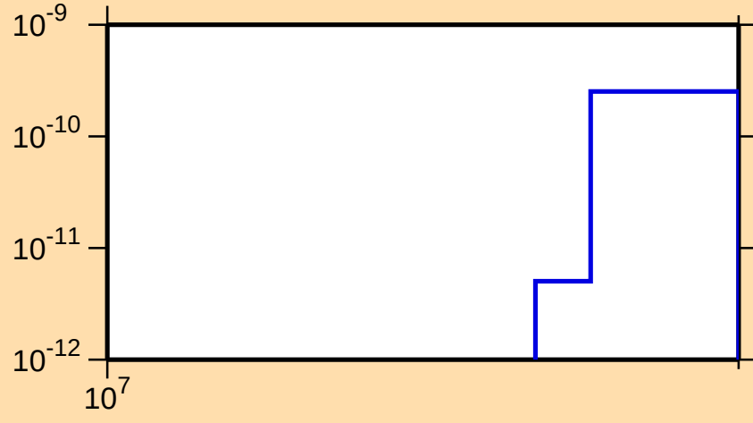
\sigma vs. E for ^{167}\text{Er}(n,\text{He3})
