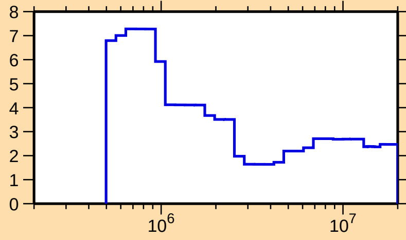
\Delta\sigma/\sigma vs. E for ^{167}\text{Er}(n,n\text{onel.})
