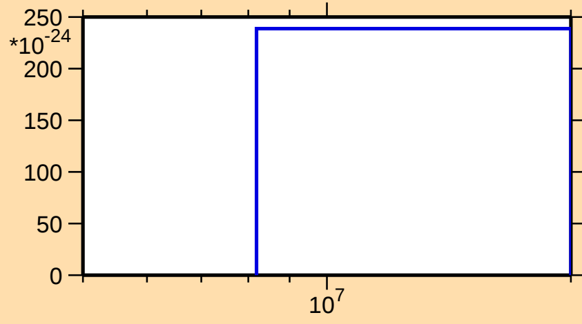
\sigma vs. E for ^{167}\text{Er}(\text{mt 11})
