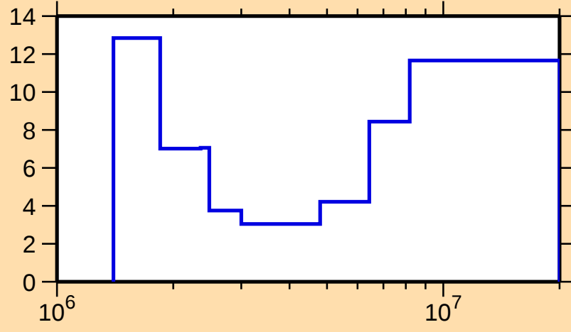
\Delta\sigma/\sigma vs. E for ^{167}\text{Er}(n,n\text{cont.})
