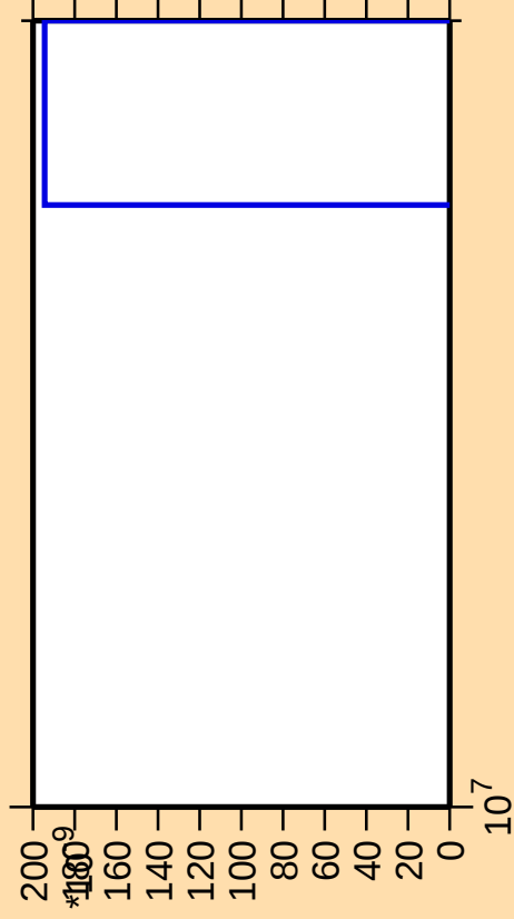
\Delta\sigma/\sigma vs. E for ^{169}\text{Er}(\text{mt 11})
