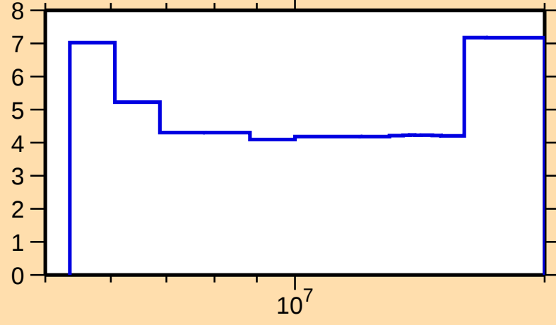
\Delta\sigma/\sigma vs. E for ^{169}\text{Er}(n,\text{tot.})
