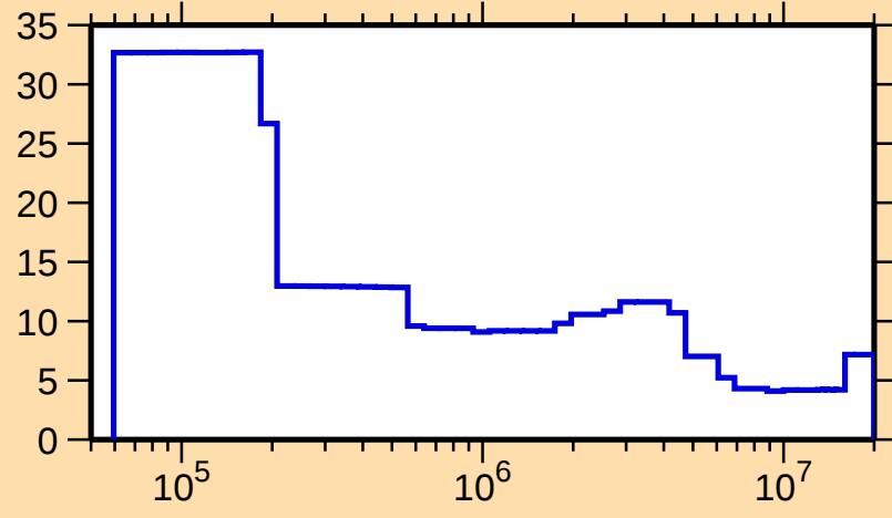
\Delta\sigma/\sigma vs. E for ^{169}\text{Er}(n,\text{tot.})
