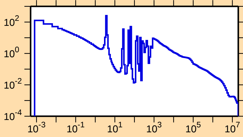
\sigma vs. E for ^{169}\text{Er}(n,\gamma)
