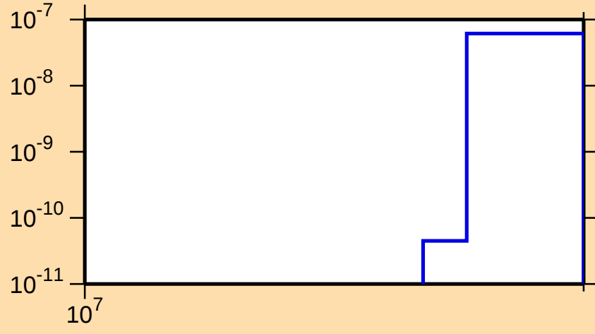
\sigma vs. E for ^{169}\text{Er}(n,nt)
