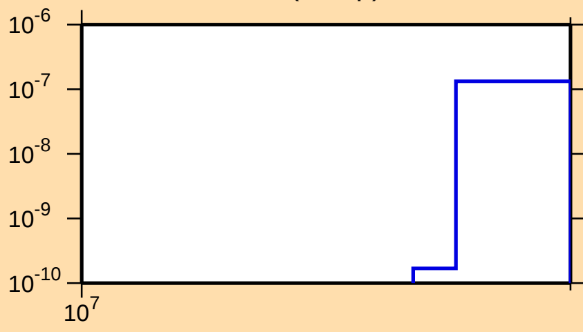
\sigma vs. E for ^{169}\text{Er}(n,2np)
