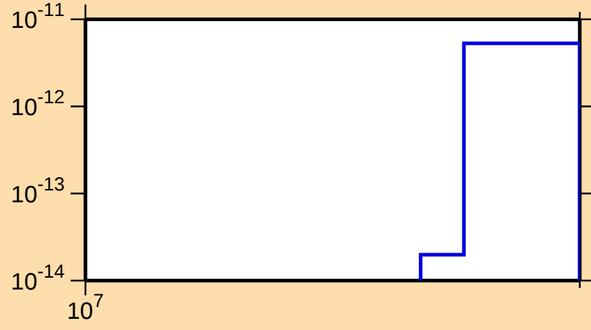
\sigma vs. E for ^{169}\text{Er}(n,\text{He3})
