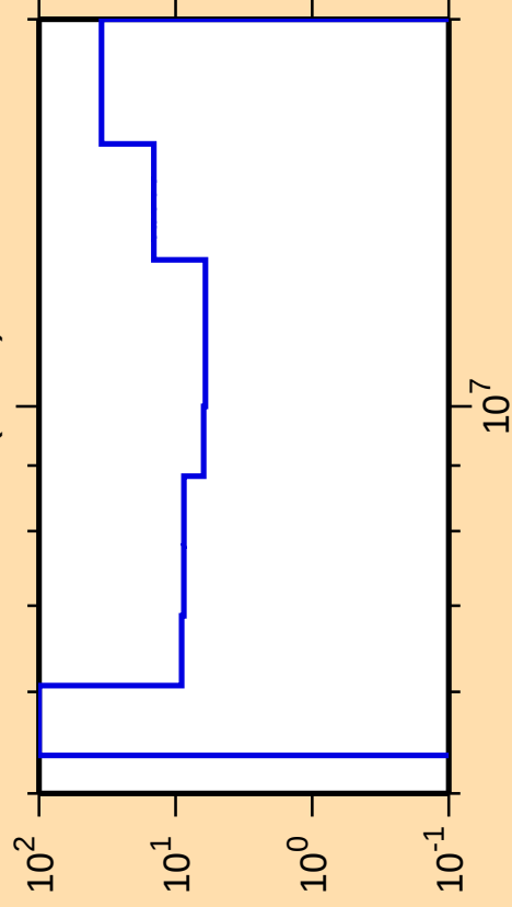
\Delta\sigma/\sigma vs. E for ^{169}\text{Er}(n,2n)
