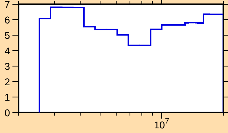
\Delta\sigma/\sigma vs. E for ^{169}\text{Er}(n,\text{nonel.})
