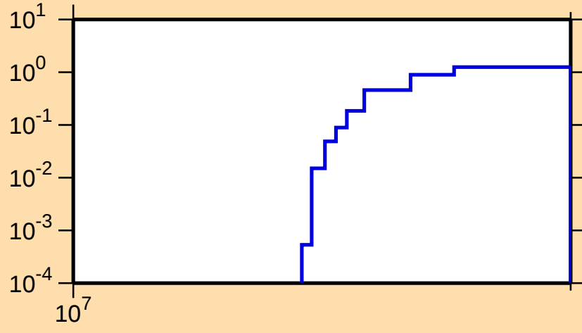
\sigma vs. E for ^{169}\text{Er}(n,3n)
