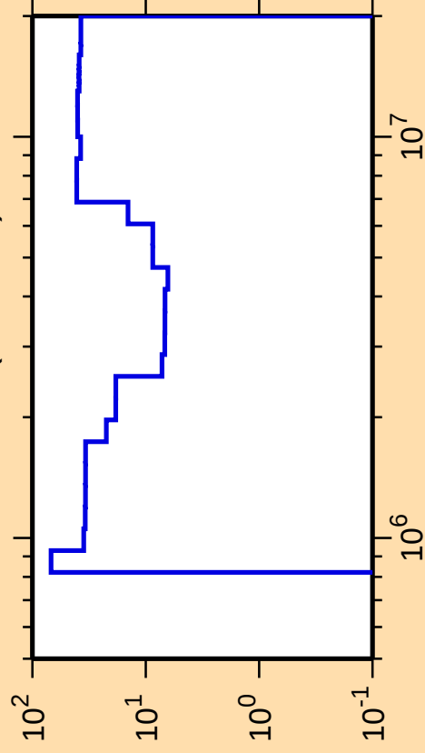
\Delta\sigma/\sigma vs. E for ^{169}\text{Er}(n,n\text{cont.})
