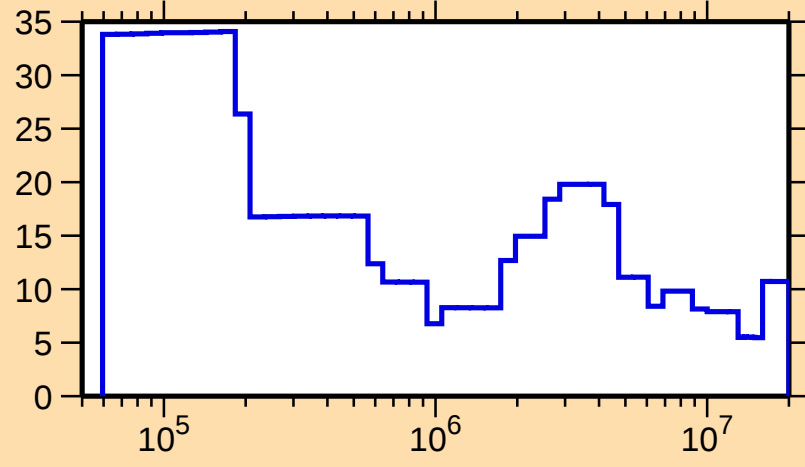
\Delta\sigma/\sigma vs. E for ^{169}\text{Er}(n,\text{el.})
