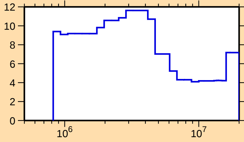
\Delta\sigma/\sigma vs. E for ^{169}\text{Er}(n,\text{tot.})
