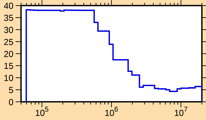
\Delta\sigma/\sigma vs. E for ^{169}\text{Er}(n,\text{nonel.})
