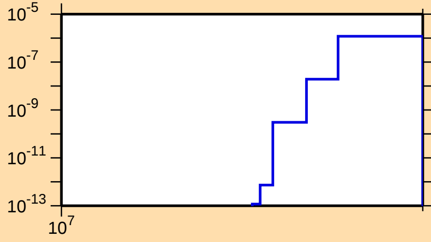
\sigma vs. E for ^{169}\text{Er}(n,\text{nd})
