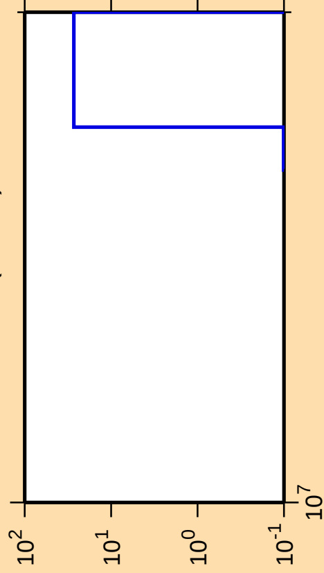
\Delta\sigma/\sigma vs. E for ^{169}\text{Er}(n,\text{He3})
