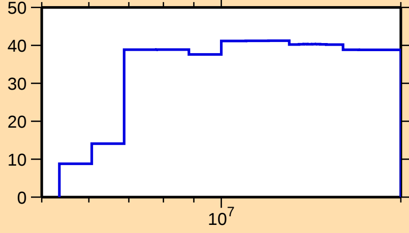
\Delta\sigma/\sigma vs. E for ^{169}\text{Er}(n,\text{inel.})
