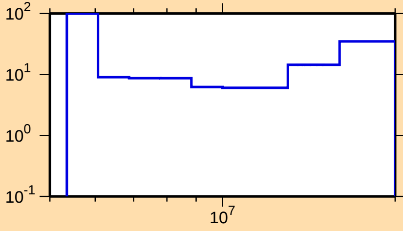
\Delta\sigma/\sigma vs. E for ^{169}\text{Er}(n,2n)
