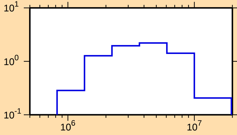
\sigma vs. E for ^{169}\text{Er}(n,n\text{cont.})
