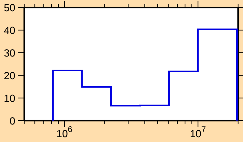
\Delta\sigma/\sigma vs. E for ^{169}\text{Er}(n,\text{inel.})
