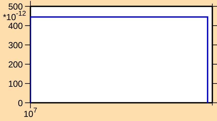
\sigma vs. E for ^{169}\text{Er}(n,nt)
