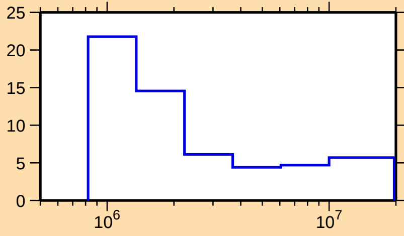
\Delta\sigma/\sigma vs. E for ^{169}\text{Er}(\text{n},\text{nonel.})
