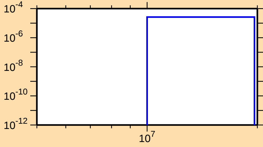
\sigma vs. E for ^{169}\text{Er}(n,t)
