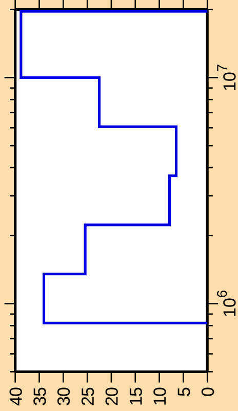
\Delta\sigma/\sigma vs. E for ^{169}\text{Er}(\text{n},\text{ncont.})
