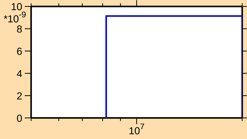
\sigma vs. E for ^{169}\text{Er}(n,2n\alpha)
