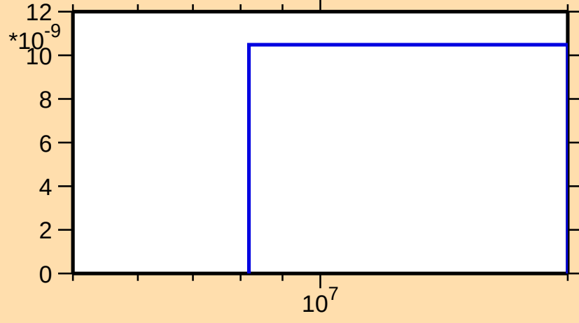
\sigma vs. E for ^{169}\text{Er}(n,\text{nd})
