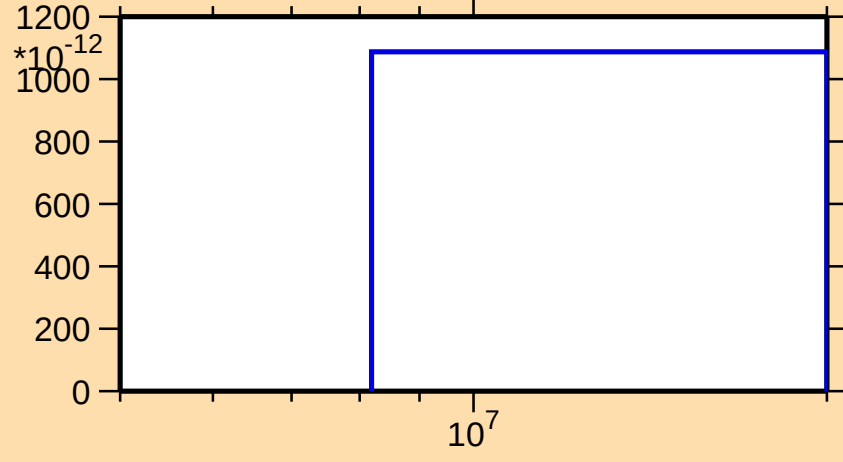
\sigma vs. E for ^{169}\text{Er}(n,2np)
