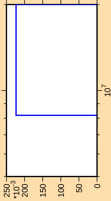
\Delta\sigma/\sigma vs. E for ^{169}\text{Er}(n,\text{He3})
