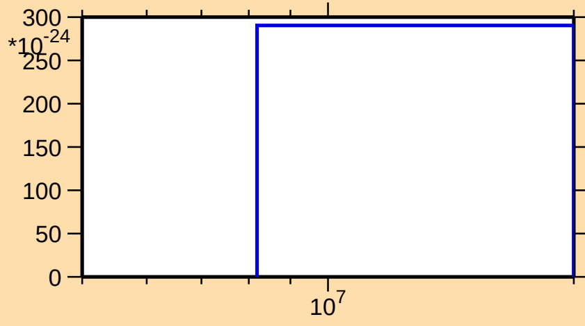
\sigma vs. E for ^{169}\text{Er}(\text{mt 11})
