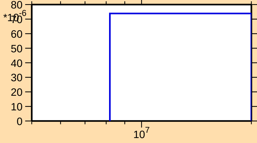
\sigma vs. E for ^{169}\text{Er}(n,np)
