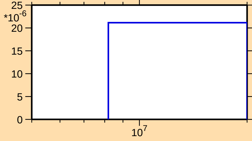
\sigma vs. E for ^{169}\text{Er}(n,t)
