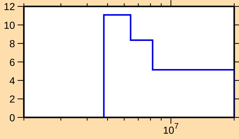
\Delta\sigma/\sigma vs. E for ^{169}\text{Er}(n,\text{el.})
