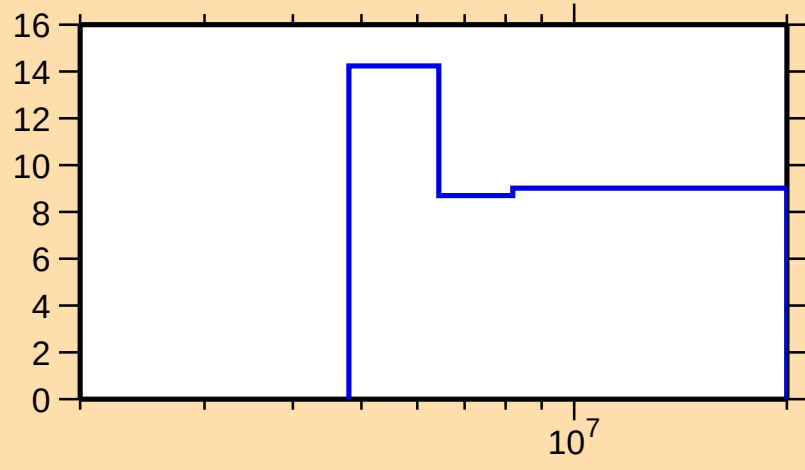
\Delta\sigma/\sigma vs. E for ^{169}\text{Er}(n,2n)
