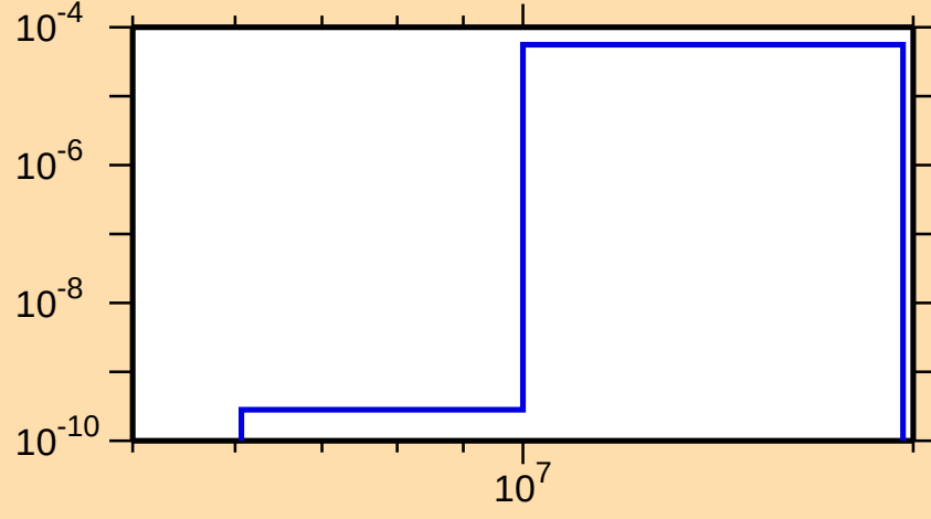
\sigma vs. E for ^{170}\text{Er}(n,n\alpha)
