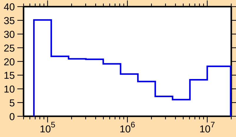
\Delta\sigma/\sigma vs. E for ^{170}\text{Er}(n,\text{inel.})
