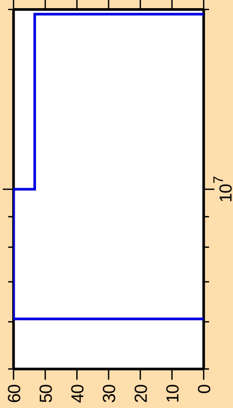
\Delta\sigma/\sigma vs. E for ^{170}\text{Er}(n,n\alpha)
