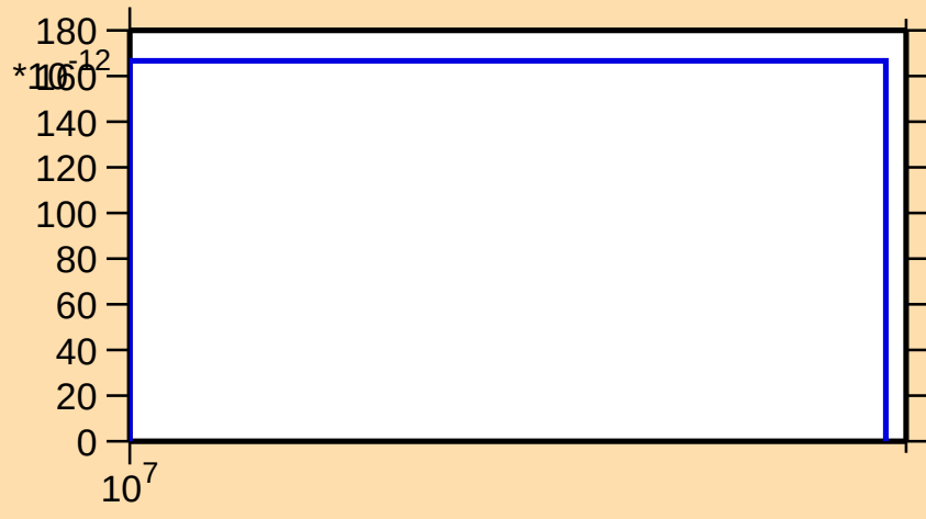
\sigma vs. E for ^{170}\text{Er}(n,\text{nt})
