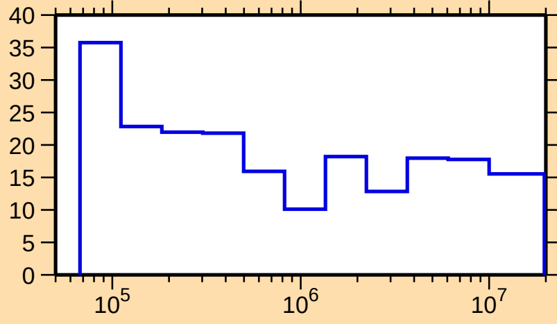
\Delta\sigma/\sigma vs. E for ^{170}\text{Er}(n,n_1)
