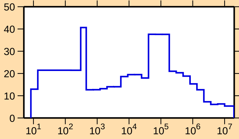
\Delta\sigma/\sigma vs. E for ^{170}\text{Er}(n,\text{nonel.})
