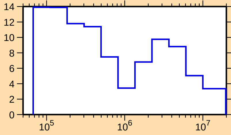
\Delta\sigma/\sigma vs. E for ^{170}\text{Er}(n,\text{tot.})
