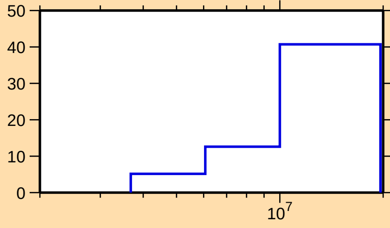
\Delta\sigma/\sigma vs. E for ^{170}\text{Er}(n,n\text{cont.})
