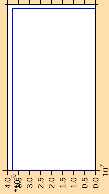
\Delta\sigma/\sigma vs. E for ^{170}\text{Er} (mt 11)
