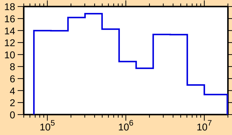
\Delta\sigma/\sigma vs. E for ^{170}\text{Er}(n,\text{el.})
