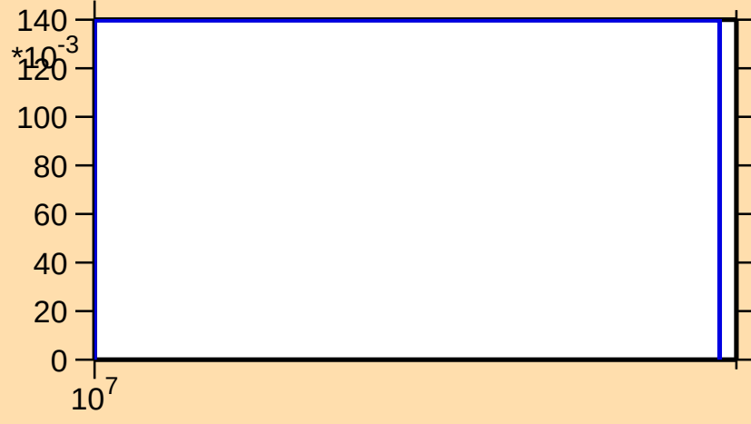
\sigma vs. E for ^{170}\text{Er}(n,3n)
