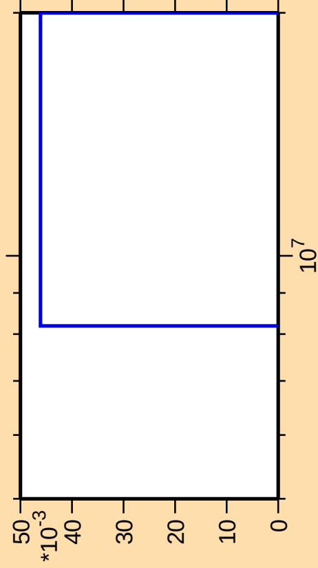
\Delta\sigma/\sigma vs. E for ^{170}\text{Er}(n,\text{He3})
