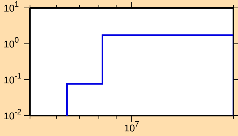
\sigma vs. E for ^{170}\text{Er}(n,2n)
