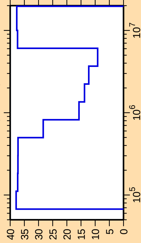
\Delta\sigma/\sigma vs. E for ^{171}\text{Er}(n,\text{inel.})
