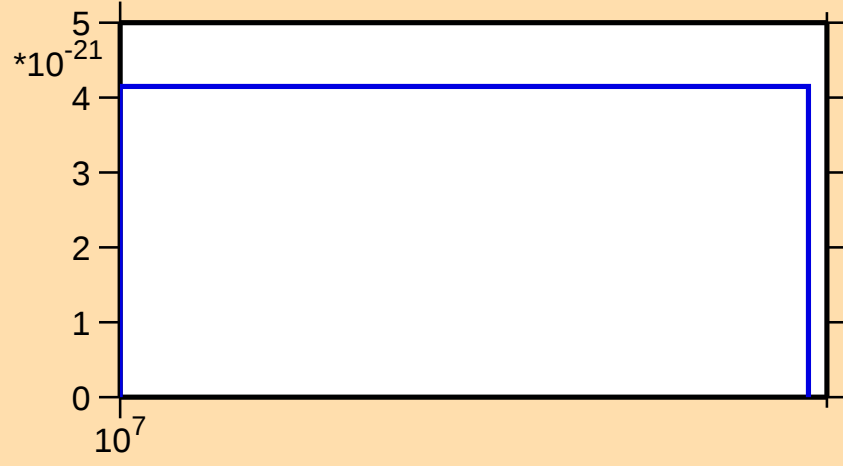
\sigma vs. E for ^{171}\text{Er}(\text{mt } 11)
