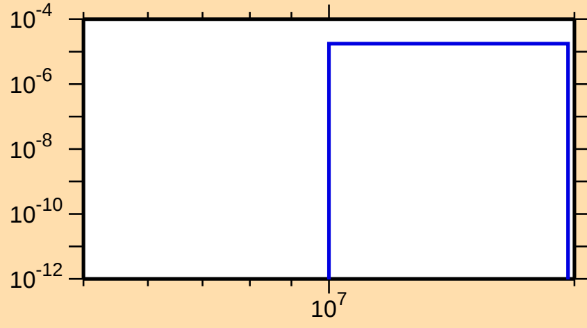
\sigma vs. E for ^{171}\text{Er}(n,t)
