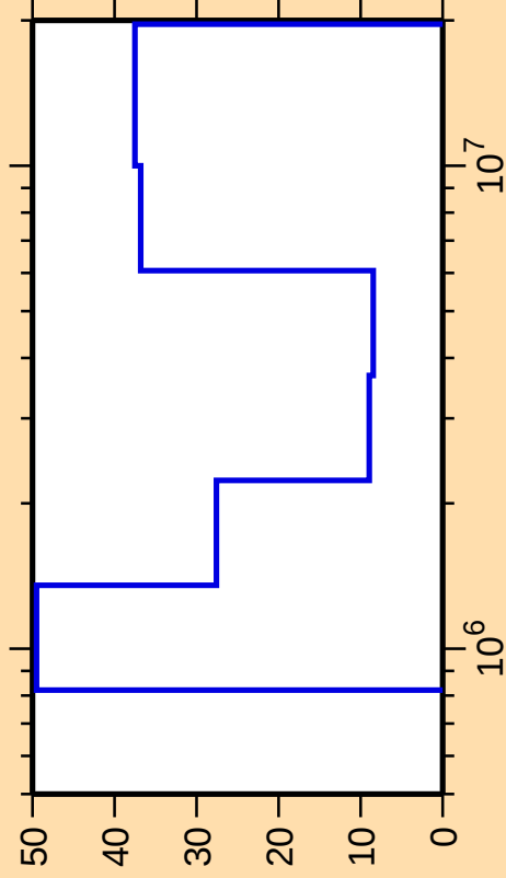
\Delta\sigma/\sigma vs. E for ^{171}\text{Er}(\text{n},\text{ncont.})
