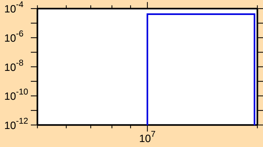
\sigma vs. E for ^{171}\text{Er}(n,np)
