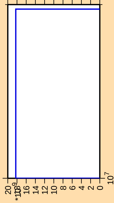
\Delta\sigma/\sigma vs. E for ^{171}\text{Er}(\text{mt } 11)
