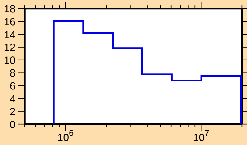
\Delta\sigma/\sigma vs. E for ^{171}\text{Er}(\text{n},\text{nonel.})
