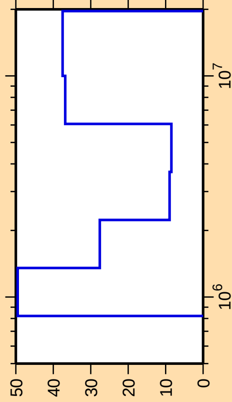
\Delta\sigma/\sigma vs. E for ^{171}\text{Er}(n,\text{ncont.})
