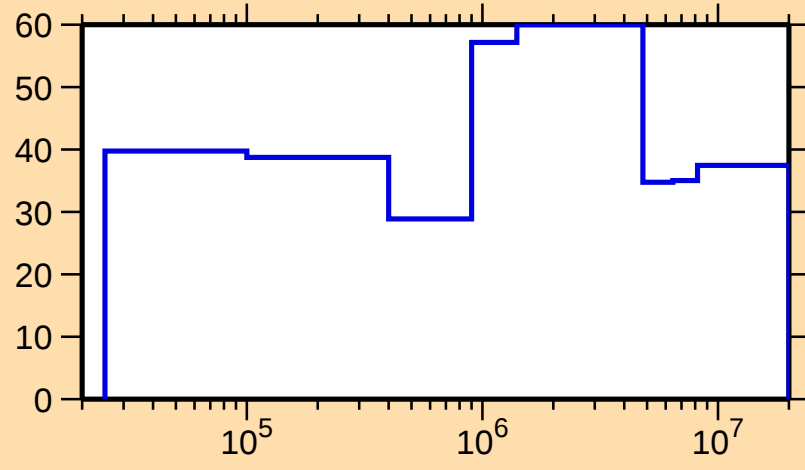
\Delta\sigma/\sigma vs. E for ^{171}\text{Er}(n,n_1)
