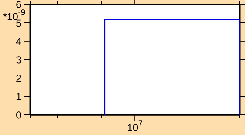
\sigma vs. E for ^{171}\text{Er}(n,\text{nd})
