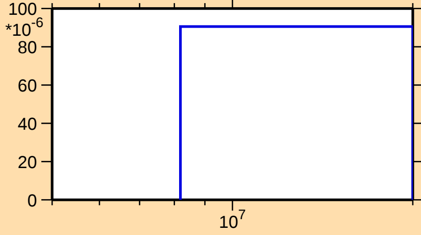
\sigma vs. E for ^{171}\text{Er}(n,d)
