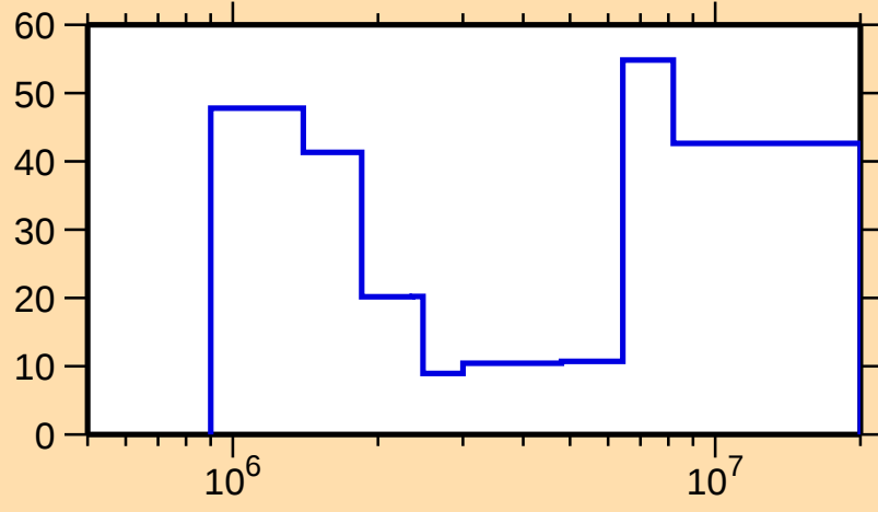
\Delta\sigma/\sigma vs. E for ^{171}\text{Er}(n,n\text{cont.})
