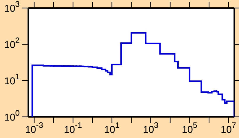
\sigma vs. E for ^{171}\text{Er}(n,\text{el.})
