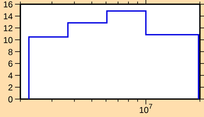
\Delta\sigma/\sigma vs. E for ^{172}\text{Er}(n,n\text{oncl.})
