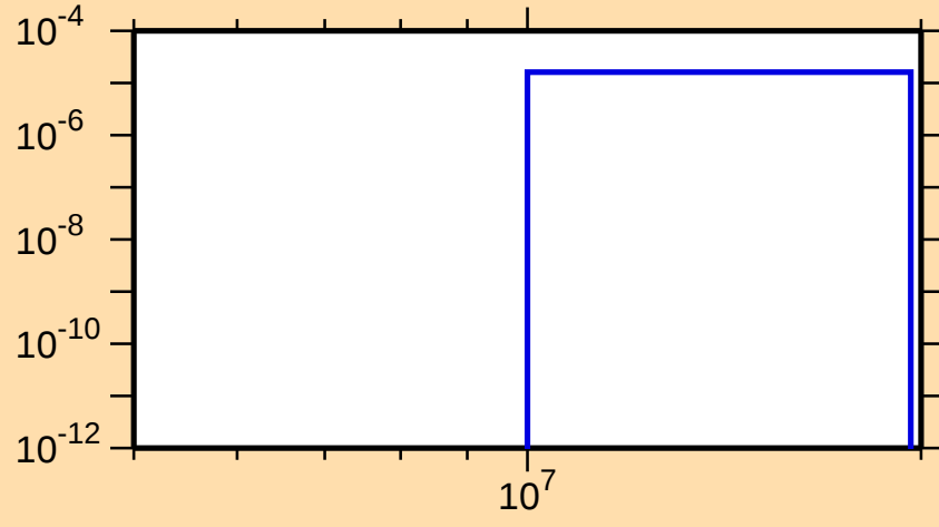
\sigma vs. E for ^{172}\text{Er}(n,np)
