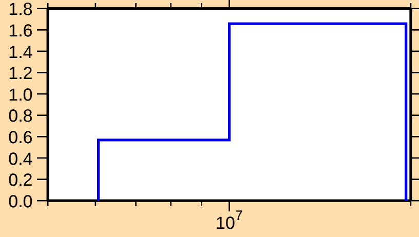
\sigma vs. E for ^{172}\text{Er}(n,2n)
