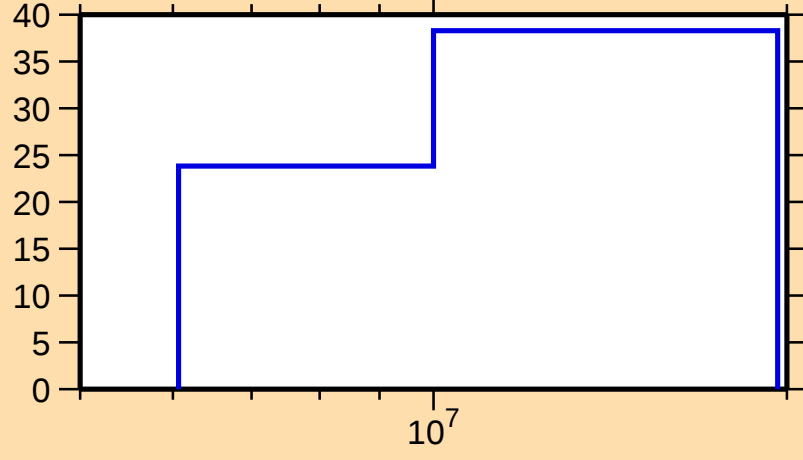
\Delta\sigma/\sigma vs. E for ^{172}\text{Er}(n,\text{ncont.})
