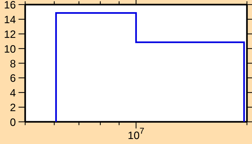
\Delta\sigma/\sigma vs. E for ^{172}\text{Er}(n,\text{nonel.})
