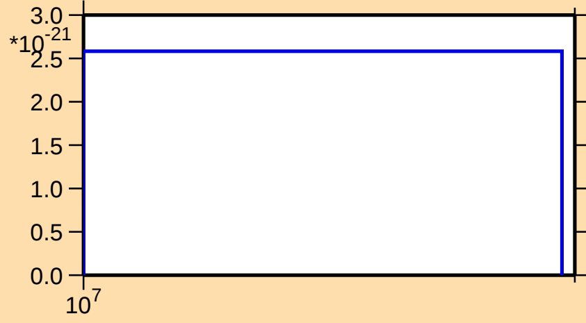
\sigma vs. E for ^{172}\text{Er} (mt 11)
