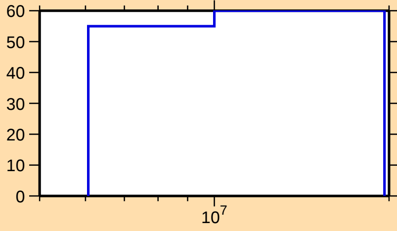
\Delta\sigma/\sigma vs. E for ^{172}\text{Er}(n,\gamma)
