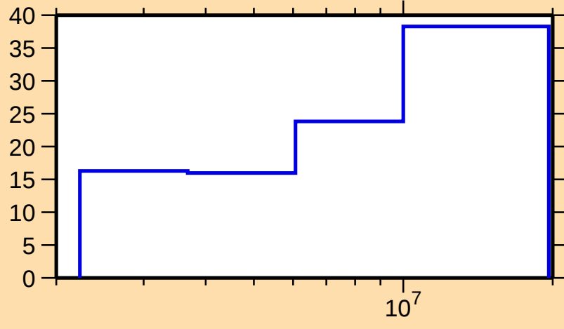
\Delta\sigma/\sigma vs. E for ^{172}\text{Er}(n,n\text{cont.})
