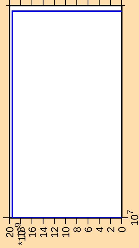
\Delta\sigma/\sigma vs. E for ^{172}\text{Er} (mt 11)
