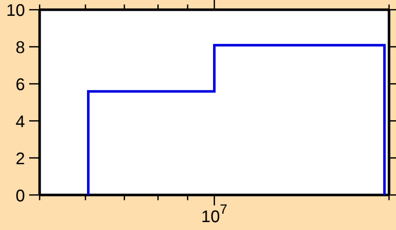
\Delta\sigma/\sigma vs. E for ^{172}\text{Er}(n,\text{tot.})
