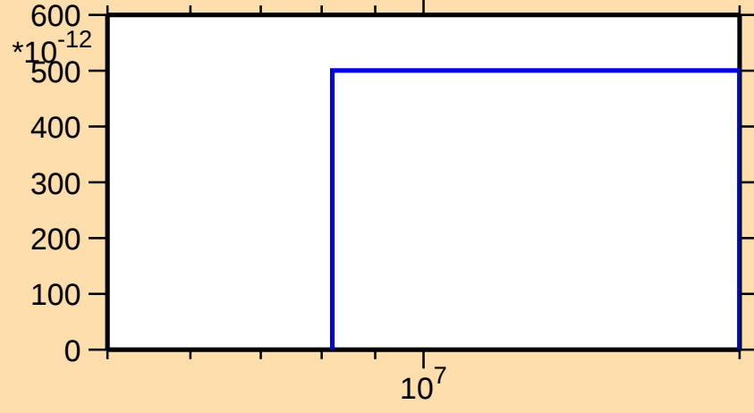
\sigma vs. E for ^{172}\text{Er}(n,nt)
