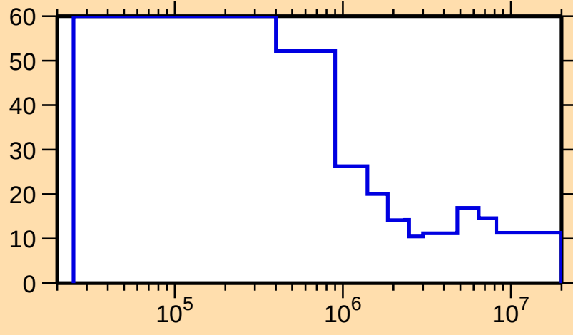
\Delta\sigma/\sigma vs. E for ^{172}\text{Er}(\text{n,nonel.})
