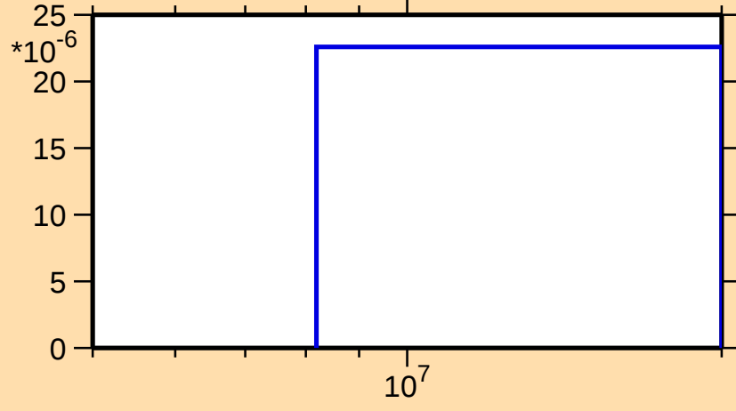
\sigma vs. E for ^{172}\text{Er}(n,d)
