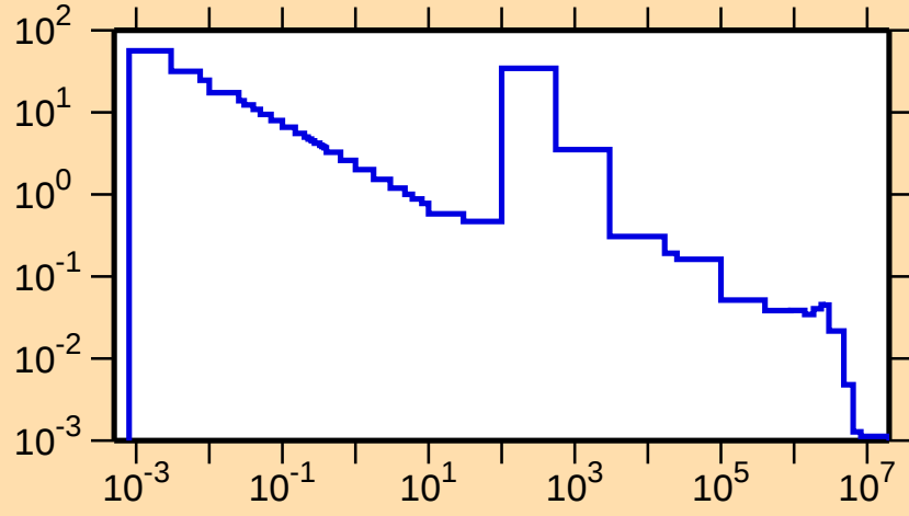
\sigma vs. E for ^{172}\text{Er}(n,\gamma)
