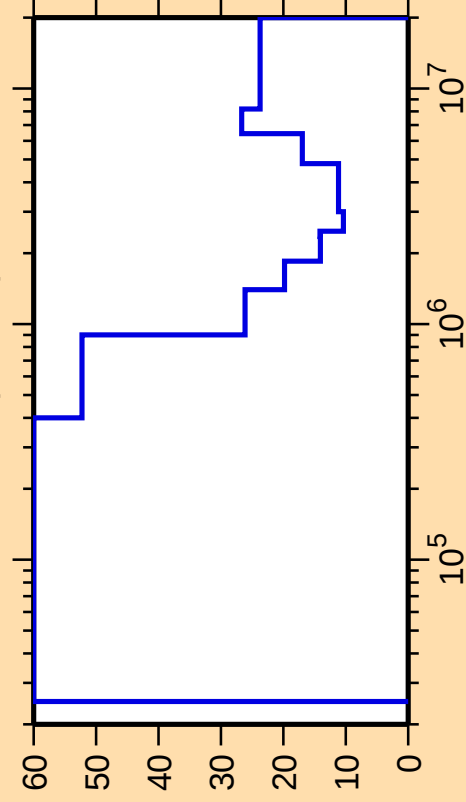
\Delta\sigma/\sigma vs. E for ^{172}\text{Er}(\text{n,inel.})
