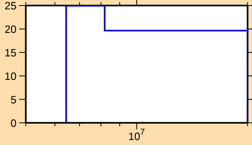
\Delta\sigma/\sigma vs. E for ^{172}\text{Er}(n,\text{el.})
