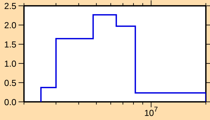
\sigma vs. E for ^{172}\text{Er}(n,n\text{cont.})
