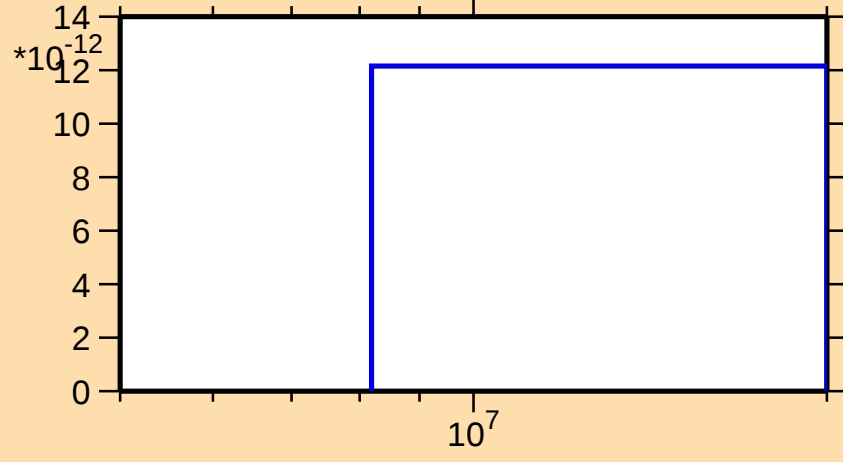
\sigma vs. E for ^{172}\text{Er}(n,2np)
