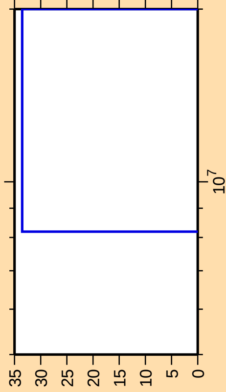
\Delta\sigma/\sigma vs. E for ^{172}\text{Er}(n,3n)
