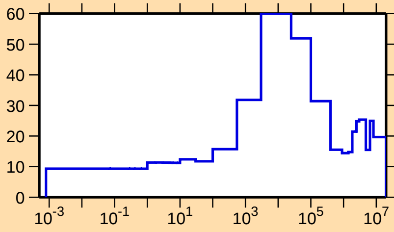
\Delta\sigma/\sigma vs. E for ^{172}\text{Er}(n,\text{el.})
