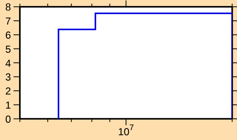
\Delta\sigma/\sigma vs. E for ^{172}\text{Er}(n,\text{tot.})
