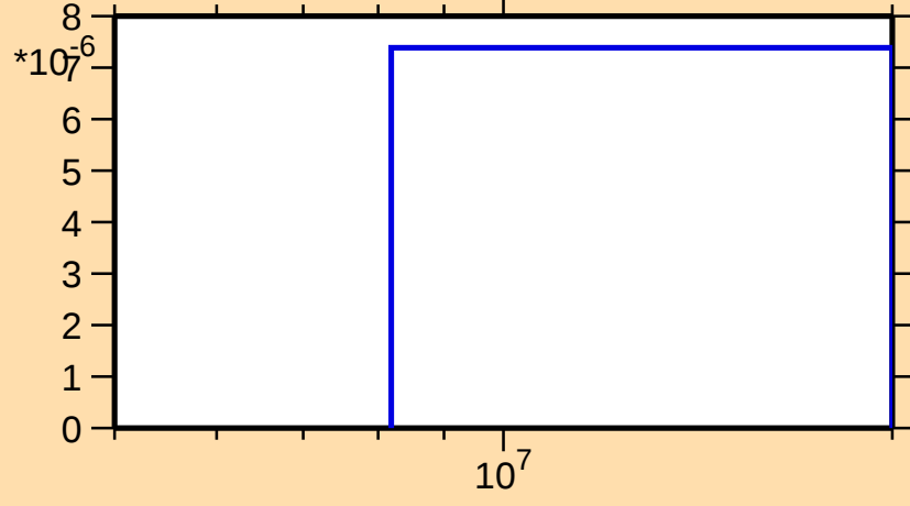
\sigma vs. E for ^{172}\text{Er}(n,t)
