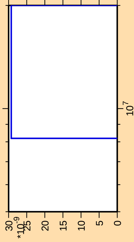
\Delta\sigma/\sigma vs. E for ^{172}\text{Er}(\text{mt } 11)
