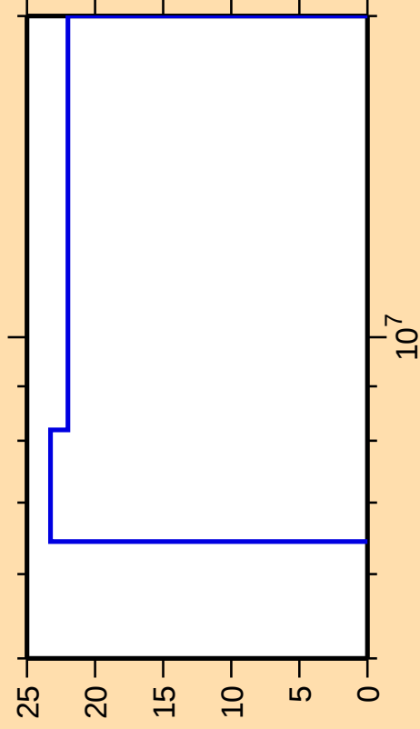
\Delta\sigma/\sigma vs. E for ^{172}\text{Er}(n,2n)
