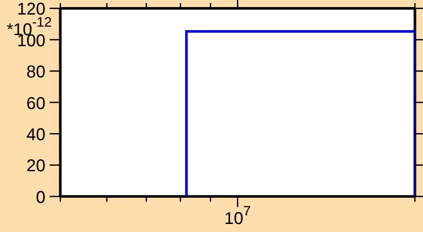
\sigma vs. E for ^{172}\text{Er}(n,2n\alpha)
