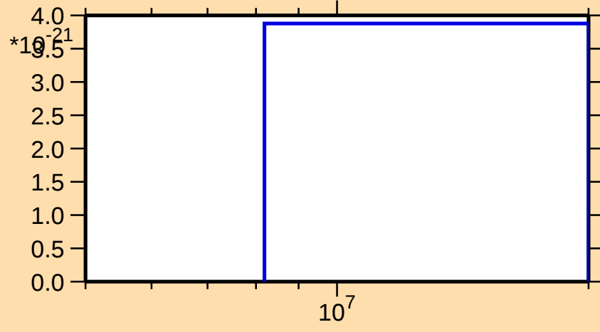
\sigma vs. E for ^{172}\text{Er}(\text{mt } 11)
