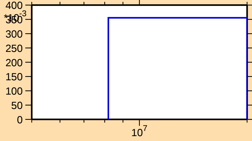
\sigma vs. E for ^{172}\text{Er}(n,3n)
