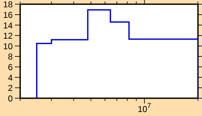
\Delta\sigma/\sigma vs. E for ^{172}\text{Er}(\text{n},\text{nonel.})
