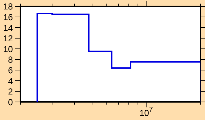
\Delta\sigma/\sigma vs. E for ^{172}\text{Er}(n,\text{tot.})
