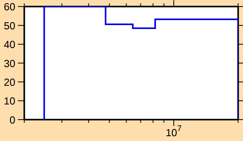
\Delta\sigma/\sigma vs. E for ^{172}\text{Er}(n,n_1)
