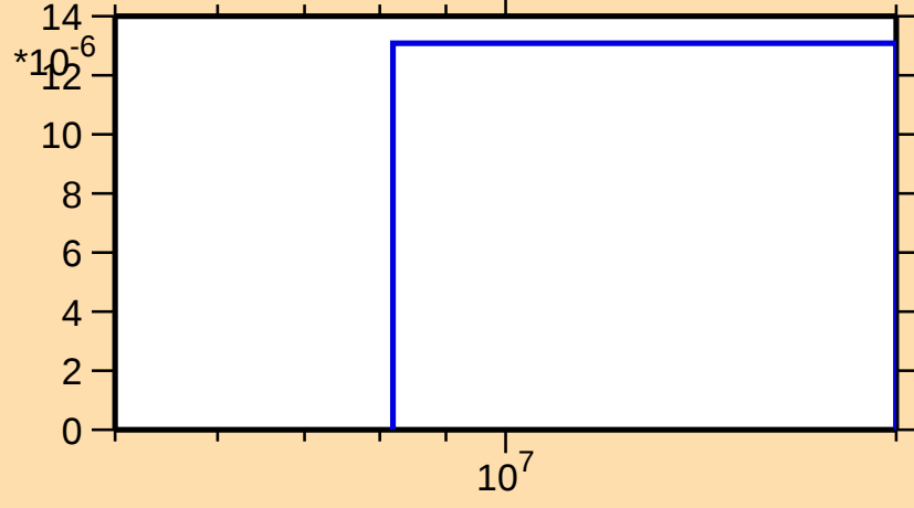
\sigma vs. E for ^{172}\text{Er}(n,np)
