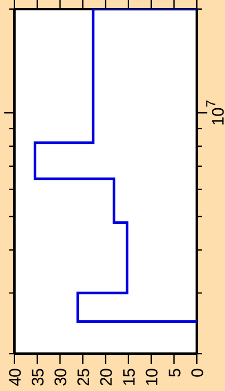
\Delta\sigma/\sigma vs. E for ^{172}\text{Er}(n,\text{ncont.})
