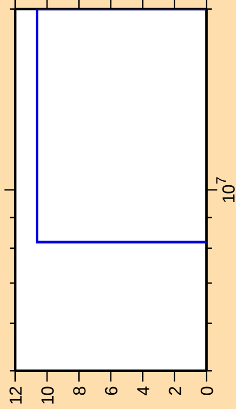
\Delta\sigma/\sigma vs. E for ^{172}\text{Er}(n,2np)
