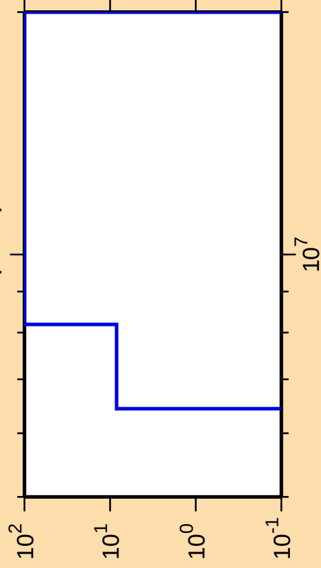
\Delta\sigma/\sigma vs. E for ^{172}\text{Er}(n,n\alpha)
