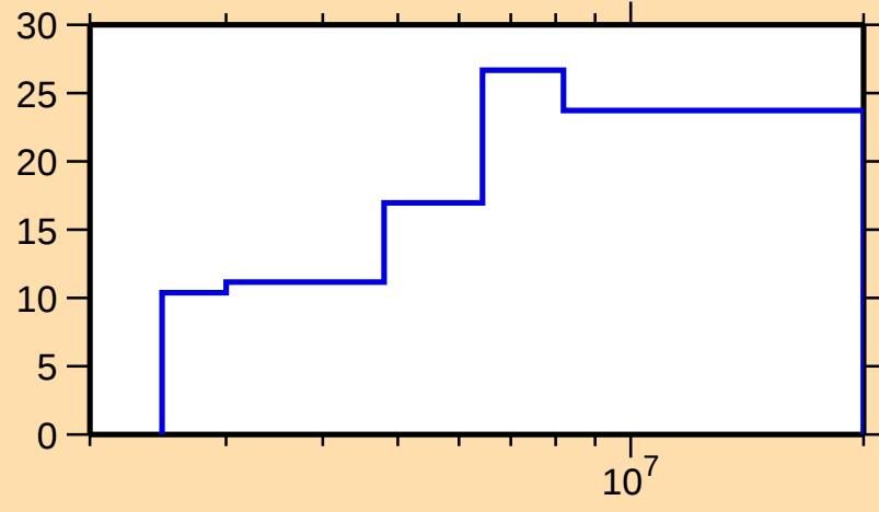
\Delta\sigma/\sigma vs. E for ^{172}\text{Er}(n,\text{inel.})
