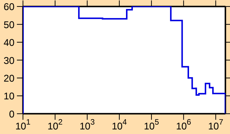
\Delta\sigma/\sigma vs. E for ^{172}\text{Er}(n,\text{nonel.})
