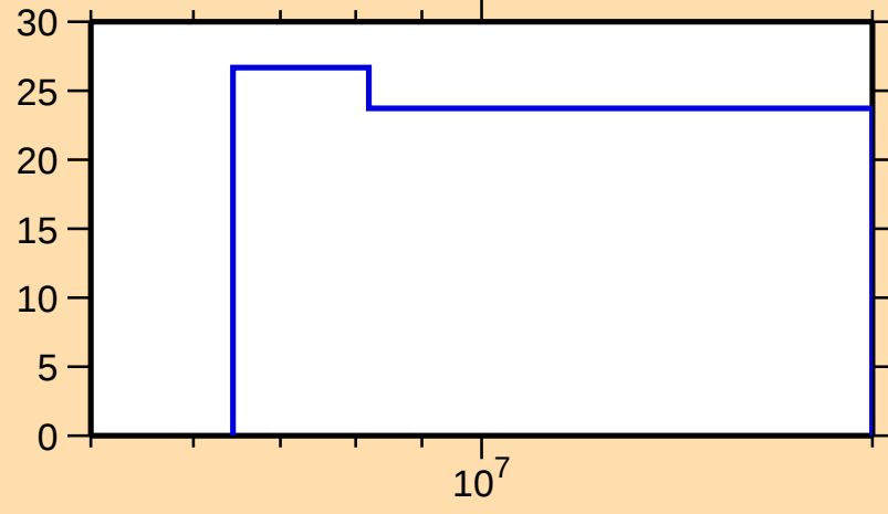
\Delta\sigma/\sigma vs. E for ^{172}\text{Er}(n,\text{inel.})
