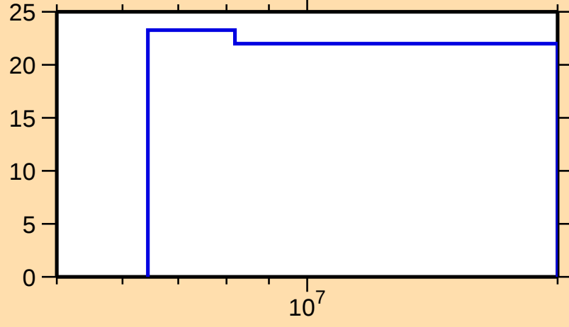
\Delta\sigma/\sigma vs. E for ^{172}\text{Er}(n,2n)
