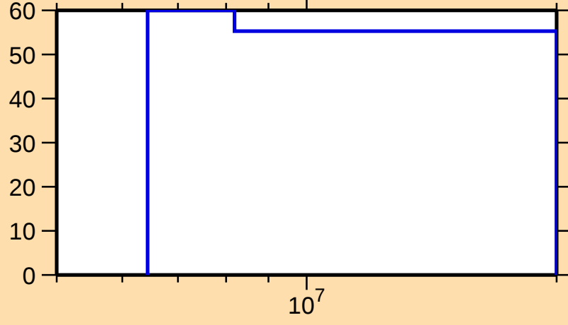
\Delta\sigma/\sigma vs. E for ^{172}\text{Er}(n,p)
