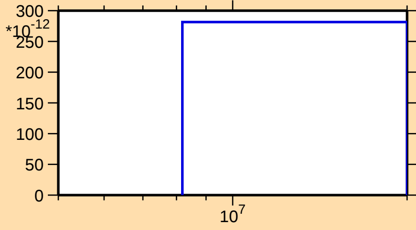
\sigma vs. E for ^{172}\text{Er}(n,\text{nd})
