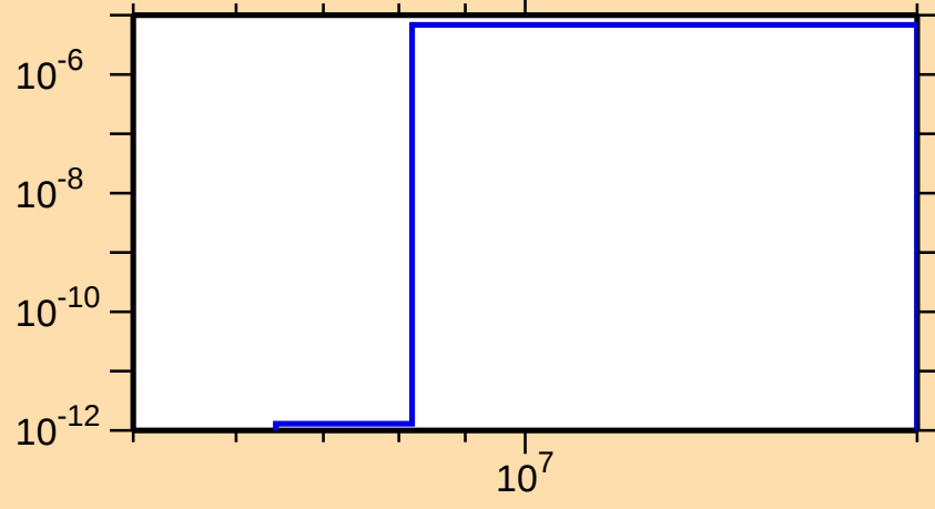
\sigma vs. E for ^{172}\text{Er}(n,n\alpha)
