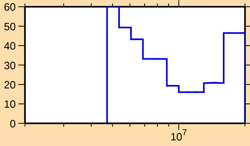
\Delta\sigma/\sigma vs. E for ^{173}\text{Er}(n,2n)
