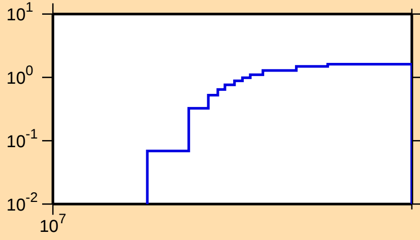
\sigma vs. E for ^{173}\text{Er}(n,3n)
