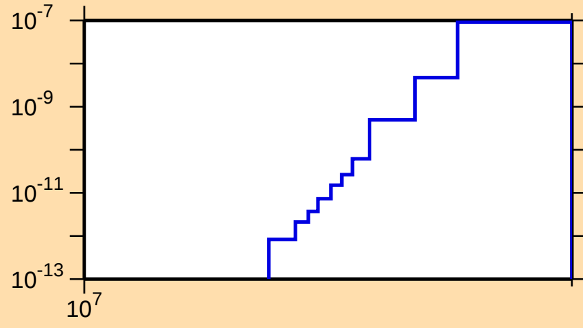
\sigma vs. E for ^{173}\text{Er}(n,2n\alpha)
