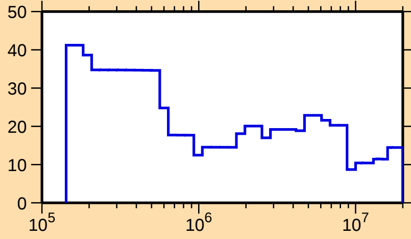
\Delta\sigma/\sigma vs. E for ^{173}\text{Er}(n,\text{tot.})
