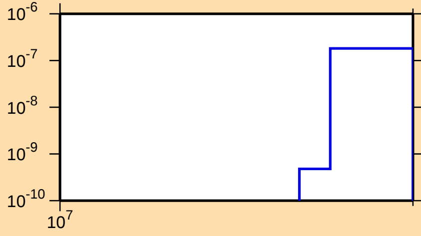
\sigma vs. E for ^{173}\text{Er}(n,nt)
