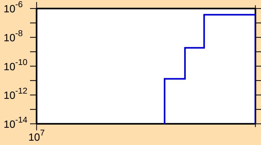
\sigma vs. E for ^{173}\text{Er}(n,\text{nd})
