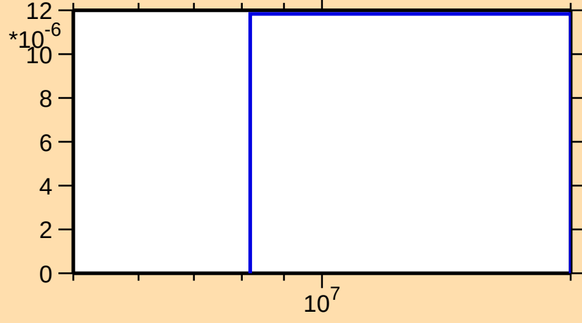
\sigma vs. E for ^{173}\text{Er}(n,np)
