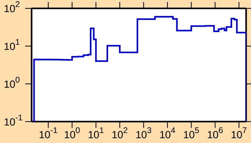
\Delta\sigma/\sigma vs. E for ^{173}\text{Er}(n,\text{el.})
