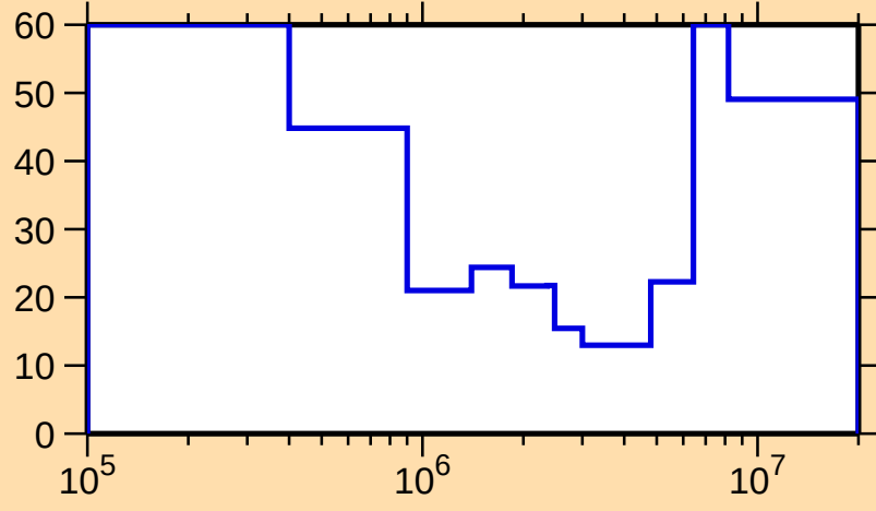
\Delta\sigma/\sigma vs. E for ^{173}\text{Er}(n,n\text{cont.})
