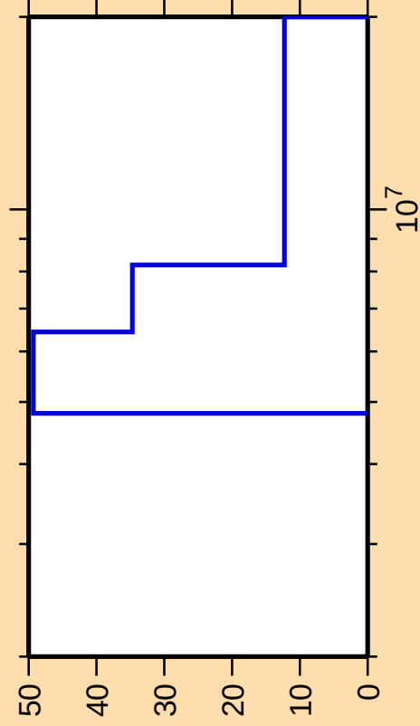
\Delta\sigma/\sigma vs. E for ^{173}\text{Er}(n,2n)
