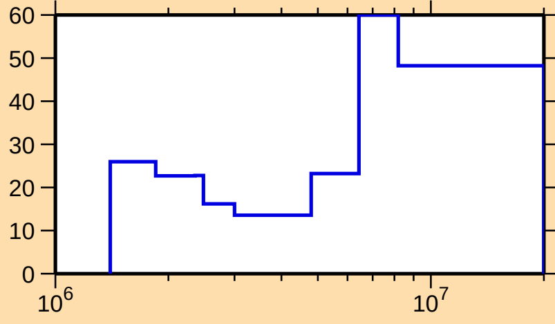
\Delta\sigma/\sigma vs. E for ^{173}\text{Er}(n,\text{inel.})
