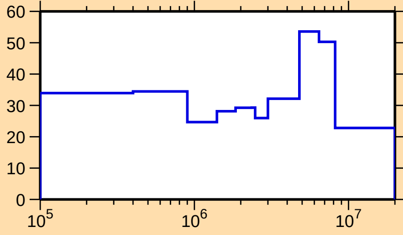
\Delta\sigma/\sigma vs. E for ^{173}\text{Er}(\text{n,el.})
