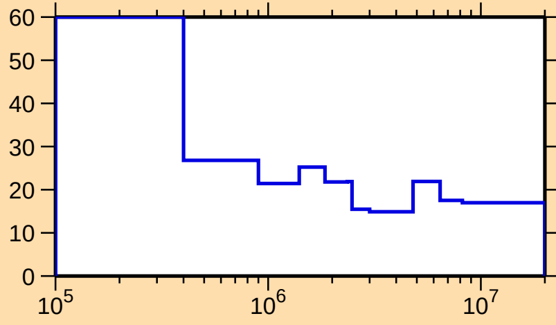
\Delta\sigma/\sigma vs. E for ^{173}\text{Er}(n,\text{nonel.})
