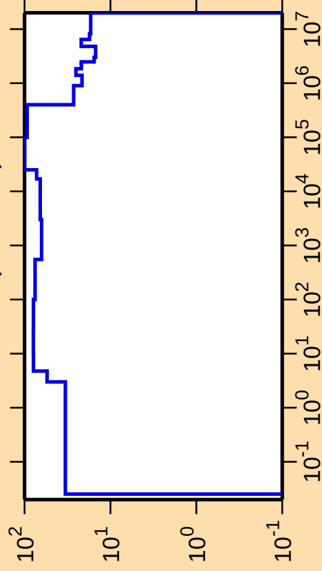
\Delta\sigma/\sigma vs. E for ^{173}\text{Er}(n,\text{nonel.})
