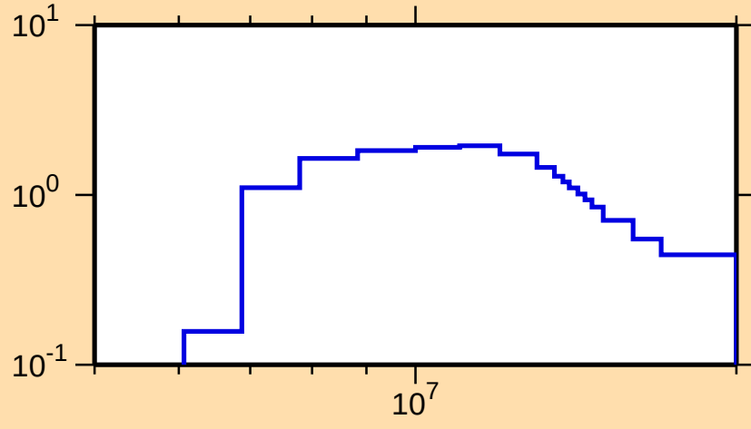
\sigma vs. E for ^{174}\text{Er}(n,2n)
