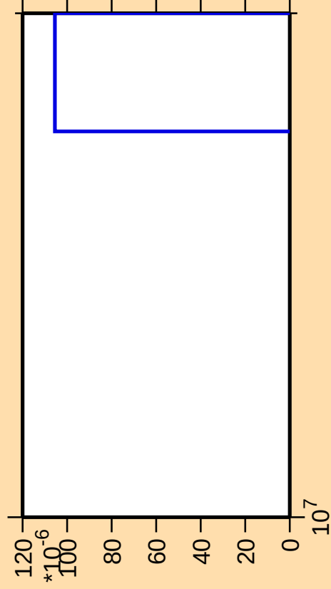
\Delta\sigma/\sigma vs. E for ^{174}\text{Er}(\text{mt 11})
