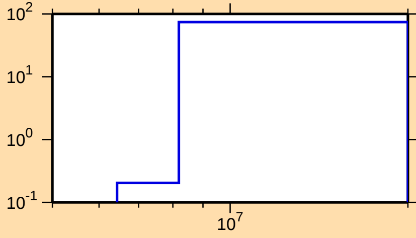
\Delta\sigma/\sigma vs. E for ^{174}\text{Er}(n,p)
