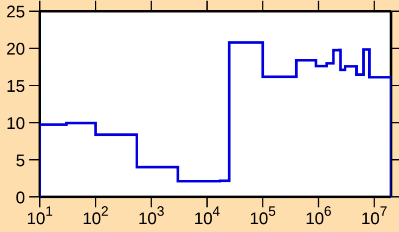
\Delta\sigma/\sigma vs. E for ^{174}\text{Er}(n,\text{tot.})
