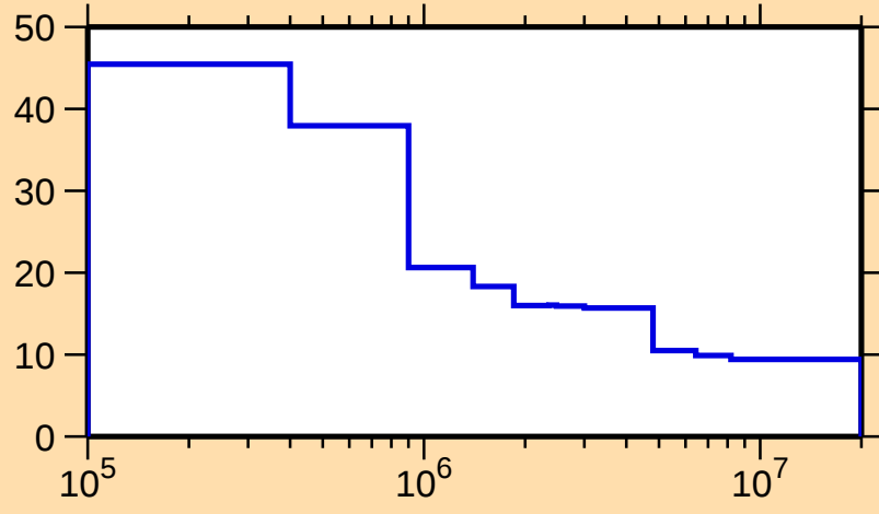
\Delta\sigma/\sigma vs. E for ^{174}\text{Er}(\text{n,nonel.})
