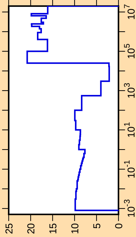
\Delta\sigma/\sigma vs. E for ^{174}\text{Er}(n,\text{tot.})
