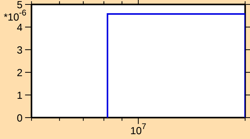
\sigma vs. E for ^{174}\text{Er}(n,np)
