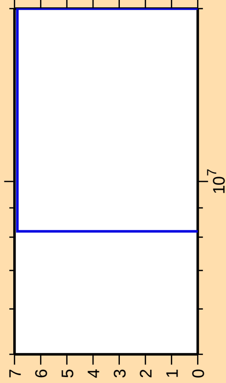
\Delta\sigma/\sigma vs. E for ^{174}\text{Er}(n,2np)
