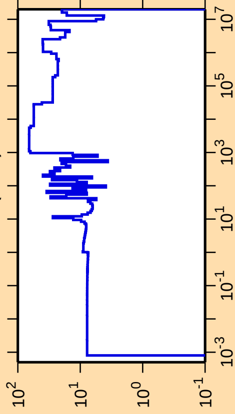
\Delta\sigma/\sigma vs. E for ^{175}\text{Er}(n,\text{el.})
