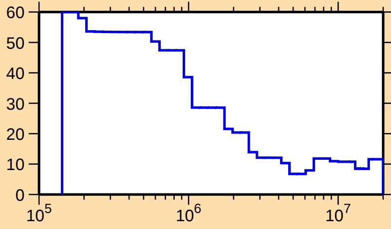
\Delta\sigma/\sigma vs. E for ^{175}\text{Er}(n,n\text{onel.})
