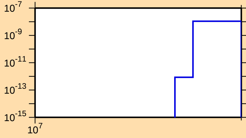
\sigma vs. E for ^{175}\text{Er}(n,2np)
