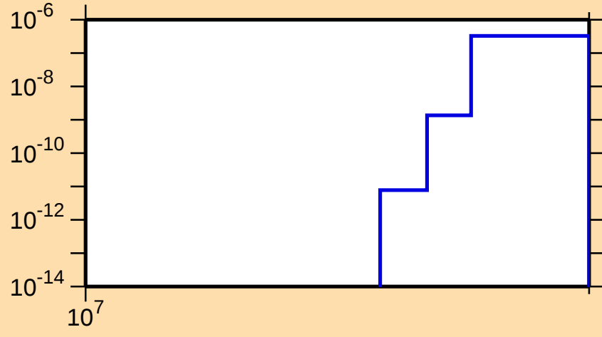
\sigma vs. E for ^{175}\text{Er}(n,nt)
