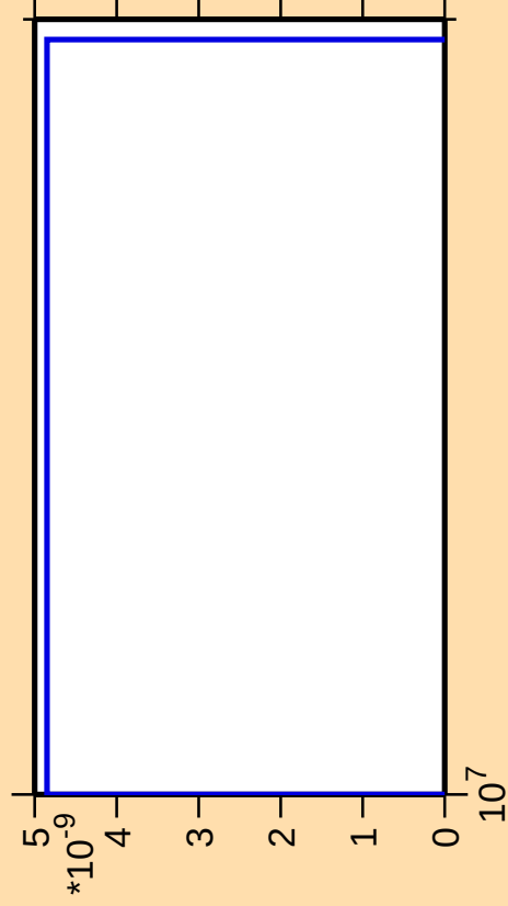
\Delta\sigma/\sigma vs. E for ^{175}\text{Er}(\text{mt 11})
