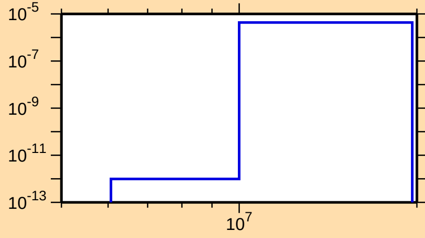
\sigma vs. E for ^{175}\text{Er}(n,n\alpha)
