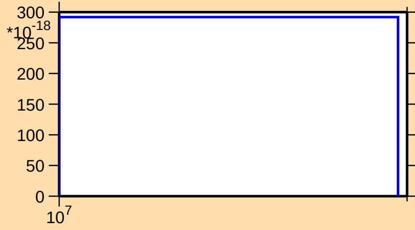
\sigma vs. E for ^{175}\text{Er}(n,3n\alpha)
