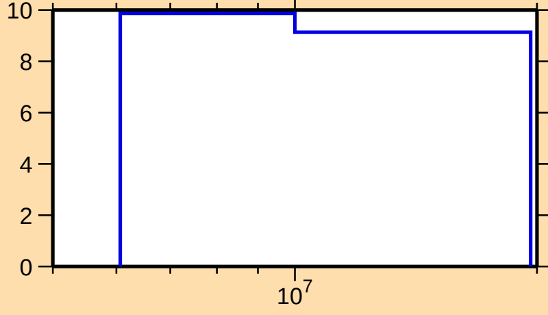
\Delta\sigma/\sigma vs. E for ^{175}\text{Er}(n,\text{nonel.})
