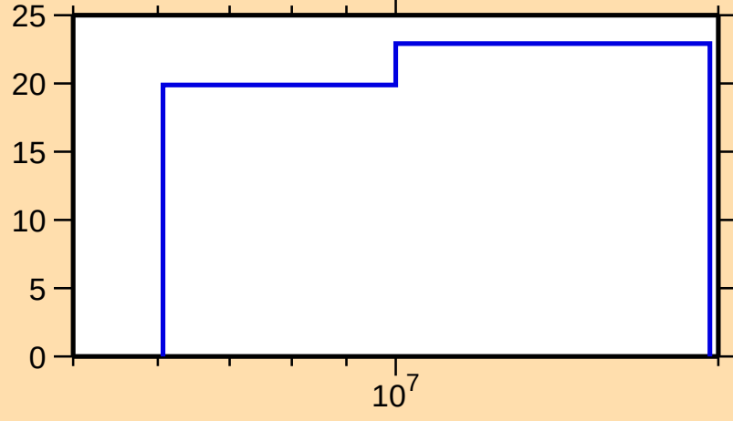
\Delta\sigma/\sigma vs. E for ^{175}\text{Er}(n,2n)
