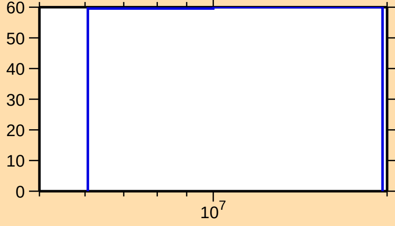
\Delta\sigma/\sigma vs. E for ^{175}\text{Er}(n,\text{ncont.})
