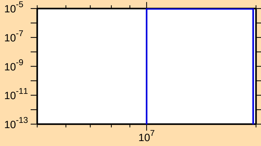
\sigma vs. E for ^{175}\text{Er}(n,t)
