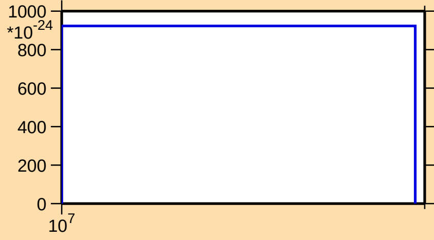
\sigma vs. E for ^{175}\text{Er}(\text{mt 11})
