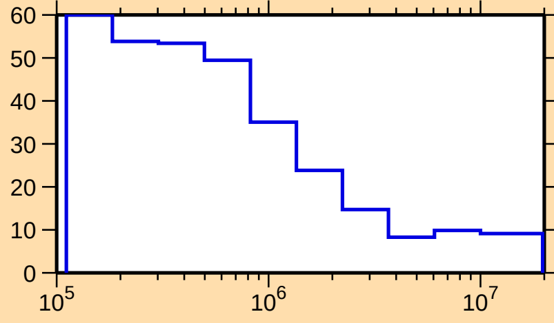
\Delta\sigma/\sigma vs. E for ^{175}\text{Er}(n,n\text{onrel.})
