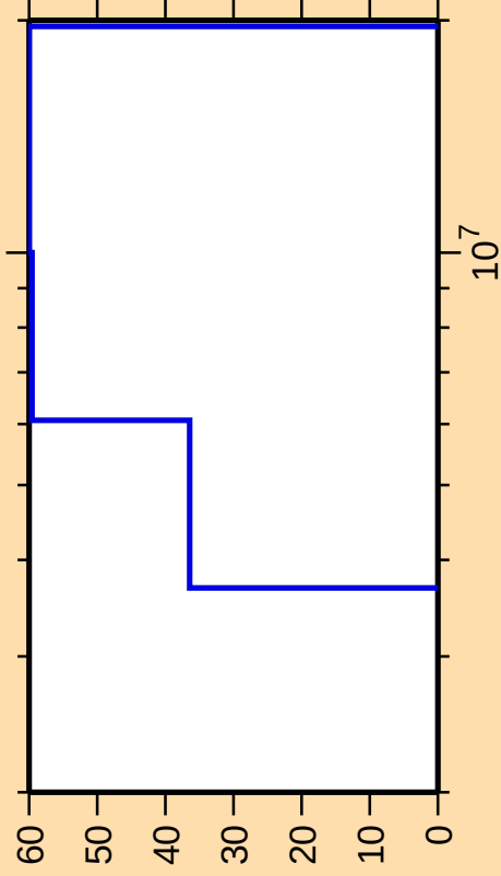
\Delta\sigma/\sigma vs. E for ^{175}\text{Er}(n,n\text{cont.})
