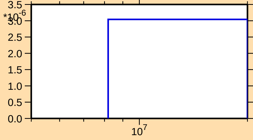
\sigma vs. E for ^{175}\text{Er}(n,np)
