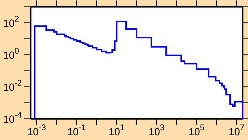
\sigma vs. E for ^{175}\text{Er}(n,\gamma)
