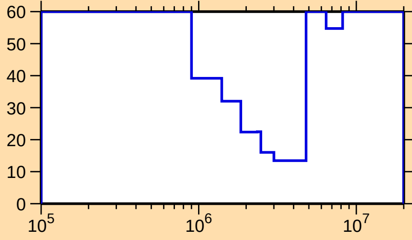
\Delta\sigma/\sigma vs. E for ^{175}\text{Er}(n,n\text{cont.})
