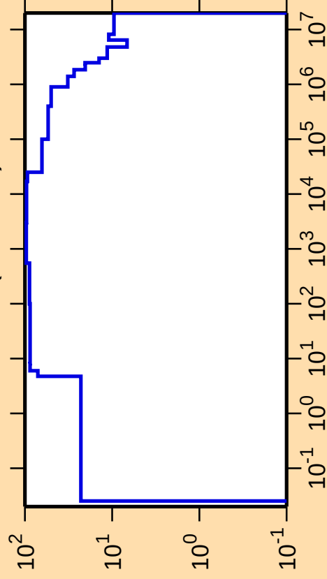
\Delta\sigma/\sigma vs. E for ^{175}\text{Er}(n,\text{nonel.})
