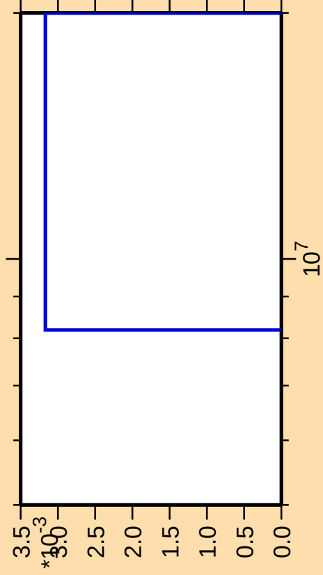
\Delta\sigma/\sigma vs. E for ^{175}\text{Er}(n,3n\alpha)
