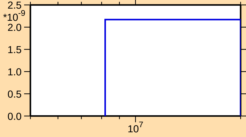
\sigma vs. E for ^{175}\text{Er}(n,\text{nd})
