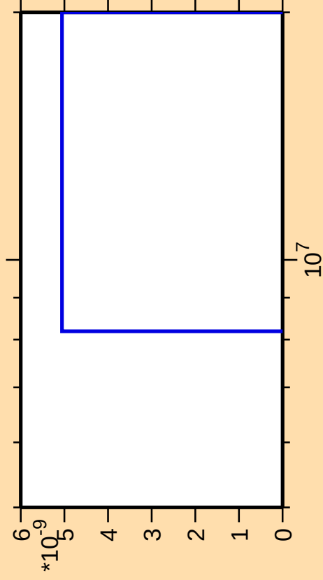
\Delta\sigma/\sigma vs. E for ^{175}\text{Er}(\text{mt 11})
