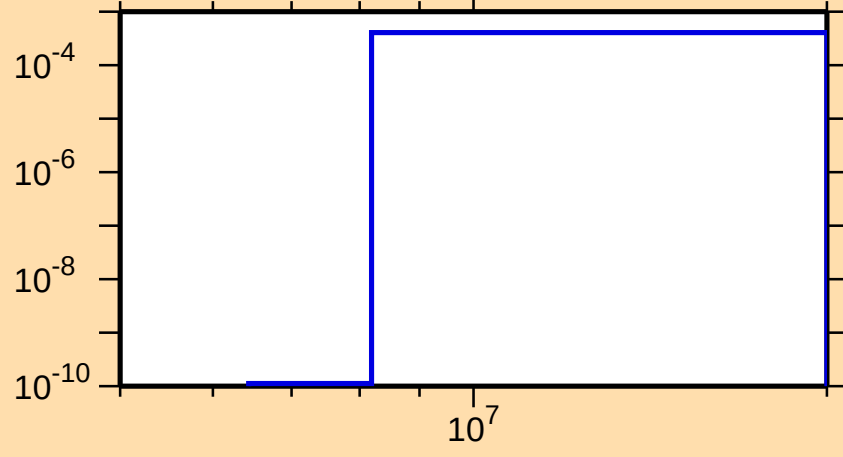
\sigma vs. E for ^{175}\text{Er}(n,p)
