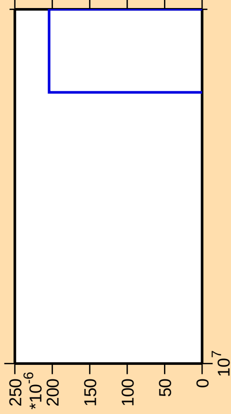
\Delta\sigma/\sigma vs. E for ^{176}\text{Er}(\text{mt 11})
