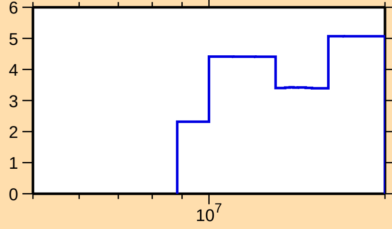
\Delta\sigma/\sigma vs. E for ^{176}\text{Er}(n,\text{tot.})
