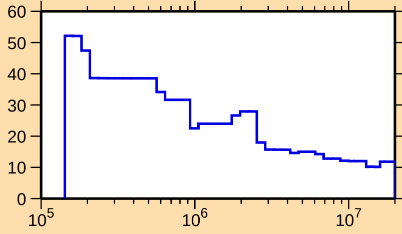
\Delta\sigma/\sigma vs. E for ^{176}\text{Er}(n,n\text{onel.})
