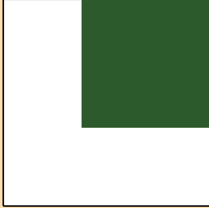
\sigma vs. E for ^{176}\text{Er}(n,2n\alpha)
