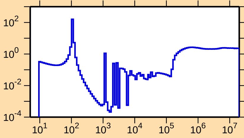
\sigma vs. E for ^{176}\text{Er}(n,\text{nonel.})
