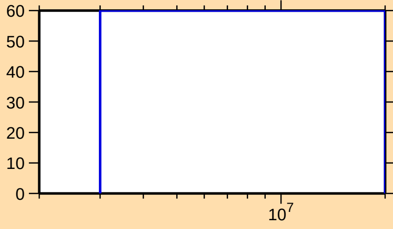
\Delta\sigma/\sigma vs. E for ^{176}\text{Er}(n,\gamma)
