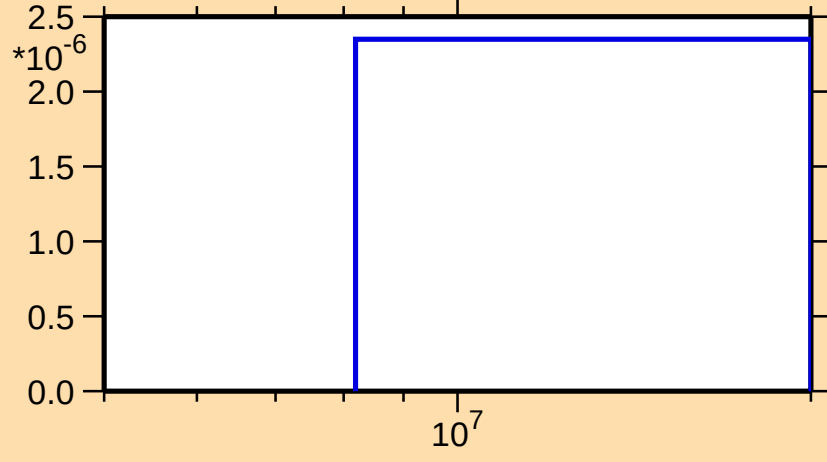
\sigma vs. E for ^{176}\text{Er}(n,d)
