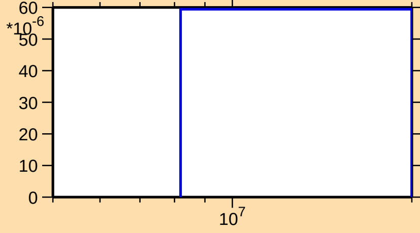
\sigma vs. E for ^{176}\text{Er}(n,p)
