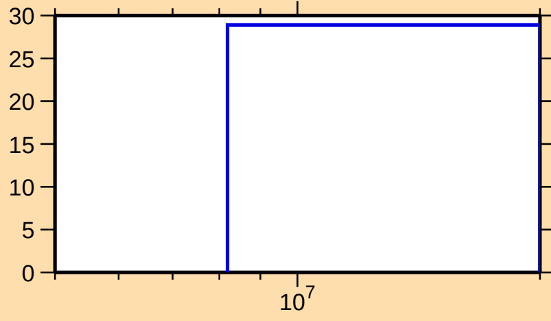
\Delta\sigma/\sigma vs. E for ^{176}\text{Er}(n,\text{ncont.})
