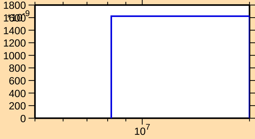
\sigma vs. E for ^{176}\text{Er}(n,n\alpha)
