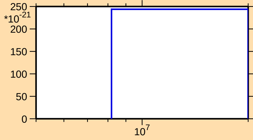
\sigma vs. E for ^{176}\text{Er}(\text{mt } 11)
