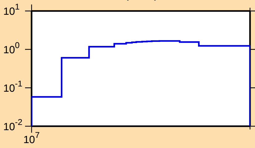
\sigma vs. E for ^{177}\text{Er}(n,3n)
