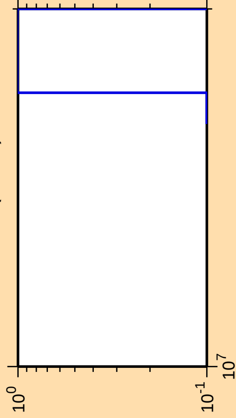
\Delta\sigma/\sigma vs. E for ^{177}\text{Er}(n,3n\alpha)
