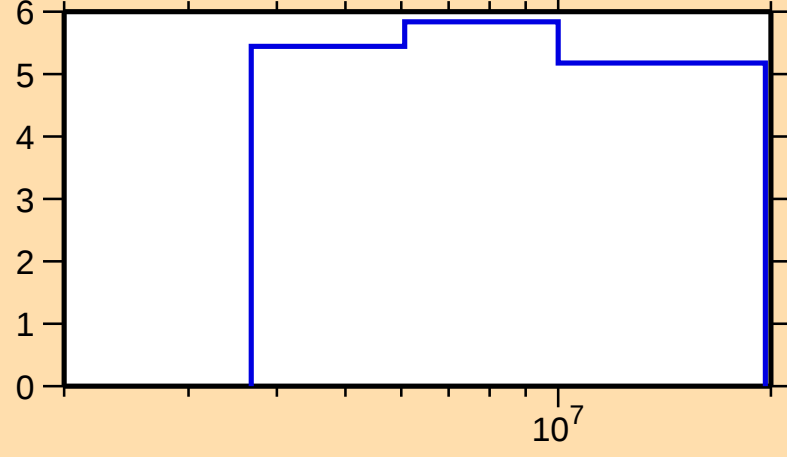
\Delta\sigma/\sigma vs. E for ^{177}\text{Er}(n,\text{nonel.})
