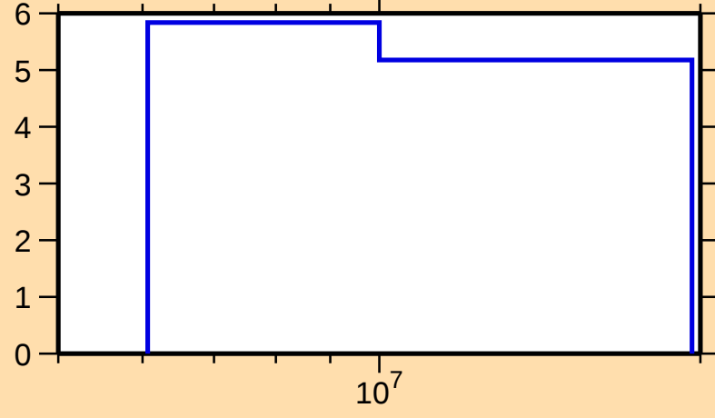
\Delta\sigma/\sigma vs. E for ^{177}\text{Er}(n,\text{nonel.})
