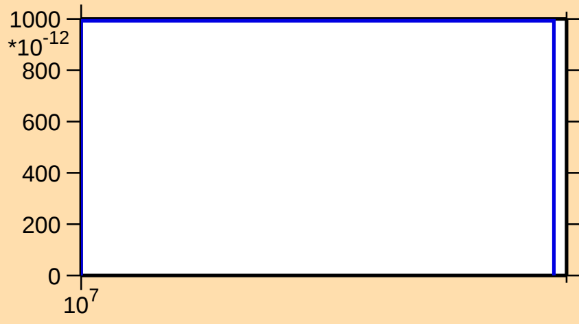
\sigma vs. E for ^{177}\text{Er}(n,\text{nd})
