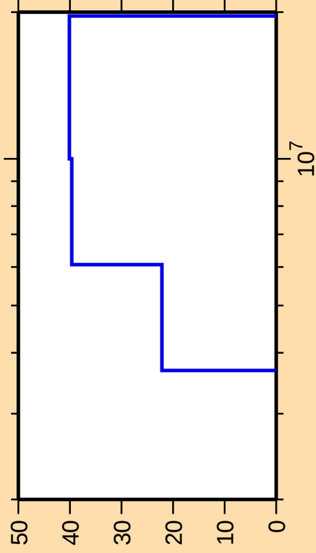
\Delta\sigma/\sigma vs. E for ^{177}\text{Er}(n,n\text{cont.})
