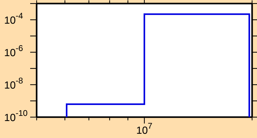
\sigma vs. E for ^{177}\text{Er}(n,p)
