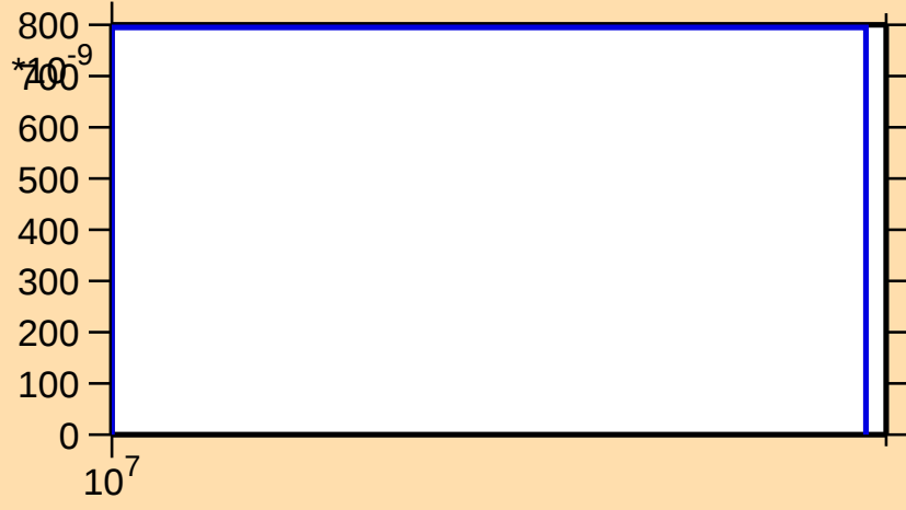
\sigma vs. E for ^{177}\text{Er}(n,np)
