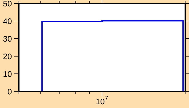
\Delta\sigma/\sigma vs. E for ^{177}\text{Er}(n,\text{ncont.})
