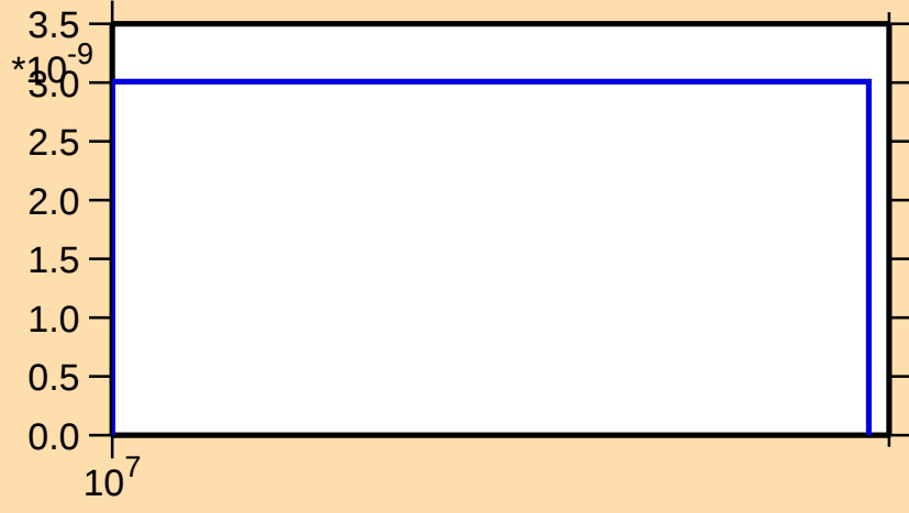
\sigma vs. E for ^{177}\text{Er}(n,\text{nt})
