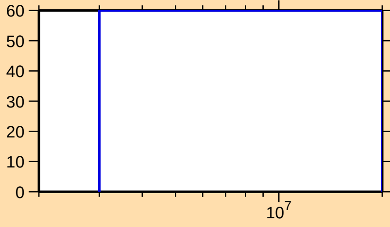
\Delta\sigma/\sigma vs. E for ^{177}\text{Er}(n,\gamma)
