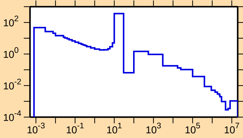
\sigma vs. E for ^{177}\text{Er}(n,\gamma)
