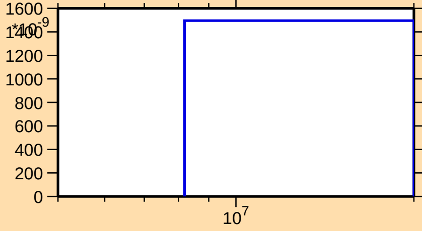
\sigma vs. E for ^{177}\text{Er}(n,n\alpha)
