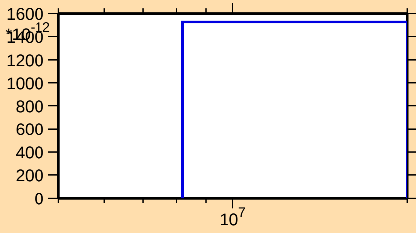
\sigma vs. E for ^{177}\text{Er}(n,2n\alpha)
