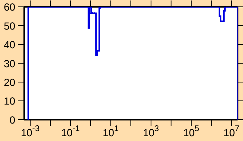
\Delta\sigma/\sigma vs. E for ^{239}\text{Es}(n,\gamma)
