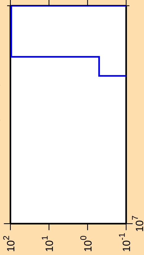
\Delta\sigma/\sigma vs. E for ^{239}\text{Es}(n,3n\alpha)
