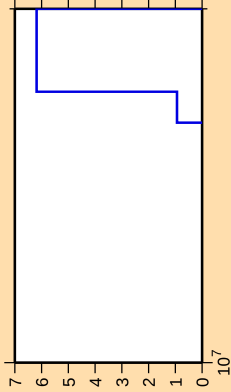
\Delta\sigma/\sigma vs. E for ^{239}\text{Es}(n,\text{pd})
