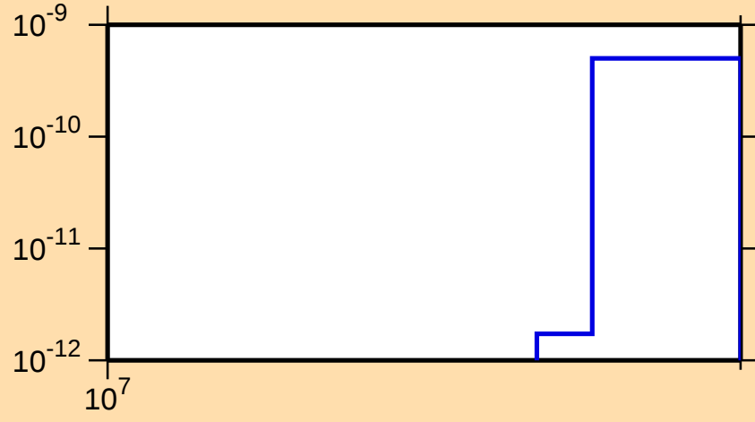
\sigma vs. E for ^{239}\text{Es}(n,3n)
