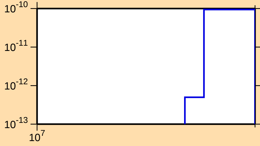
\sigma vs. E for ^{239}\text{Es}(n,3n\alpha)
