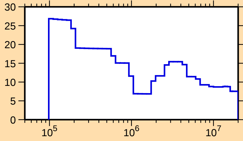
\Delta\sigma/\sigma vs. E for ^{239}\text{Es}(n,f)
