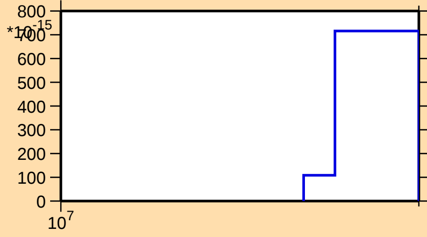
\sigma vs. E for ^{239}\text{Es}(n,\text{pd})
