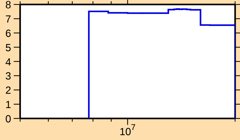
\Delta\sigma/\sigma vs. E for ^{239}\text{Es}(n,\text{nonel.})
