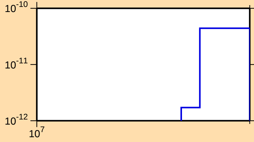
\sigma vs. E for ^{239}\text{Es}(n,nt)
