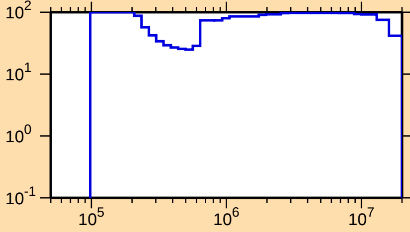
\Delta\sigma/\sigma vs. E for ^{239}\text{Es}(n,n\text{cont.})
