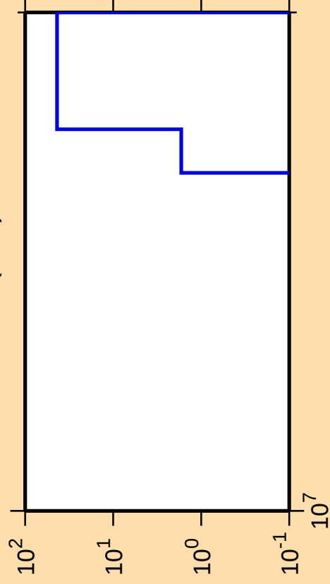
\Delta\sigma/\sigma vs. E for ^{239}\text{Es}(n,nt)
