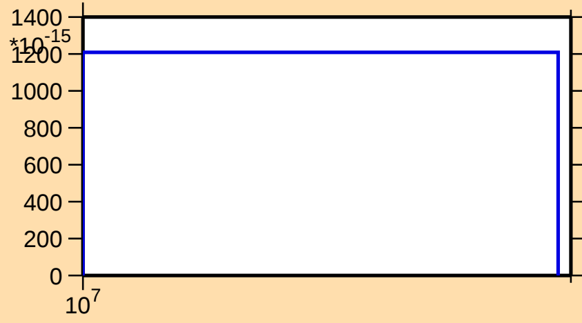
\sigma vs. E for ^{239}\text{Es}(n,3n\alpha)
