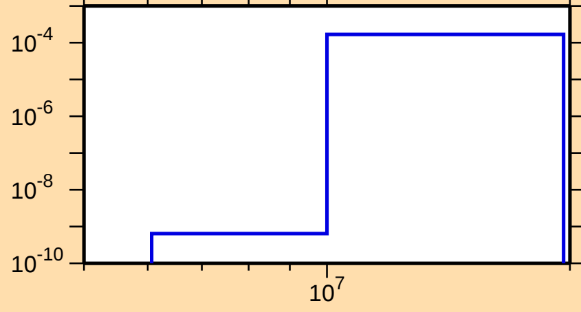
\sigma vs. E for ^{239}\text{Es}(n,t)
