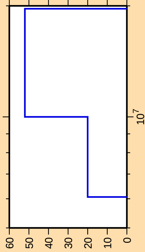
\Delta\sigma/\sigma vs. E for ^{239}\text{Es}(n,t)
