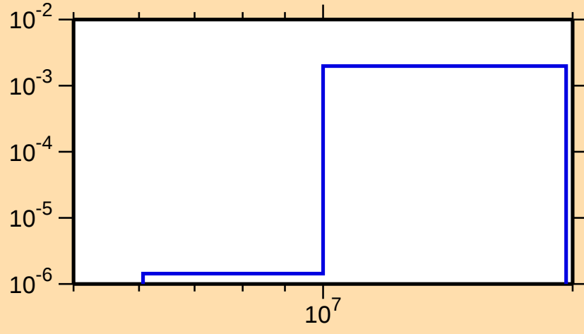
\sigma vs. E for ^{239}\text{Es}(n,2n)
