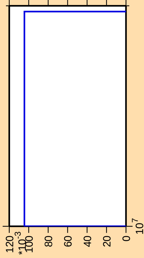
\Delta\sigma/\sigma vs. E for ^{239}\text{Es}(n,\text{pd})
