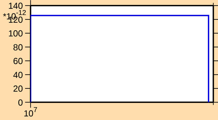
\sigma vs. E for ^{239}\text{Es}(n,\text{nd})
