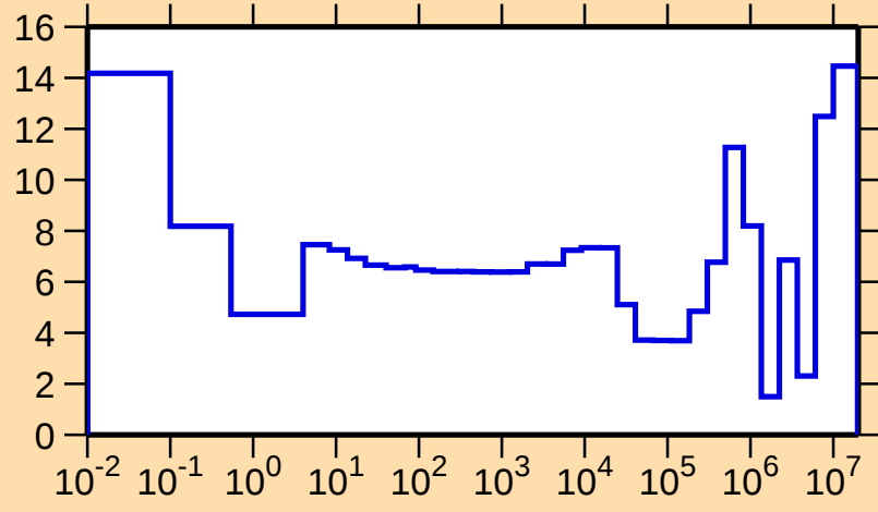
\Delta\sigma/\sigma vs. E for ^{239}\text{Es}(n,\text{el.})
