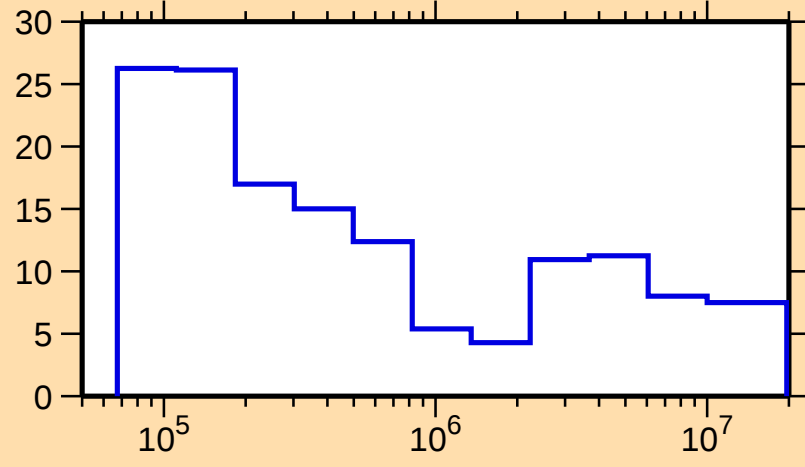
\Delta\sigma/\sigma vs. E for ^{239}\text{Es}(n,\text{nonel.})
