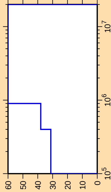
\Delta\sigma/\sigma vs. E for ^{239}\text{Es}(\text{n},\text{ncont.})
