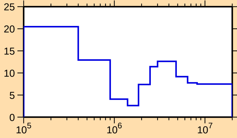
\Delta\sigma/\sigma vs. E for ^{239}\text{Es}(n,\text{nonel.})
