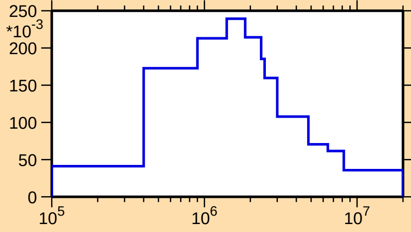
\sigma vs. E for ^{239}\text{Es}(n,n_1)
