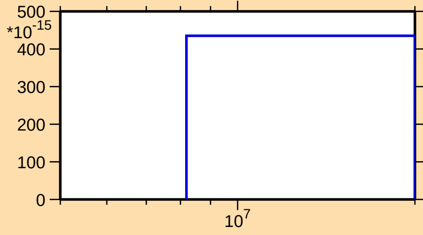
\sigma vs. E for ^{239}\text{Es}(n,nt)
