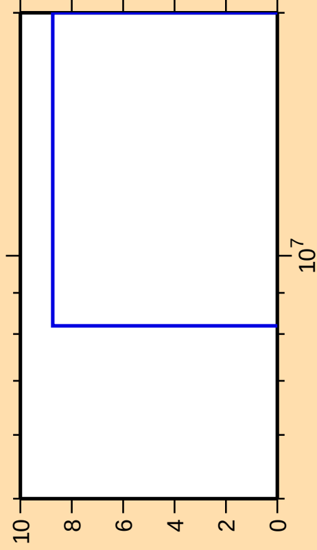
\Delta\sigma/\sigma vs. E for ^{239}\text{Es}(n,f)
