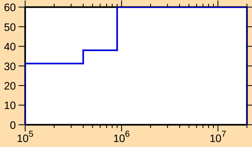
\Delta\sigma/\sigma vs. E for ^{239}\text{Es}(n,n\text{cont.})
