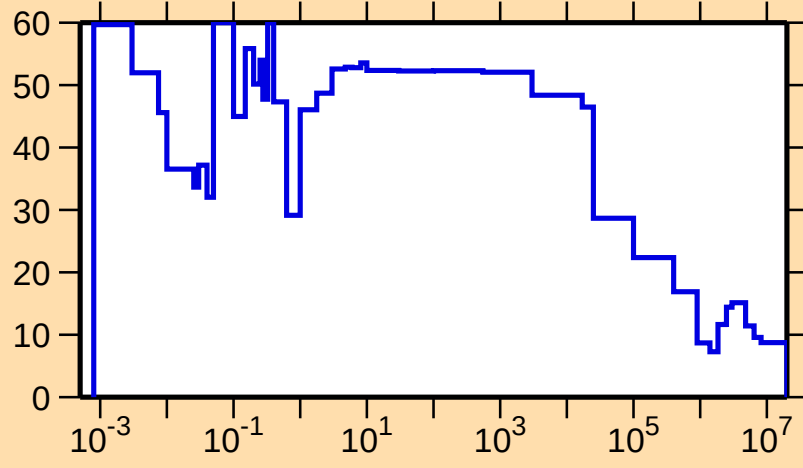
\Delta\sigma/\sigma vs. E for ^{239}\text{Es}(n,f)
