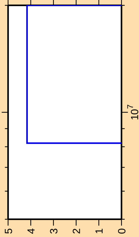
\Delta\sigma/\sigma vs. E for ^{239}\text{Es}(n,3n)
