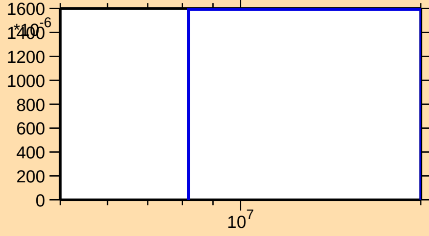
\sigma vs. E for ^{239}\text{Es}(n,2n)
