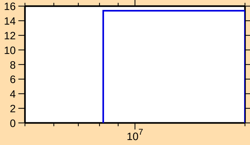
\Delta\sigma/\sigma vs. E for ^{239}\text{Es}(n,\text{el.})
