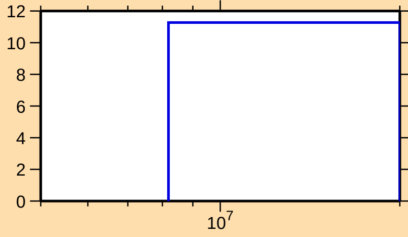
\Delta\sigma/\sigma vs. E for ^{239}\text{Es}(n,\text{tot.})
