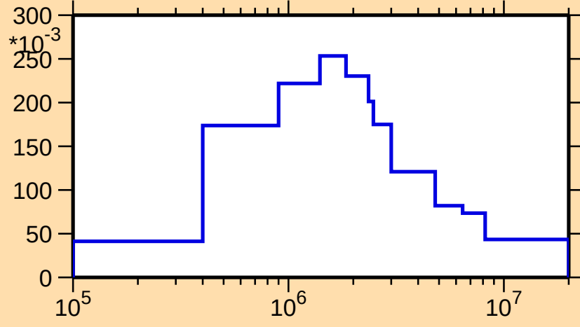
\sigma vs. E for ^{239}\text{Es}(n,\text{inel.})
