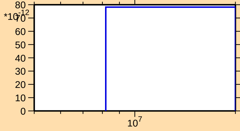
\sigma vs. E for ^{239}\text{Es}(n,2np)
