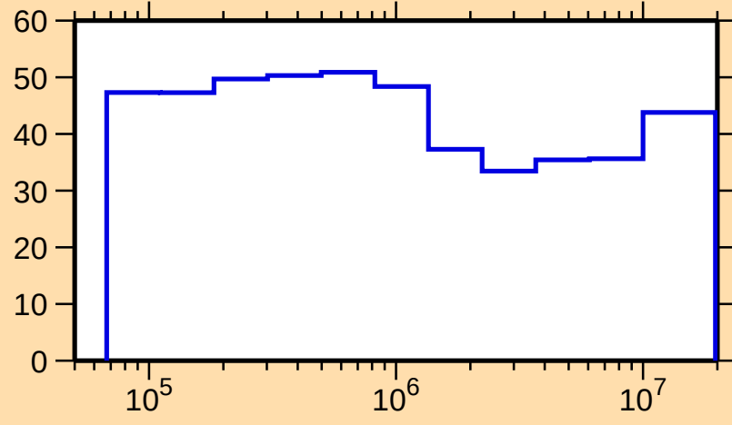
\Delta\sigma/\sigma vs. E for ^{241}\text{Es}(n,n\text{onel.})
