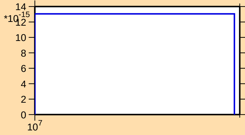
\sigma vs. E for ^{241}\text{Es}(\text{mt } 34)
