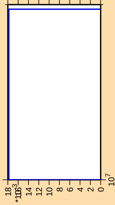
\Delta\sigma/\sigma vs. E for ^{241}\text{Es}(\text{mt } 34)
