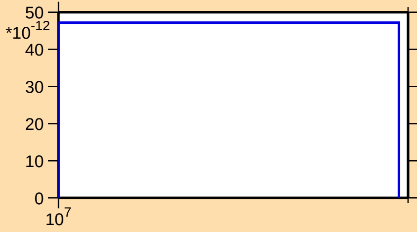
\sigma vs. E for ^{241}\text{Es}(n,nt)
