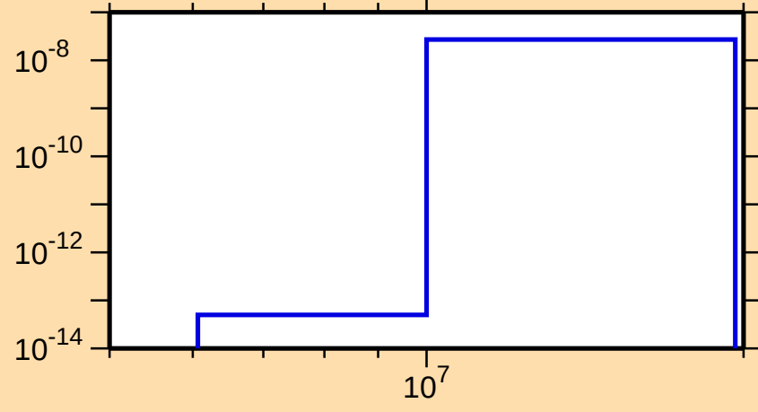
\sigma vs. E for ^{241}\text{Es}(n,\text{He3})
