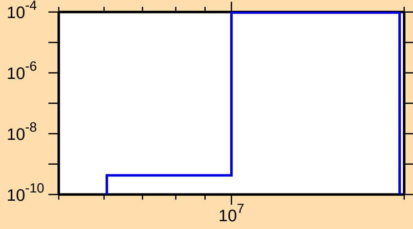
\sigma vs. E for ^{241}\text{Es}(n,t)
