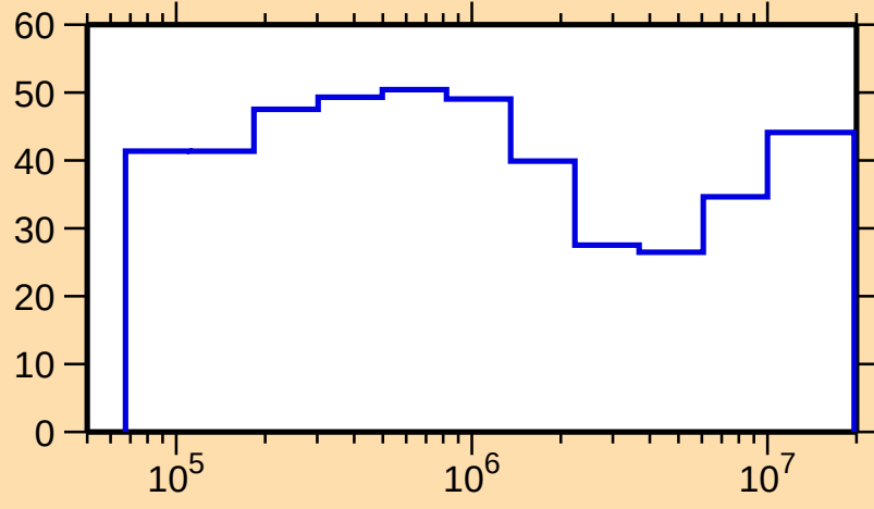
\Delta\sigma/\sigma vs. E for ^{241}\text{Es}(n,f)
