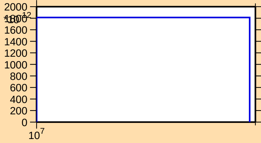
\sigma vs. E for ^{241}\text{Es}(n,\text{nd})
