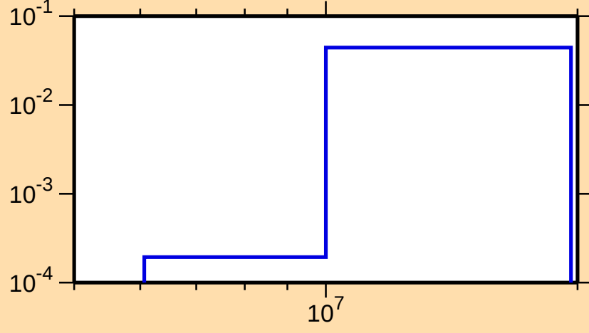
\sigma vs. E for ^{241}\text{Es}(n,2n)
