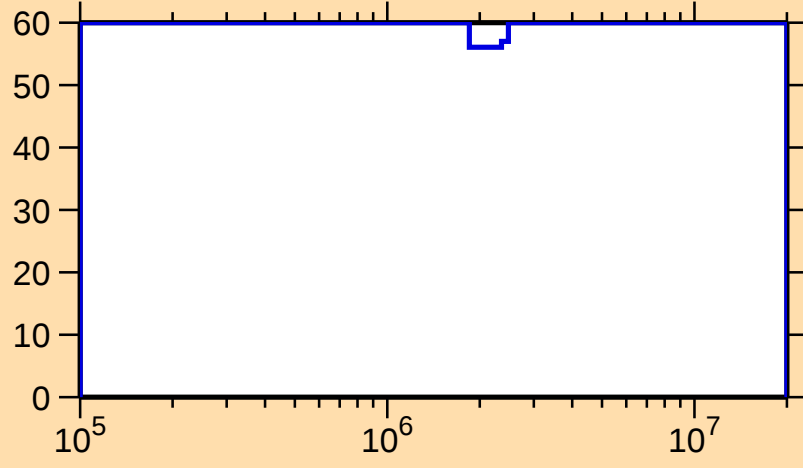
\Delta\sigma/\sigma vs. E for ^{241}\text{Es}(\text{n,el.})
