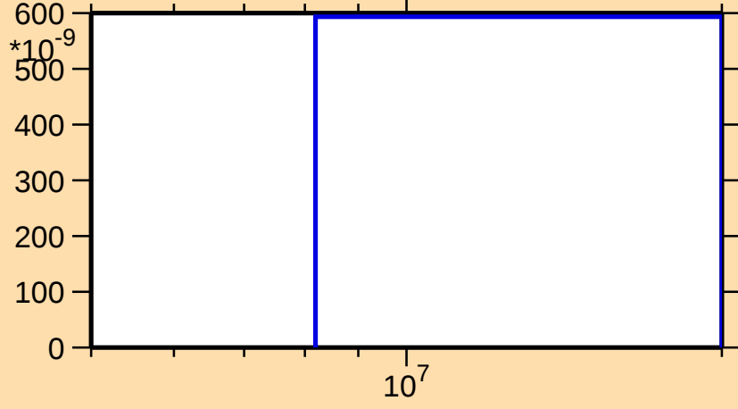
\sigma vs. E for ^{241}\text{Es}(n,3n)
