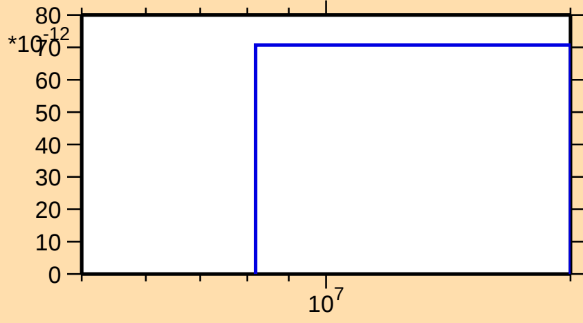
\sigma vs. E for ^{241}\text{Es}(\text{mt117})
