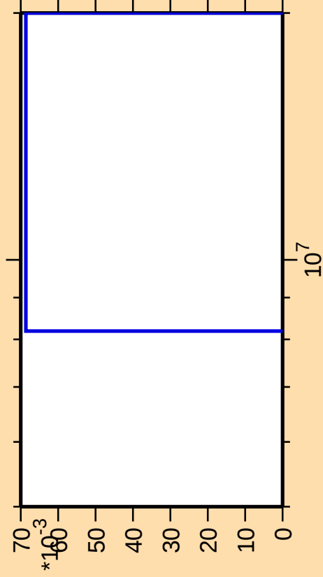
\Delta\sigma/\sigma vs. E for ^{241}\text{Es}(n,\text{pd})
