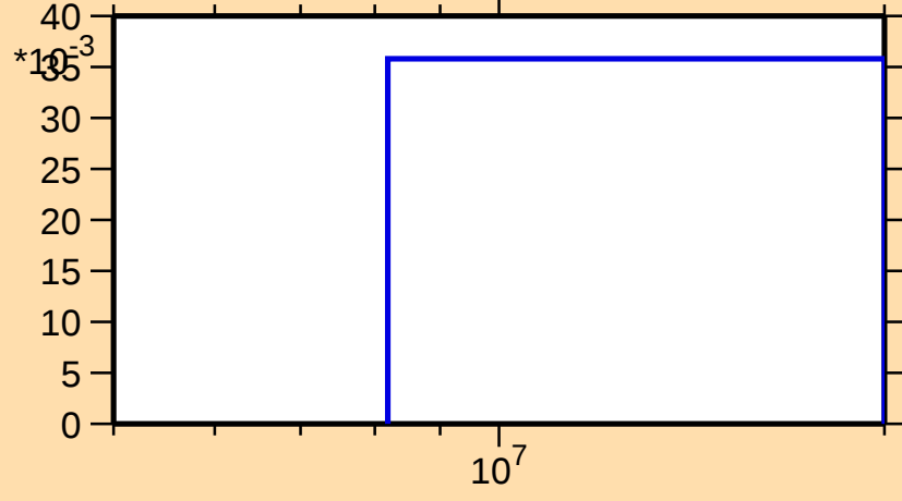
\sigma vs. E for ^{241}\text{Es}(n,2n)
