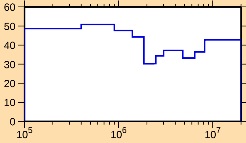
\Delta\sigma/\sigma vs. E for ^{241}\text{Es}(n,\text{nonel.})
