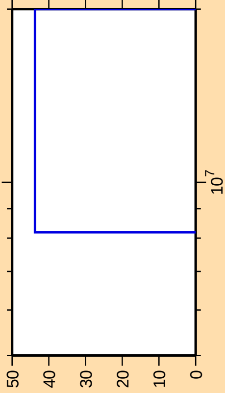
\Delta\sigma/\sigma vs. E for ^{241}\text{Es}(n,f)
