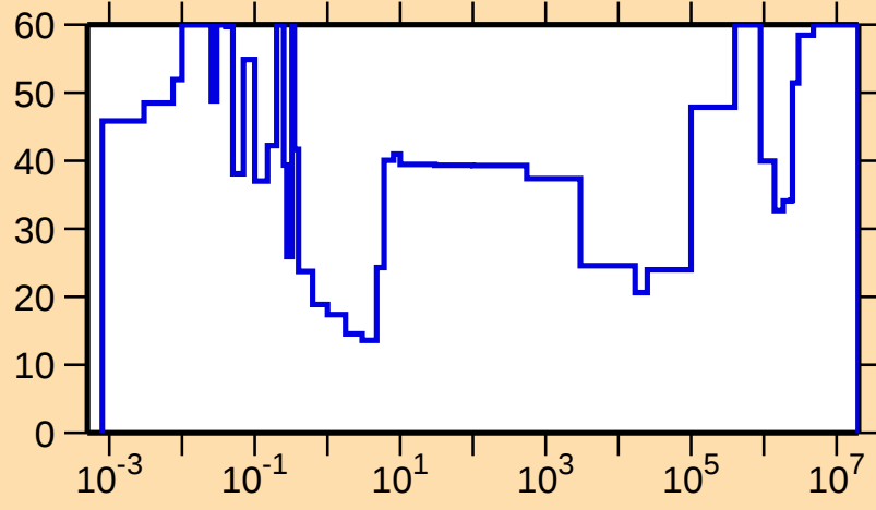
\Delta\sigma/\sigma vs. E for ^{241}\text{Es}(n,\text{tot.})
