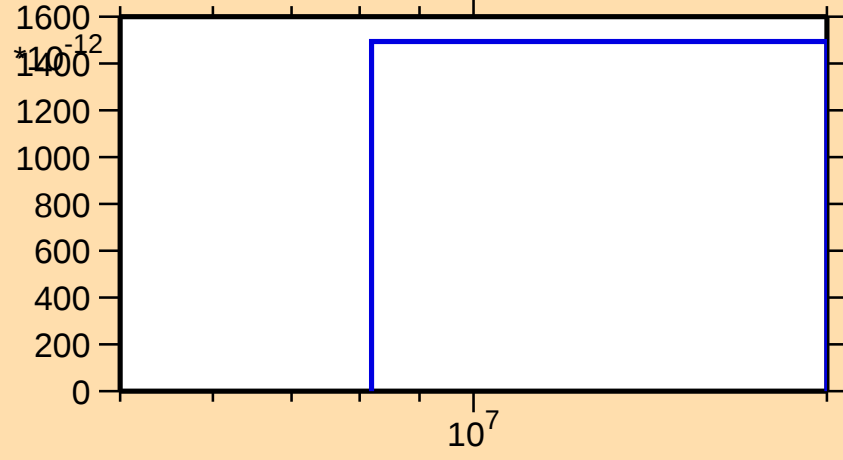
\sigma vs. E for ^{241}\text{Es}(n,nd)
