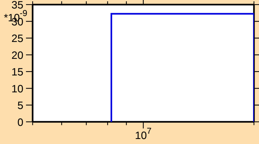
\sigma vs. E for ^{241}\text{Es}(n,3n\alpha)
