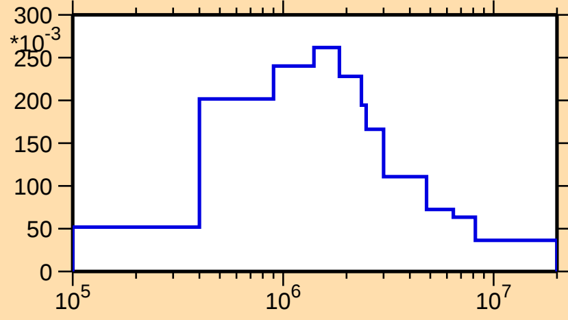
\sigma vs. E for ^{241}\text{Es}(n,n_1)
