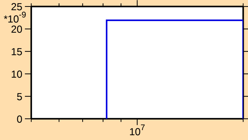
\sigma vs. E for ^{241}\text{Es}(n,\text{He}3)
