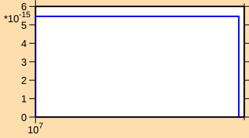
\sigma vs. E for ^{251}\text{Es}(\text{mt } 11)
