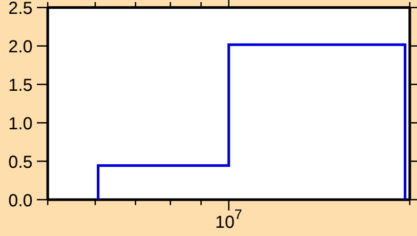
\sigma vs. E for ^{251}\text{Es}(n,2n)
