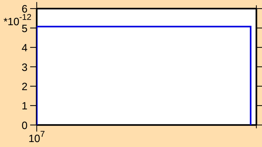
\sigma vs. E for ^{251}\text{Es}(n,\text{He}3)
