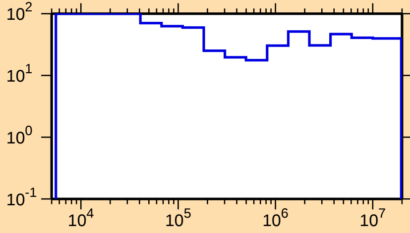
\Delta\sigma/\sigma vs. E for ^{251}\text{Es}(n,n_1)
