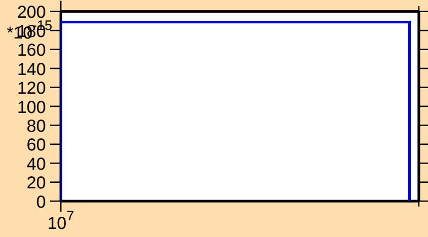
\sigma vs. E for ^{251}\text{Es}(n,3n\alpha)
