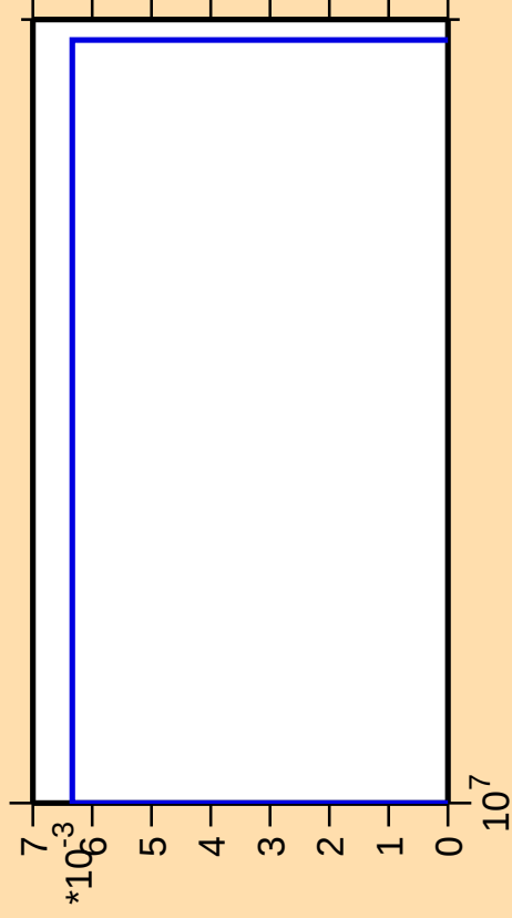
\Delta\sigma/\sigma vs. E for ^{251}\text{Es}(\text{mt } 11)
