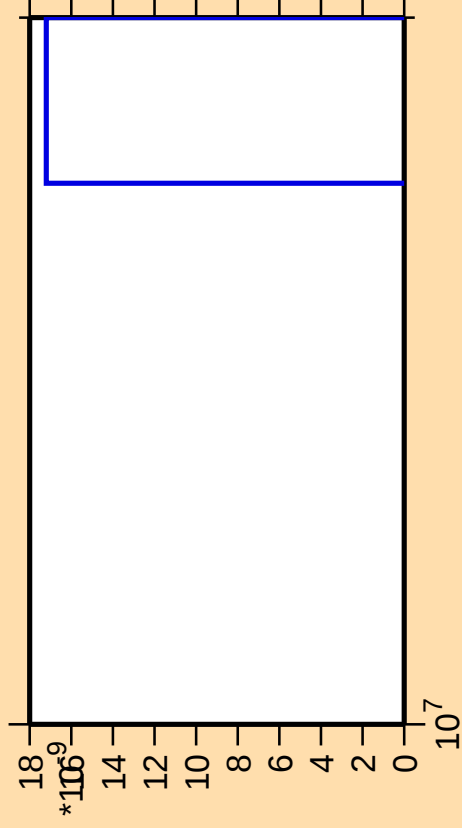
\Delta\sigma/\sigma vs. E for ^{142}\text{Eu} (mt 11)
