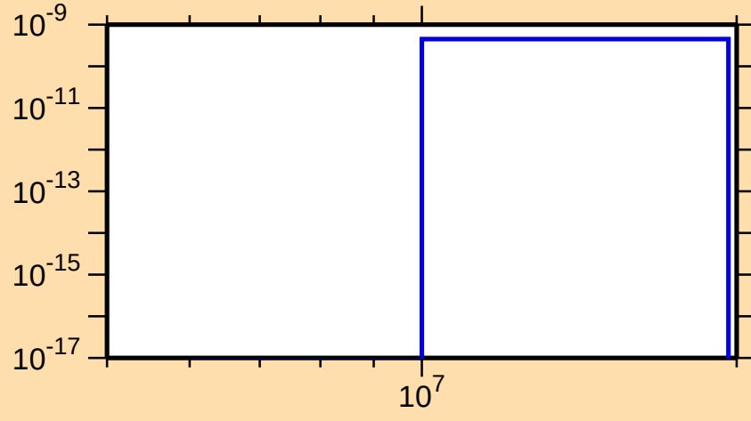
\sigma vs. E for ^{142}\text{Eu}(\text{mt117})
