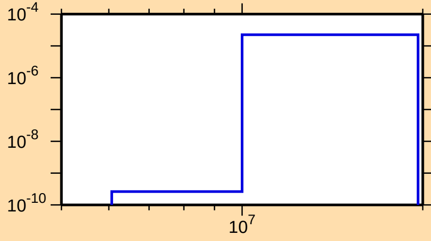
\sigma vs. E for ^{142}\text{Eu}(n,\text{He3})
