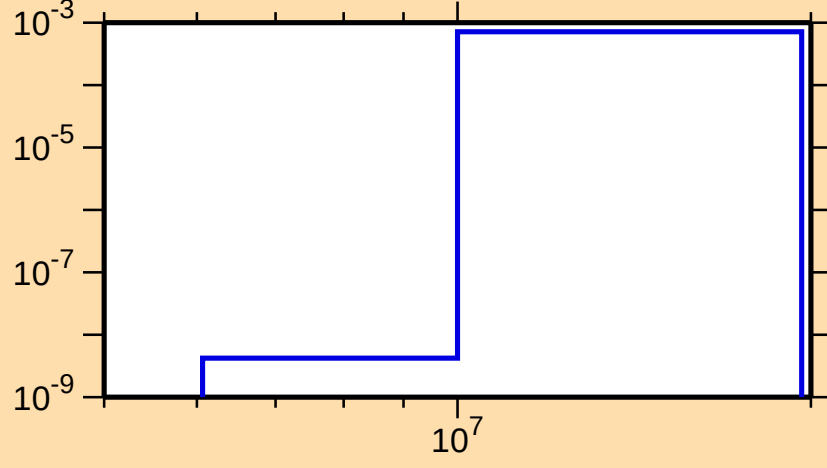
\sigma vs. E for ^{142}\text{Eu}(n,t)
