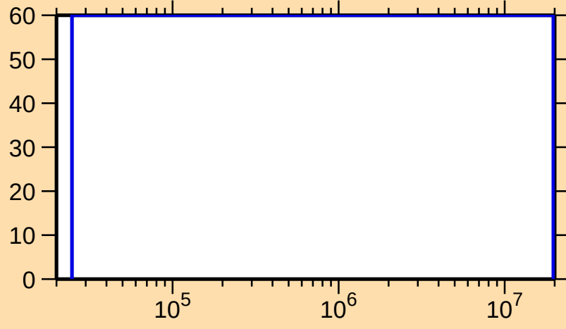
\Delta\sigma/\sigma vs. E for ^{142}\text{Eu}(n, n_1)
