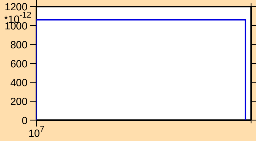
\sigma vs. E for ^{142}\text{Eu}(n,\text{pt})
