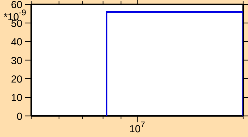
\sigma vs. E for ^{142}\text{Eu}(n,\text{pd})
