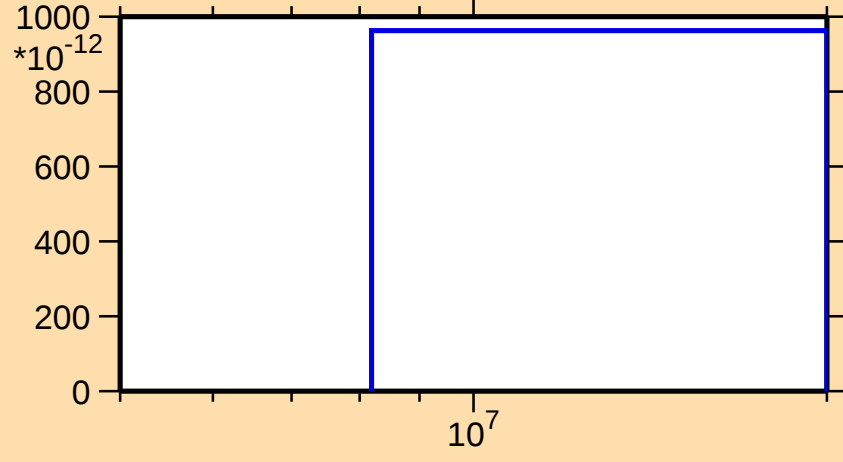
\sigma vs. E for ^{142}\text{Eu}(n,pt)
