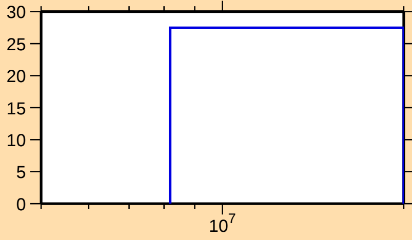
\Delta\sigma/\sigma vs. E for ^{142}\text{Eu}(n,\text{nonel.})
