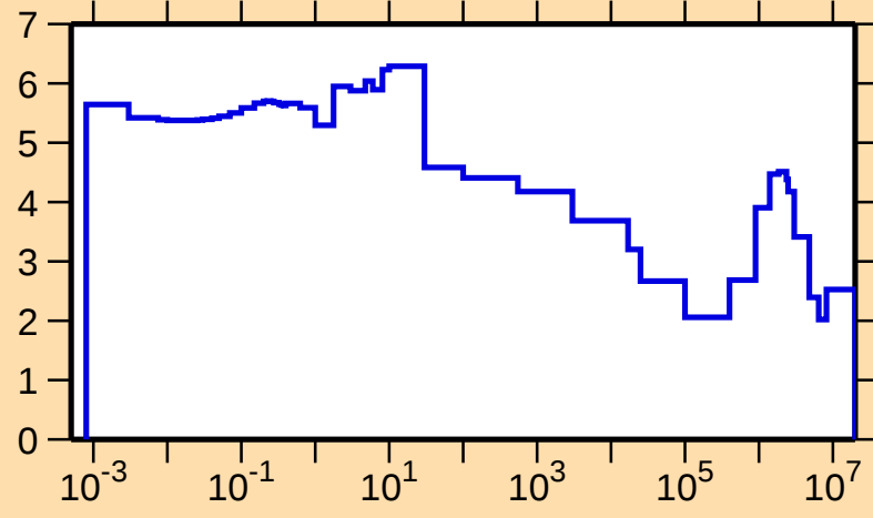
\sigma vs. E for ^{142}\text{Eu}(n,\text{el.})
