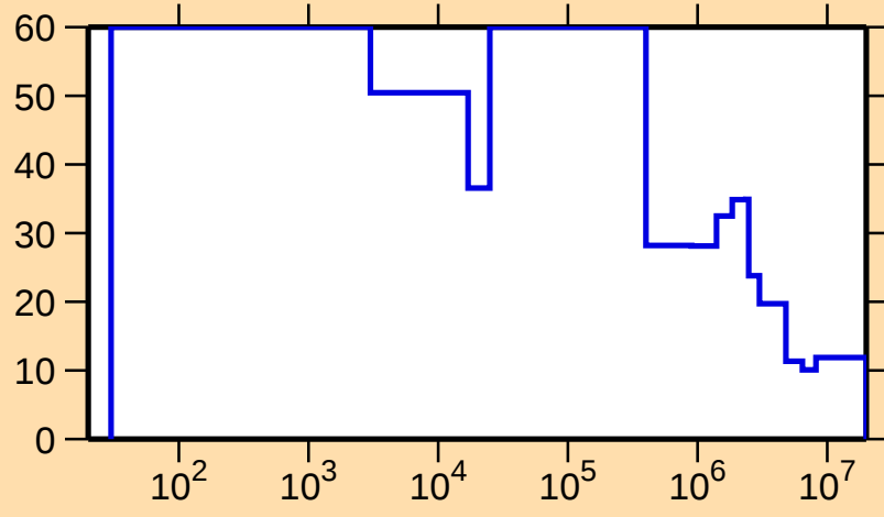
\Delta\sigma/\sigma vs. E for ^{142}\text{Eu}(n,\text{tot.})
