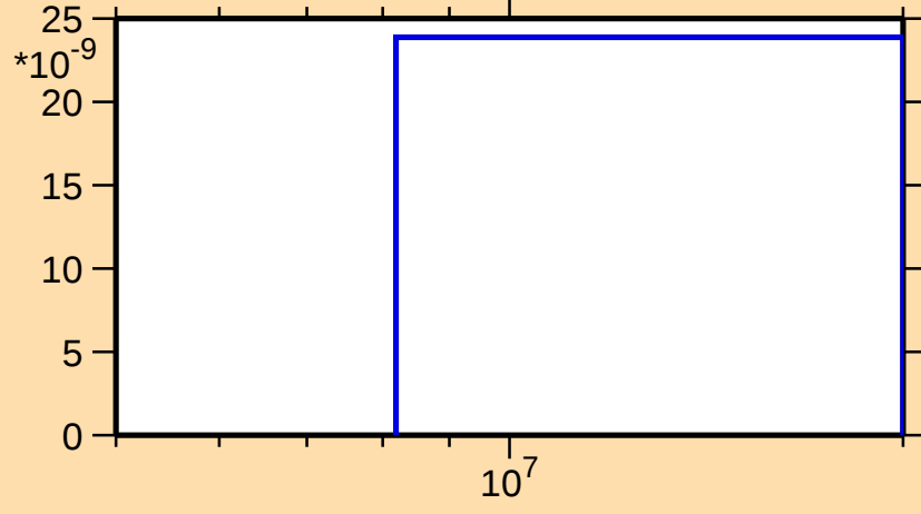
\sigma vs. E for ^{142}\text{Eu}(n,2n\alpha)
