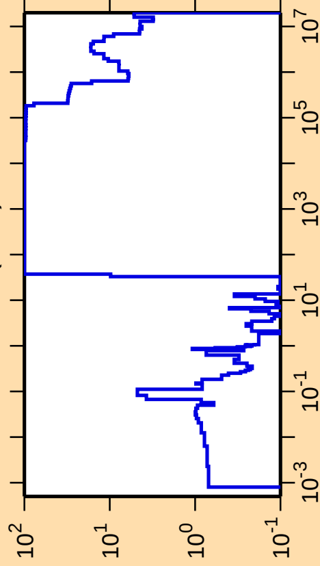
\Delta\sigma/\sigma vs. E for ^{143}\text{Eu}(n,\text{el.})
