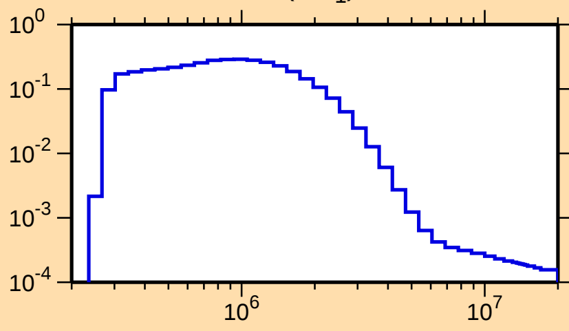
\sigma vs. E for ^{143}\text{Eu}(n,n_1)
