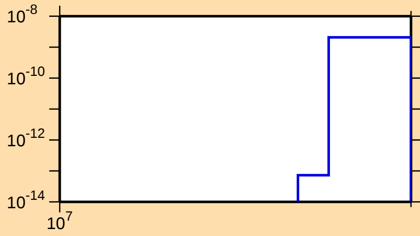
\sigma vs. E for ^{143}\text{Eu}(n,nt)
