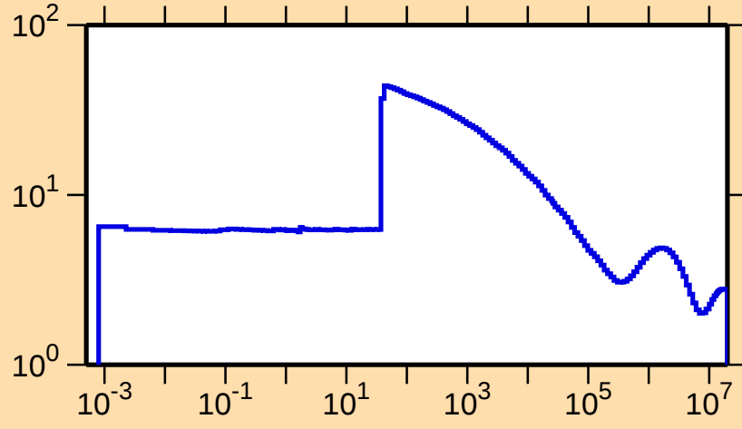
\sigma vs. E for ^{143}\text{Eu}(n,\text{el.})
