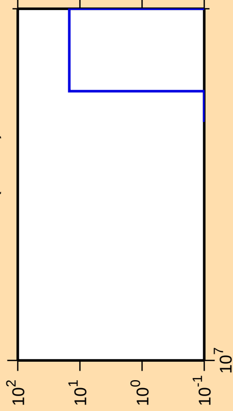
\Delta\sigma/\sigma vs. E for ^{143}\text{Eu} (mt 34)
