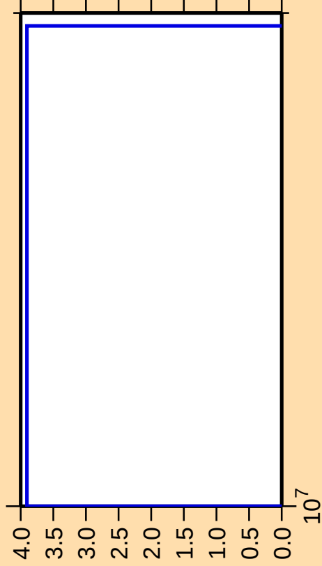
\Delta\sigma/\sigma vs. E for ^{143}\text{Eu}(n,\text{pt})
