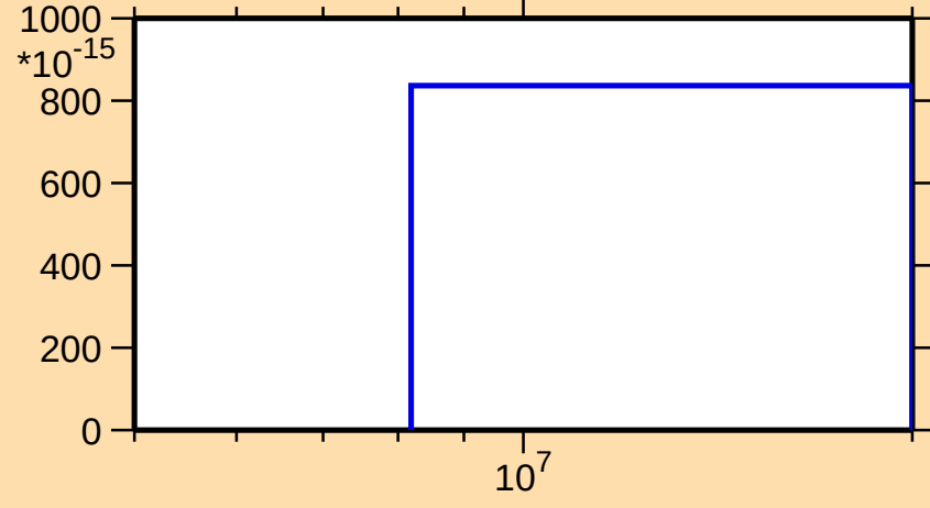
\sigma vs. E for ^{143}\text{Eu}(n,pt)
