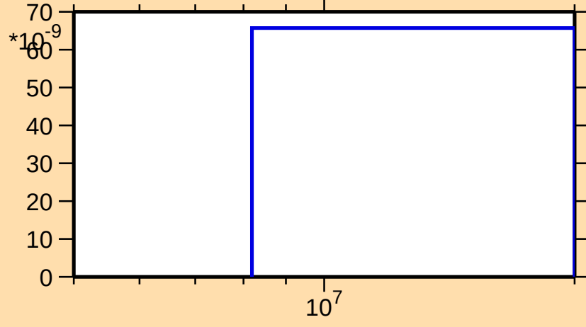
\sigma vs. E for ^{143}\text{Eu}(n,nd)
