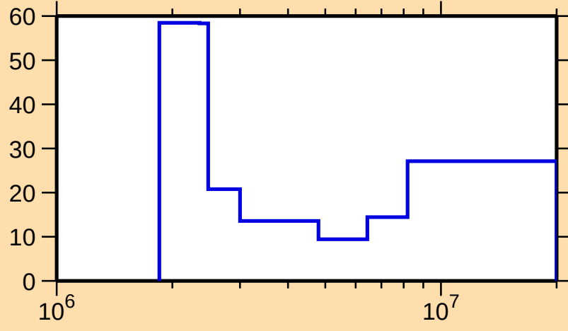
\Delta\sigma/\sigma vs. E for ^{143}\text{Eu}(n,n\text{cont.})
