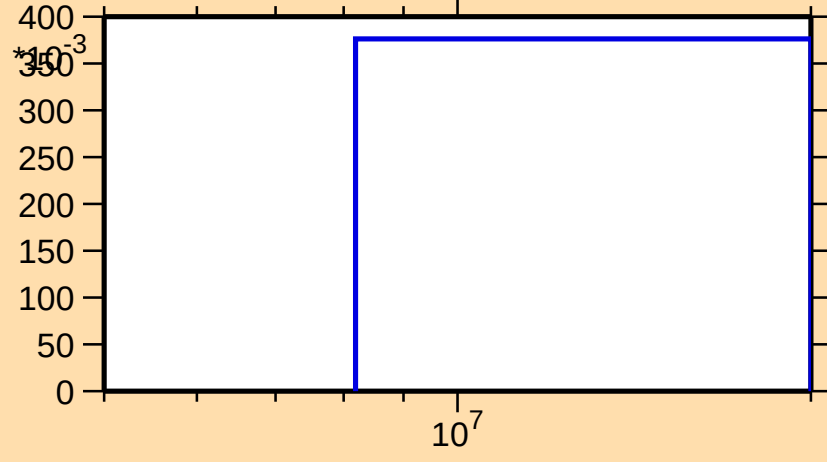
\sigma vs. E for ^{143}\text{Eu}(n,2n)
