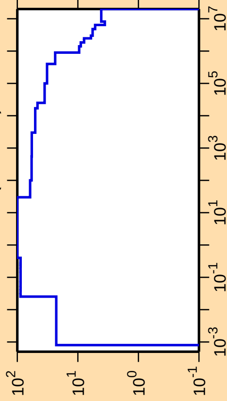
\Delta\sigma/\sigma vs. E for ^{143}\text{Eu}(n,\text{nonel.})
