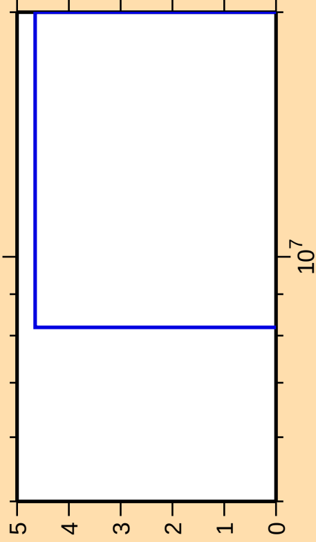
\Delta\sigma/\sigma vs. E for ^{143}\text{Eu}(n,pt)
