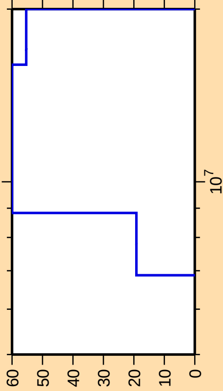
\Delta\sigma/\sigma vs. E for ^{146}\text{Eu}(n,n\text{cont.})
