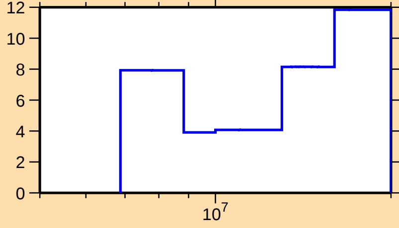
\Delta\sigma/\sigma vs. E for ^{146}\text{Eu}(n,\text{tot.})
