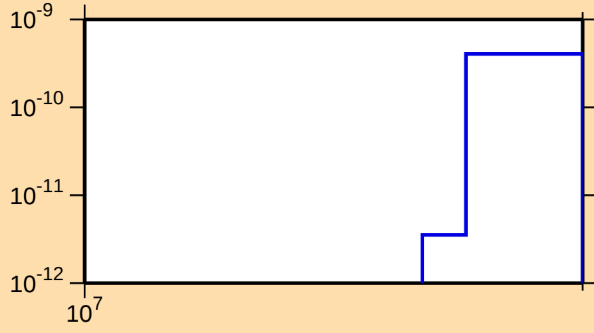
\sigma vs. E for ^{146}\text{Eu} (mt 34)
