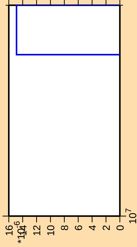
\Delta\sigma/\sigma vs. E for ^{146}\text{Eu} (mt 11)
