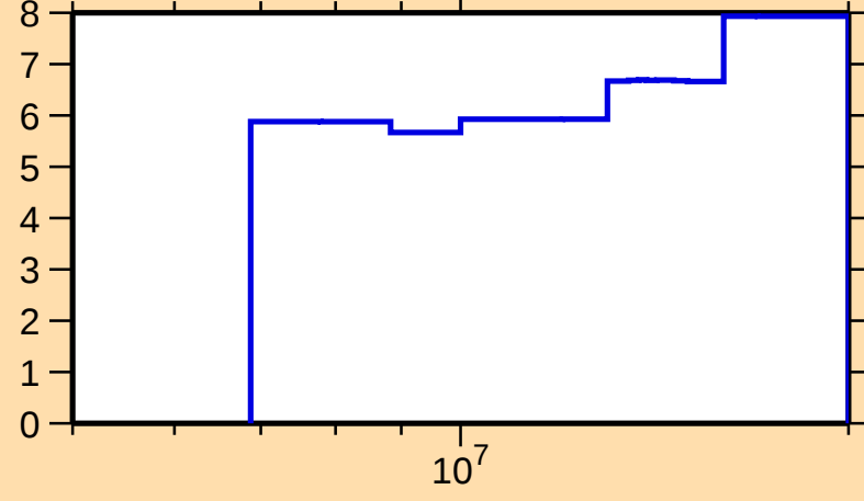
\Delta\sigma/\sigma vs. E for ^{146}\text{Eu}(n,\text{nonel.})
