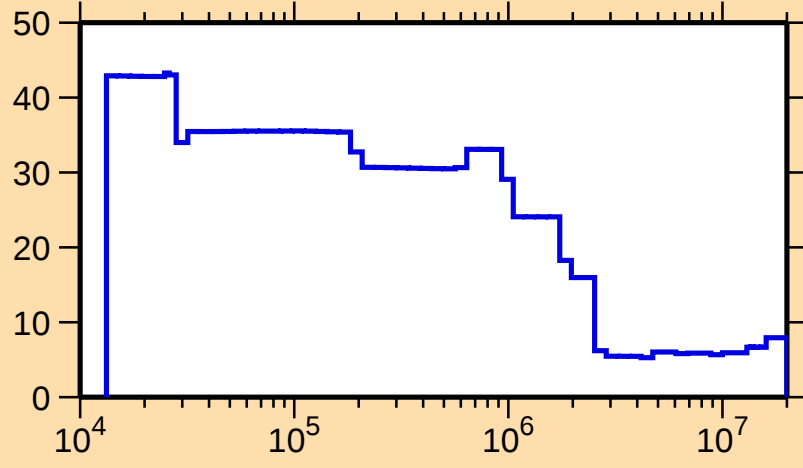
\Delta\sigma/\sigma vs. E for ^{146}\text{Eu}(n,\text{nonel.})
