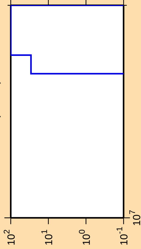
\Delta\sigma/\sigma vs. E for ^{146}\text{Eu} (mt 34)
