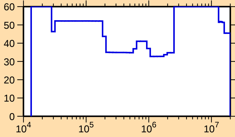
\Delta\sigma/\sigma vs. E for ^{146}\text{Eu}(n,n_1)
