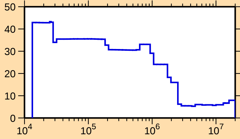
\Delta\sigma/\sigma vs. E for ^{146}\text{Eu}(n,\text{nonel.})
