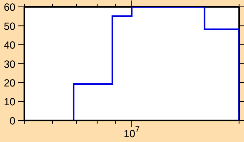
\Delta\sigma/\sigma vs. E for ^{146}\text{Eu}(n,\text{inel.})
