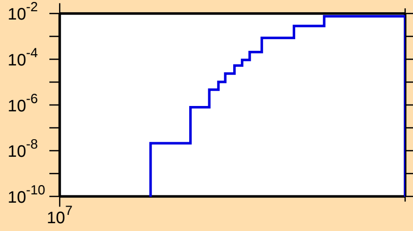
\sigma vs. E for ^{146}\text{Eu}(n,2np)
