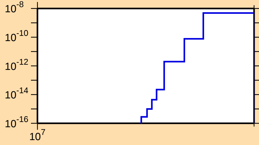
\sigma vs. E for ^{146}\text{Eu}(n,\text{pt})
