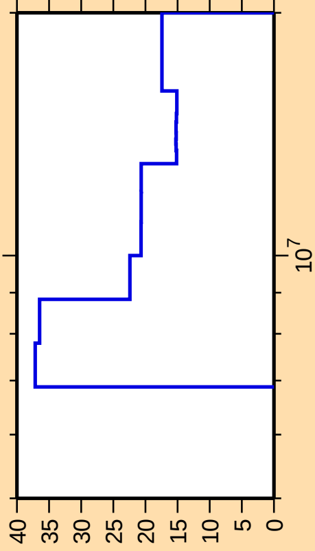
\Delta\sigma/\sigma vs. E for ^{146}\text{Eu}(n,2n)
