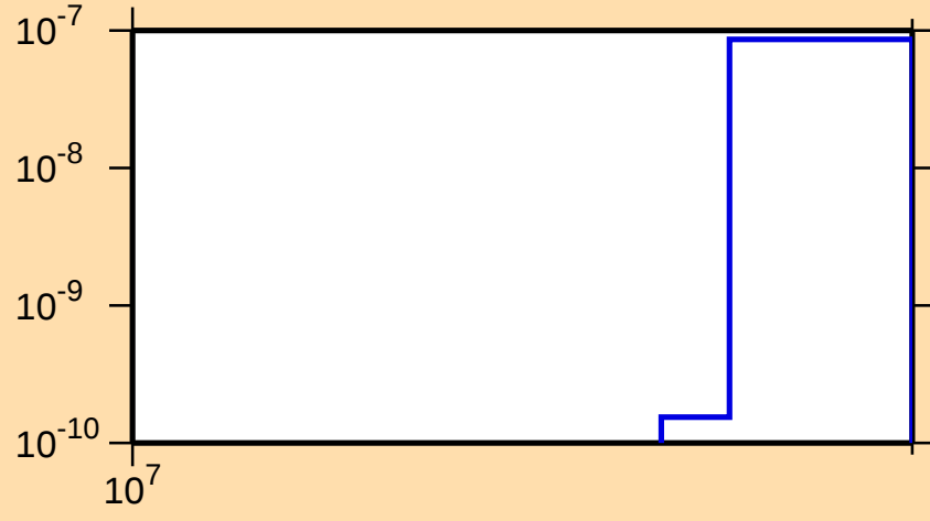
\sigma vs. E for ^{146}\text{Eu}(n,nt)
