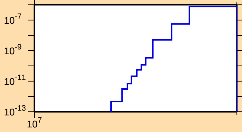
\sigma vs. E for ^{146}\text{Eu}(n,2n\alpha)
