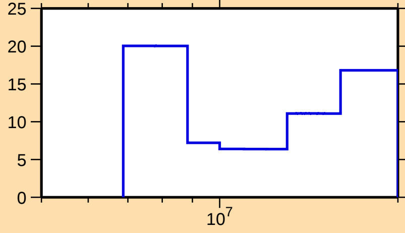
\Delta\sigma/\sigma vs. E for ^{146}\text{Eu}(n,\text{el.})
