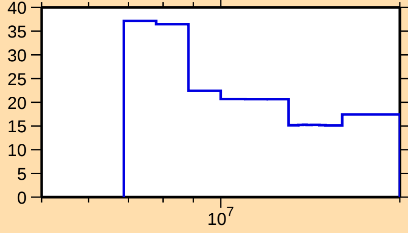
\Delta\sigma/\sigma vs. E for ^{146}\text{Eu}(n,2n)
