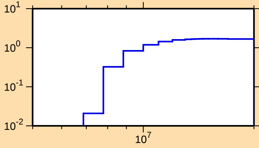
\sigma vs. E for ^{146}\text{Eu}(n,2n)
