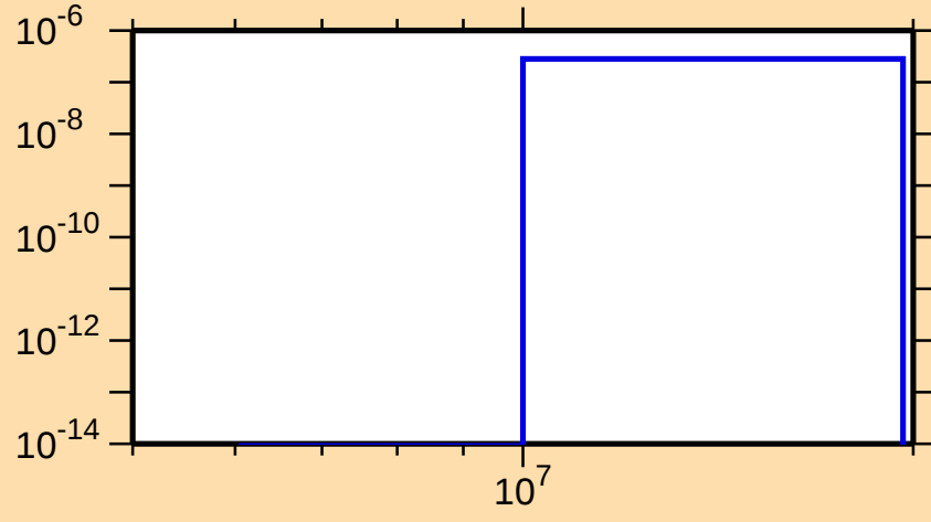
\sigma vs. E for ^{146}\text{Eu}(n,\text{He3})
