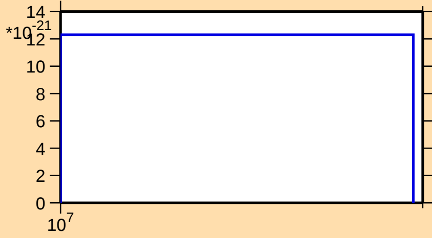
\sigma vs. E for ^{146}\text{Eu} (mt 11)
