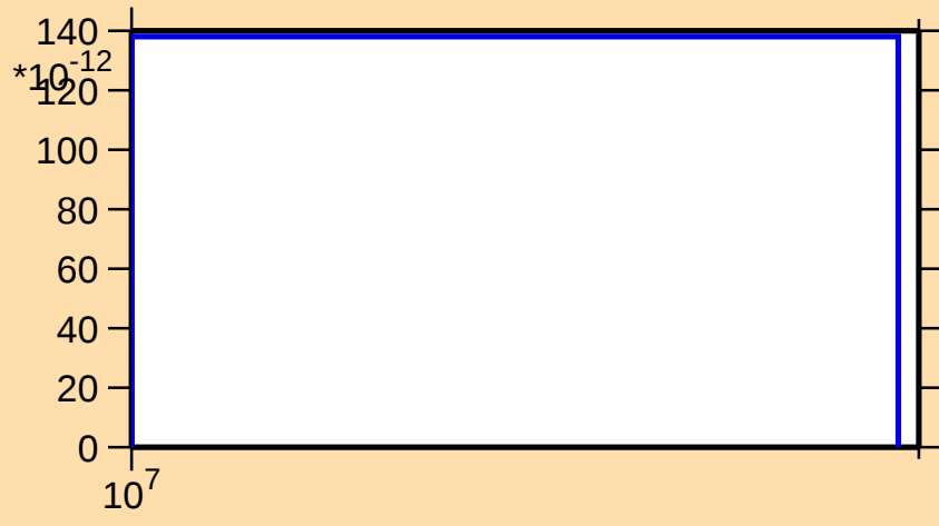
\sigma vs. E for ^{146}\text{Eu} (mt 45)
