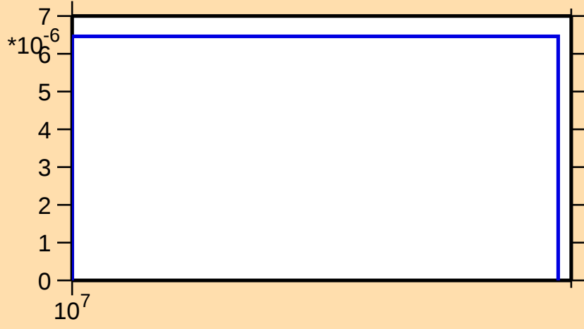
\sigma vs. E for ^{146}\text{Eu}(n,3n)
