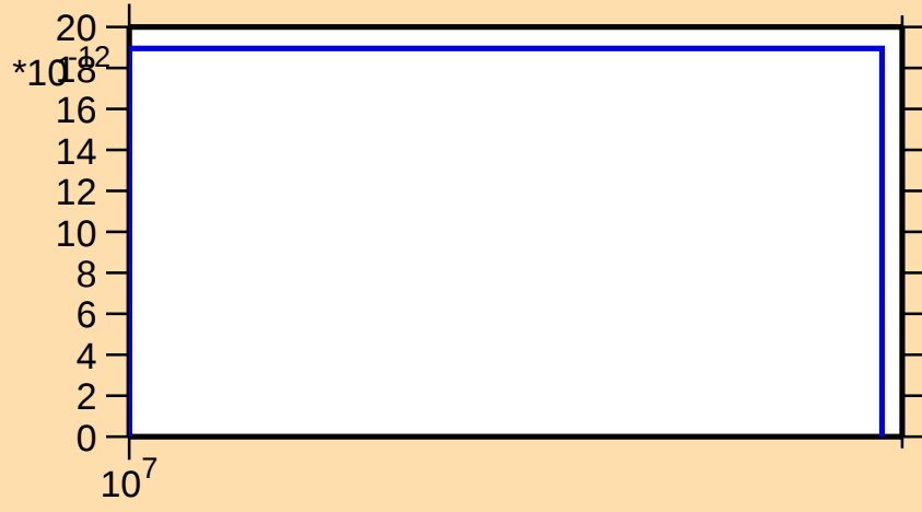
\sigma vs. E for ^{146}\text{Eu}(\text{mt117})
