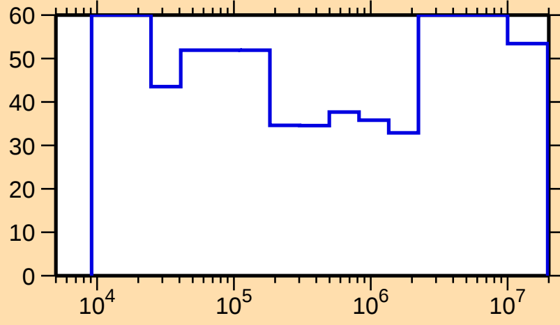
\Delta\sigma/\sigma vs. E for ^{146}\text{Eu}(n,n_1)
