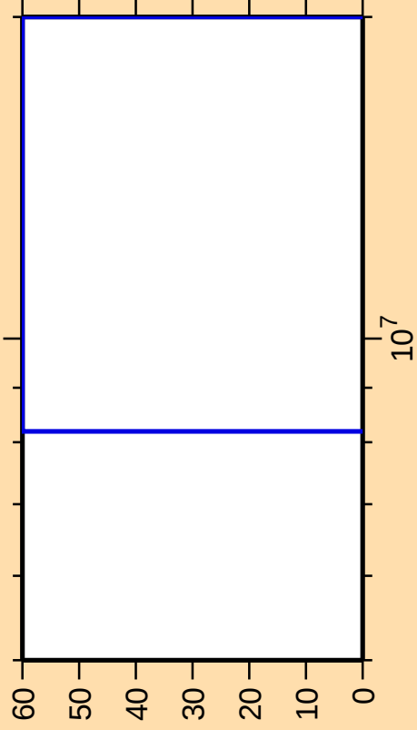
\Delta\sigma/\sigma vs. E for ^{146}\text{Eu}(n,pt)
