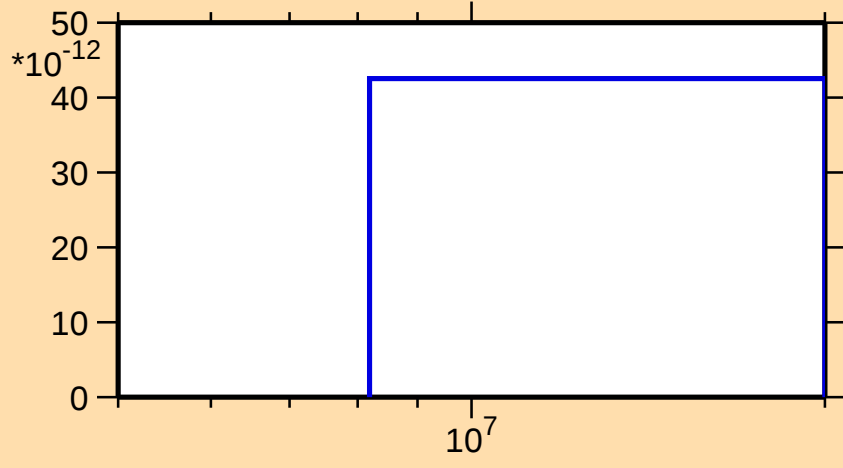
\sigma vs. E for ^{146}\text{Eu}(n,pt)
