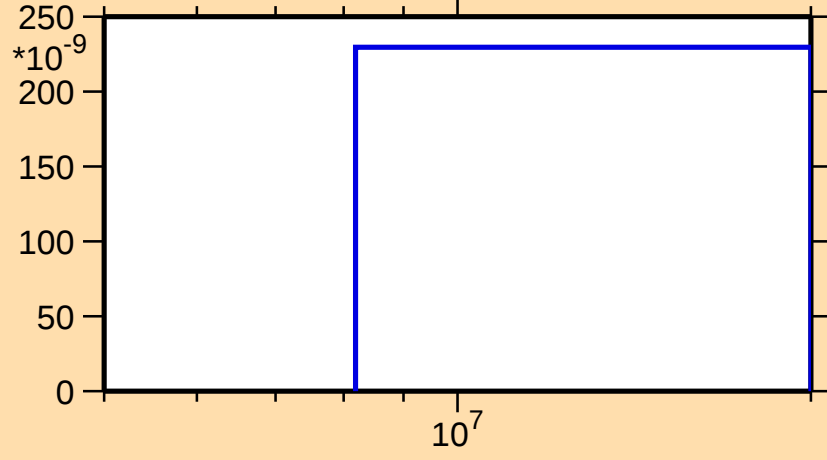
\sigma vs. E for ^{146}\text{Eu}(n,\text{He3})
