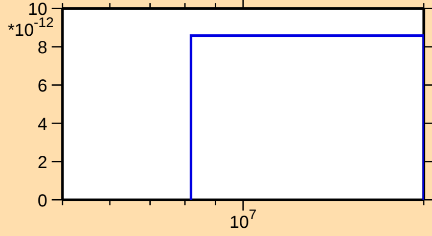
\sigma vs. E for ^{146}\text{Eu}(n,\text{pd})
