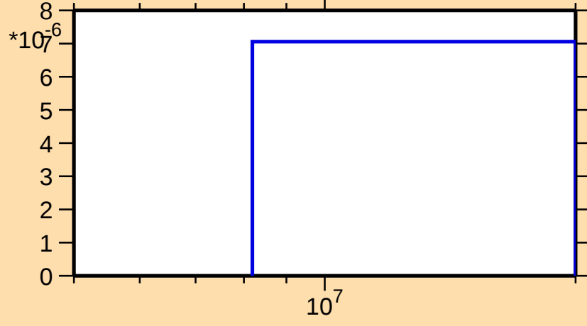
\sigma vs. E for ^{146}\text{Eu}(n,3n)
