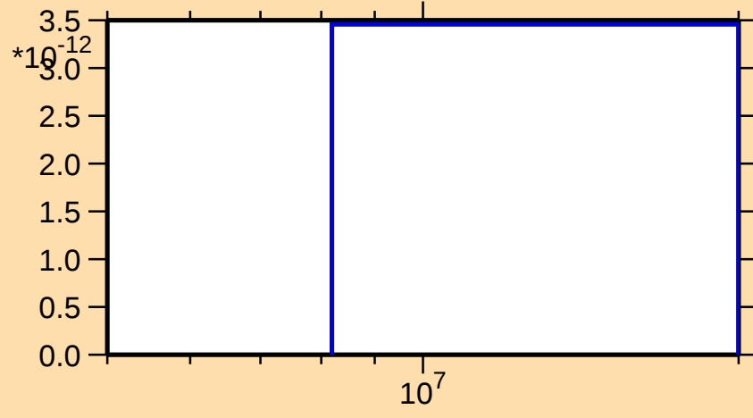
\sigma vs. E for ^{146}\text{Eu}(\text{mt } 34)
