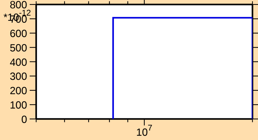
\sigma vs. E for ^{146}\text{Eu}(n,nt)
