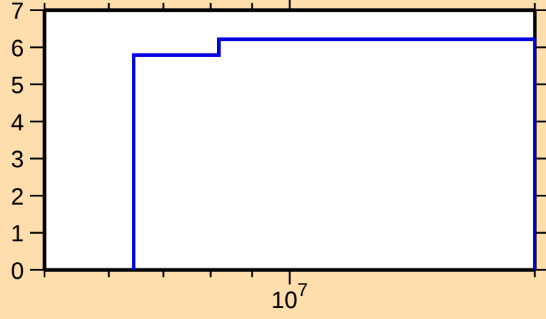
\Delta\sigma/\sigma vs. E for ^{146}\text{Eu}(n,\text{nonel.})
