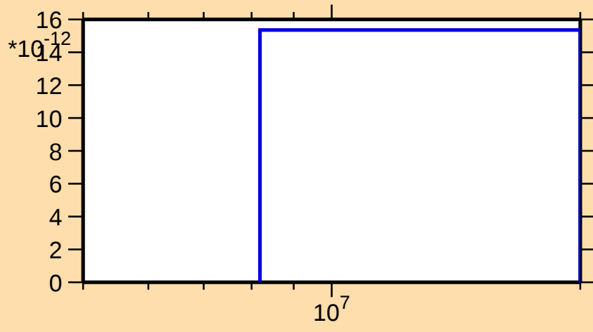
\sigma vs. E for ^{146}\text{Eu}(\text{mt117})
