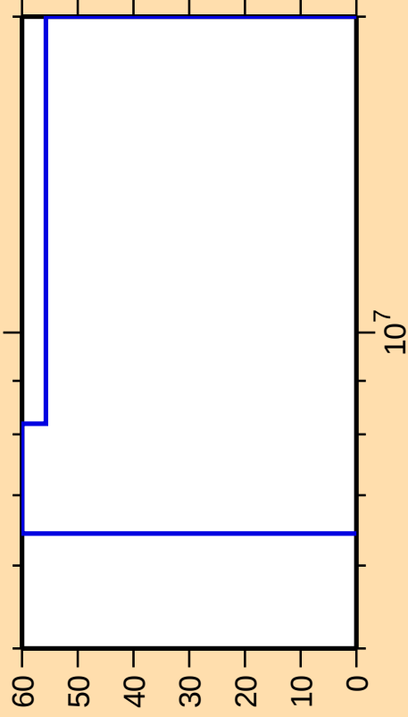
\Delta\sigma/\sigma vs. E for ^{146}\text{Eu}(n,n_1)
