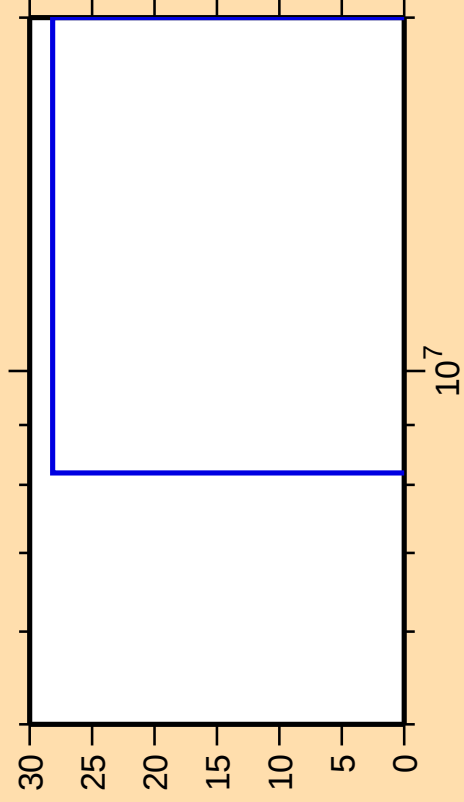
\Delta\sigma/\sigma vs. E for ^{146}\text{Eu}(\text{mt } 34)
