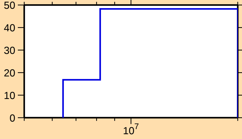
\Delta\sigma/\sigma vs. E for ^{146}\text{Eu}(n,\text{inel.})
