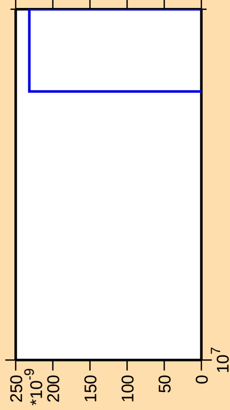
\Delta\sigma/\sigma vs. E for ^{155}\text{Eu} (mt 11)
