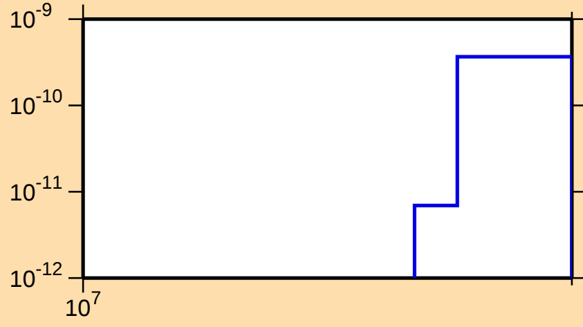
\sigma vs. E for ^{155}\text{Eu}(n,\text{He3})
