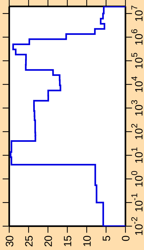
\Delta\sigma/\sigma vs. E for ^{155}\text{Eu}(n,\text{nonel.})
