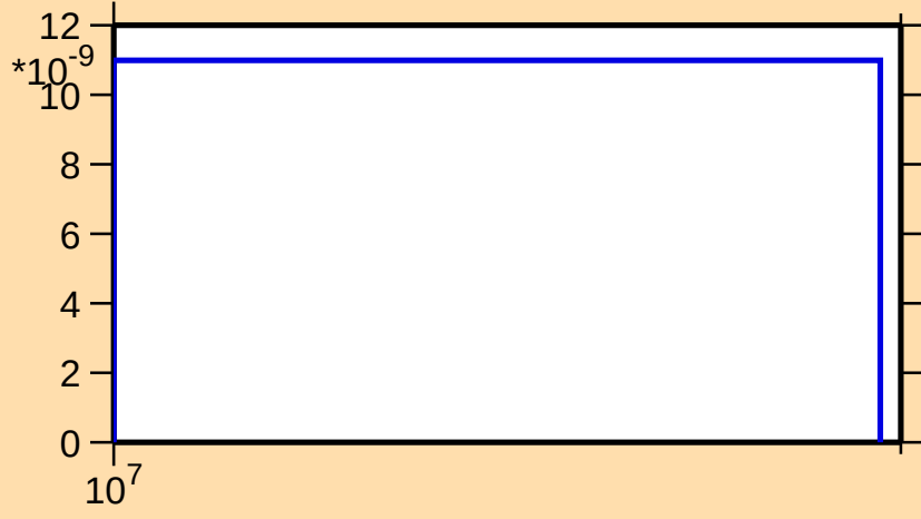
\sigma vs. E for ^{155}\text{Eu}(n,\text{nd})
