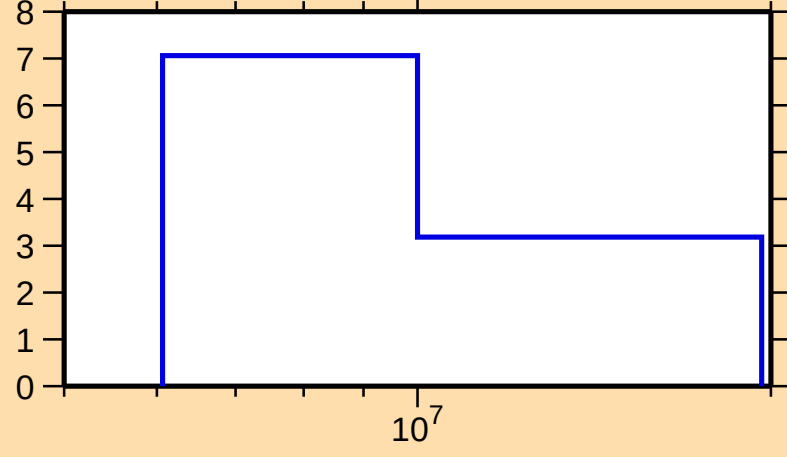
\Delta\sigma/\sigma vs. E for ^{155}\text{Eu}(n,\text{tot.})
