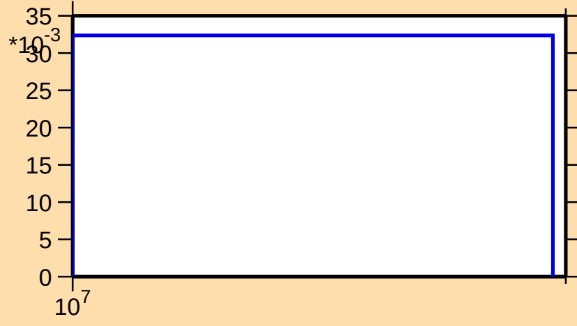
\sigma vs. E for ^{155}\text{Eu}(n,3n)
