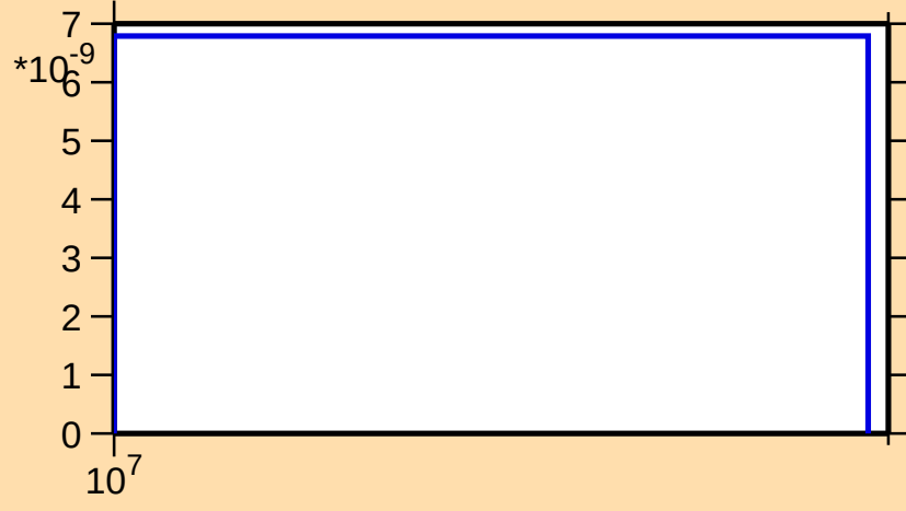
\sigma vs. E for ^{155}\text{Eu}(n,nt)
