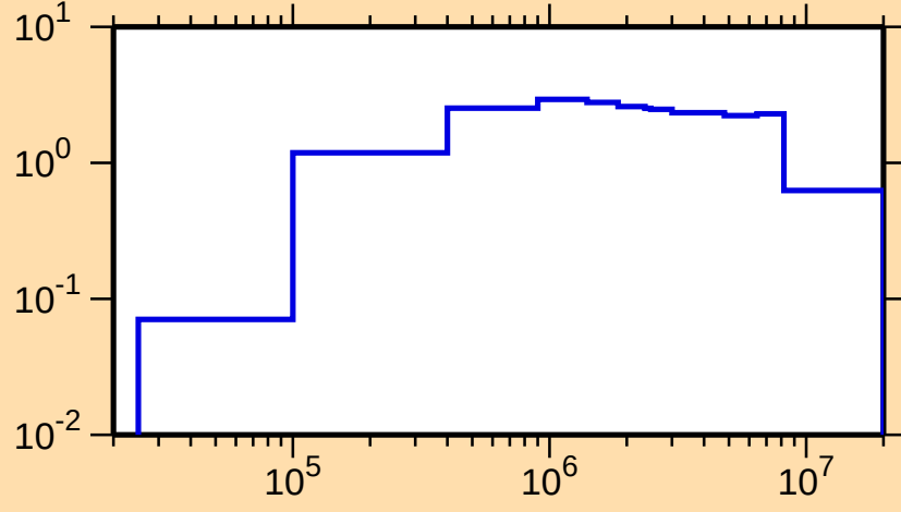
\sigma vs. E for ^{155}\text{Eu}(n,\text{inel.})
