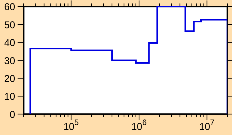
\Delta\sigma/\sigma vs. E for ^{155}\text{Eu}(n,n_1)
