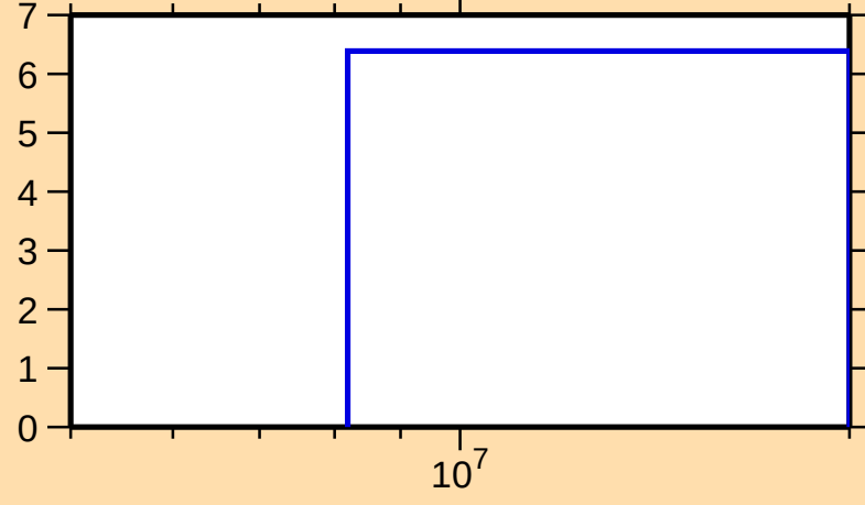
\Delta\sigma/\sigma vs. E for ^{155}\text{Eu}(n,\text{el.})
