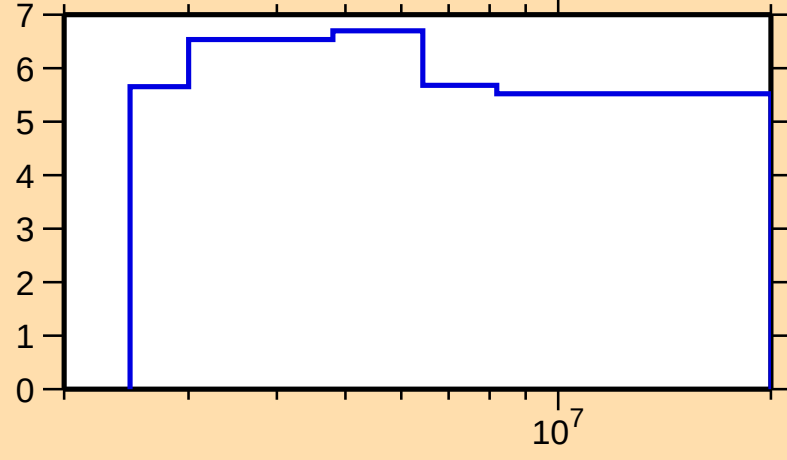
\Delta\sigma/\sigma vs. E for ^{155}\text{Eu}(n,\text{nonel.})
