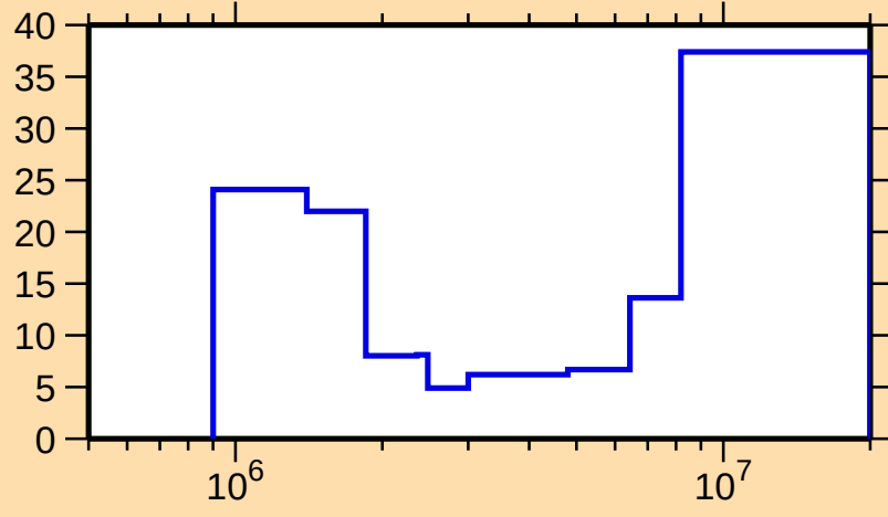
\Delta\sigma/\sigma vs. E for ^{155}\text{Eu}(n,n\text{cont.})
