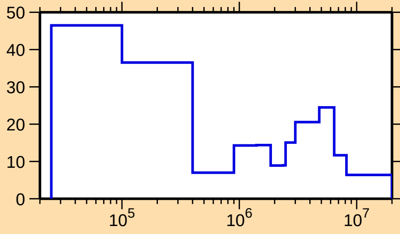
\Delta\sigma/\sigma vs. E for ^{155}\text{Eu}(n,\text{el.})
