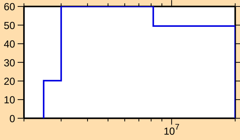
\Delta\sigma/\sigma vs. E for ^{155}\text{Eu}(n,p)
