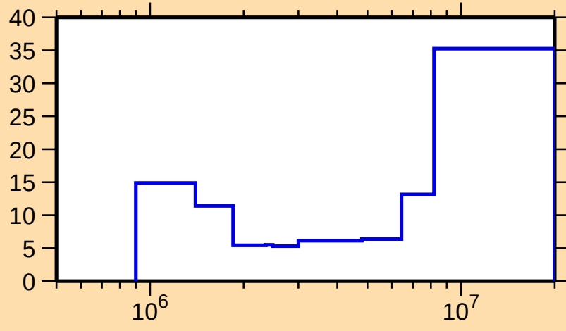
\Delta\sigma/\sigma vs. E for ^{155}\text{Eu}(n,\text{inel.})
