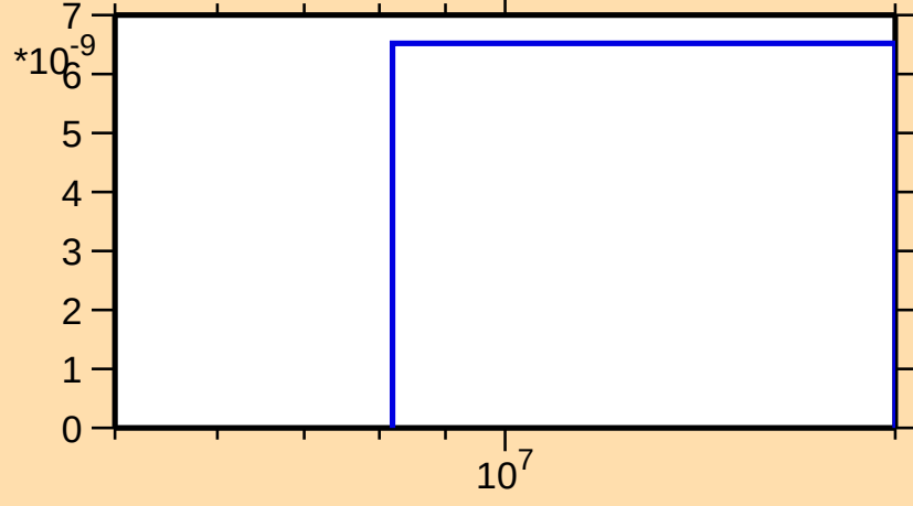
\sigma vs. E for ^{155}\text{Eu}(n,nt)
