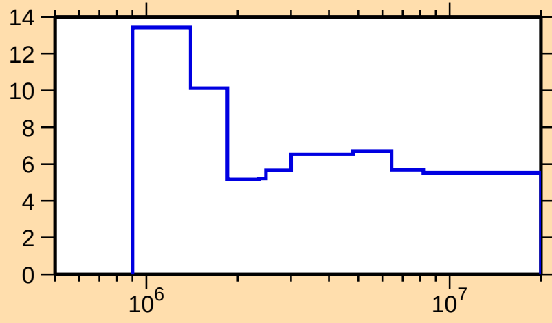
\Delta\sigma/\sigma vs. E for ^{155}\text{Eu}(n,\text{nonel.})
