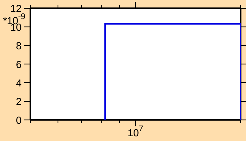
\sigma vs. E for ^{155}\text{Eu}(n,nd)
