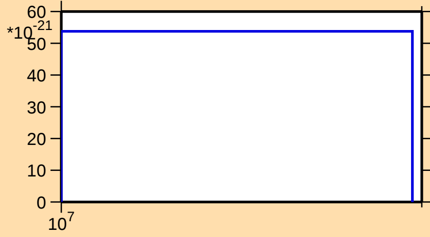
\sigma vs. E for ^{159}\text{Eu} (mt 11)
