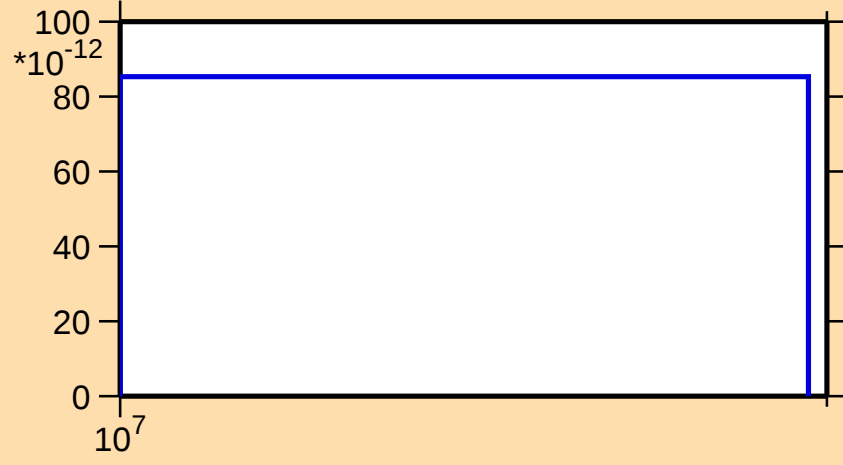
\sigma vs. E for ^{159}\text{Eu}(n,2n\alpha)
