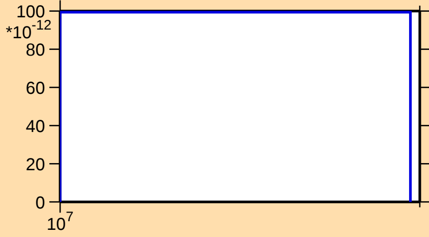
\sigma vs. E for ^{159}\text{Eu}(n,2np)
