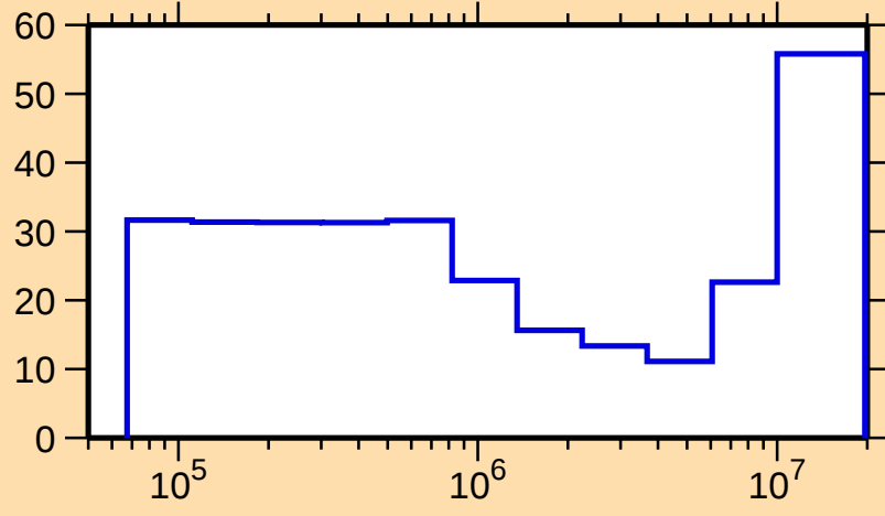
\Delta\sigma/\sigma vs. E for ^{159}\text{Eu}(n,\text{inel.})
