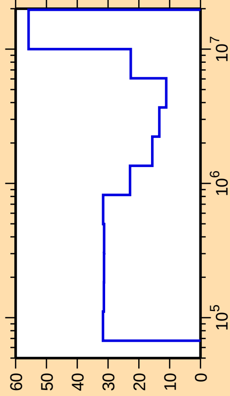
\Delta\sigma/\sigma vs. E for ^{159}\text{Eu}(n,\text{inel.})
