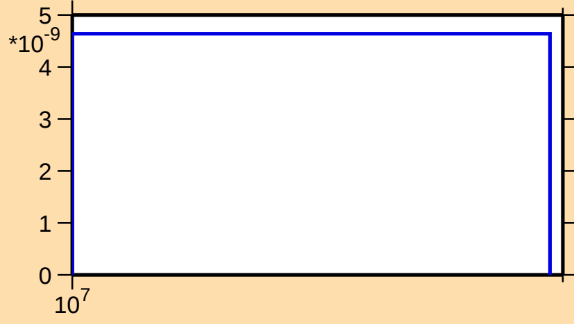
\sigma vs. E for ^{159}\text{Eu}(n,\text{nd})
