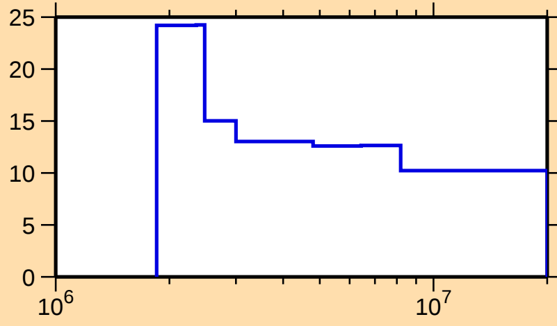
\Delta\sigma/\sigma vs. E for ^{159}\text{Eu}(n,\text{tot.})
