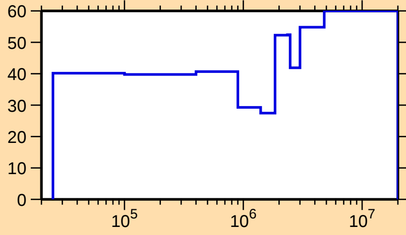
\Delta\sigma/\sigma vs. E for ^{159}\text{Eu}(n,n_1)
