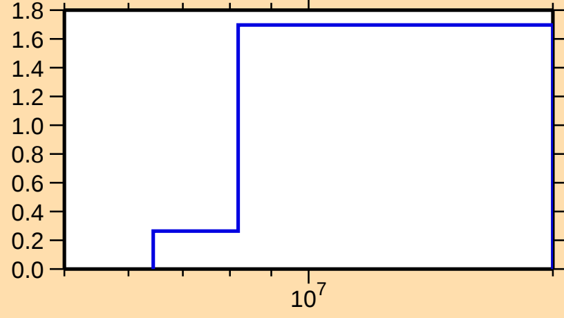
\sigma vs. E for ^{159}\text{Eu}(n,2n)
