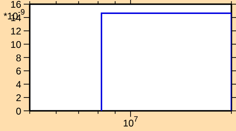
\sigma vs. E for ^{159}\text{Eu}(n,nt)
