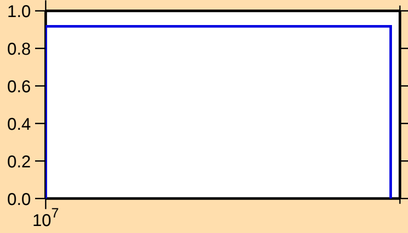
\sigma vs. E for ^{162}\text{Eu}(n,3n)
