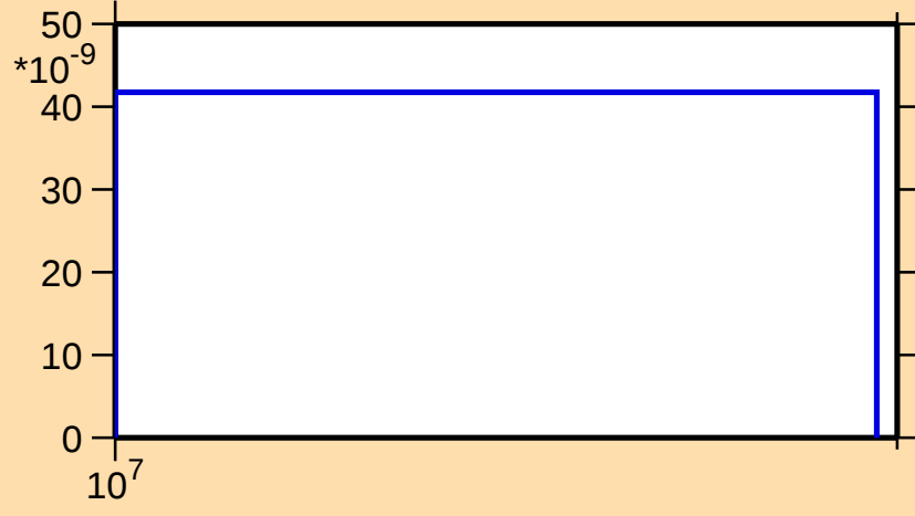
\sigma vs. E for ^{162}\text{Eu}(n,\text{nd})
