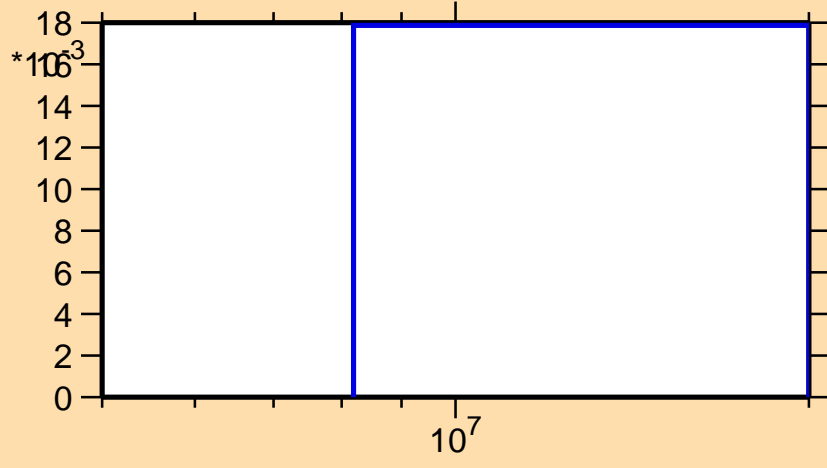
\sigma vs. E for ^{21}\text{F}(n,d)
