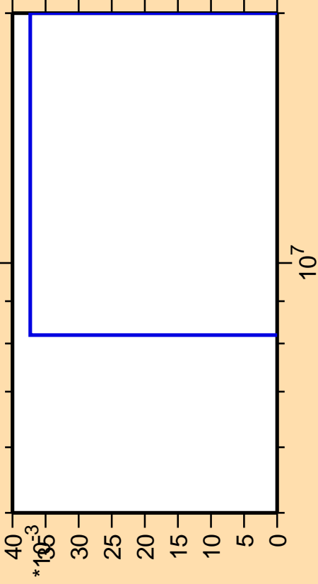
\Delta\sigma/\sigma vs. E for ^{21}\text{F}(n,2np)
