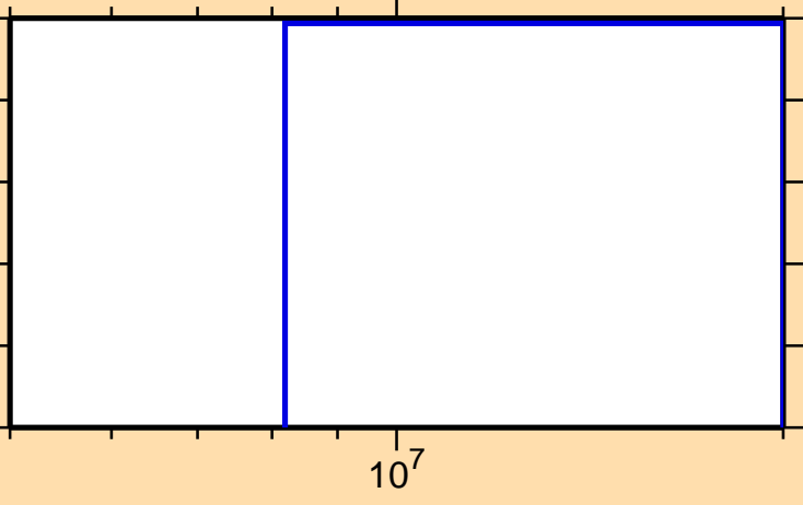
\sigma vs. E for ^{21}\text{F}(n,nt)
