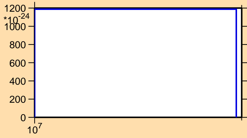
\sigma vs. E for ^{53}\text{Fe}(n,2n\alpha)
