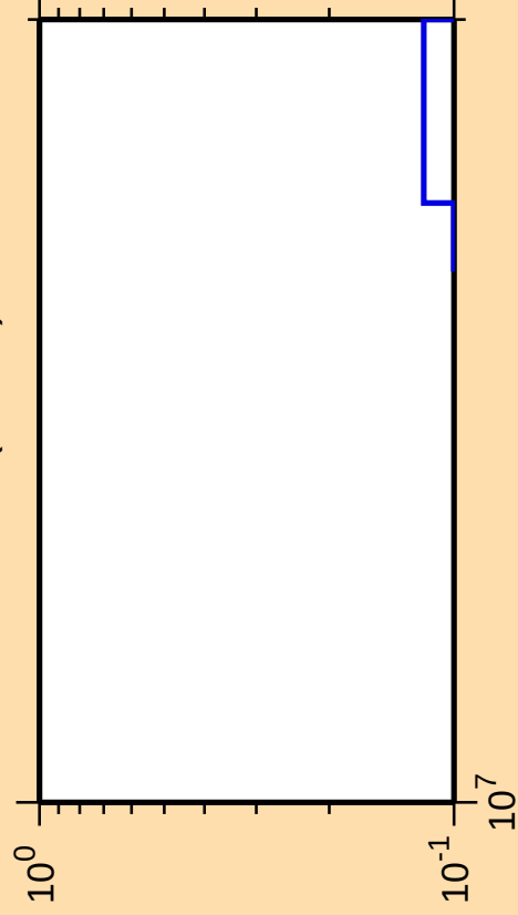
\Delta\sigma/\sigma vs. E for ^{53}\text{Fe}(n,2n\alpha)
