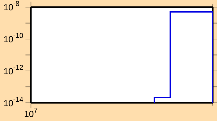
\sigma vs. E for ^{53}\text{Fe}(\text{mt } 45)
