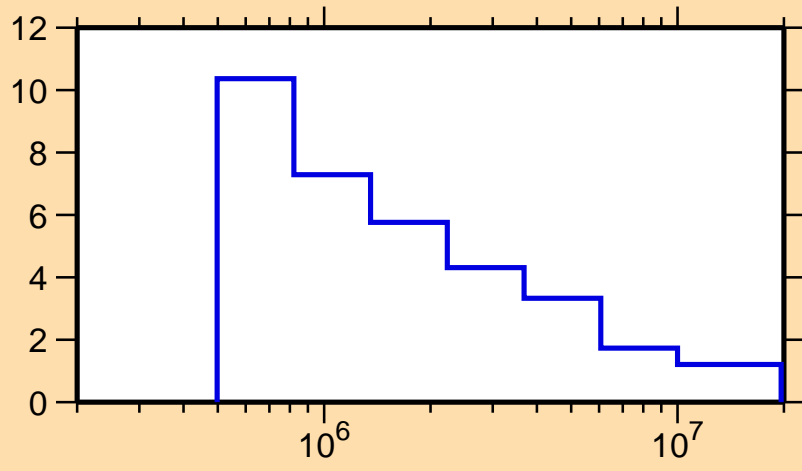
\Delta\sigma/\sigma vs. E for ^{53}\text{Fe}(n,n\text{onel.})
