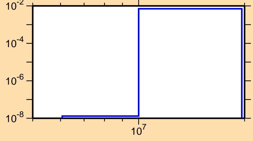
\sigma vs. E for ^{53}\text{Fe}(n,\alpha)
