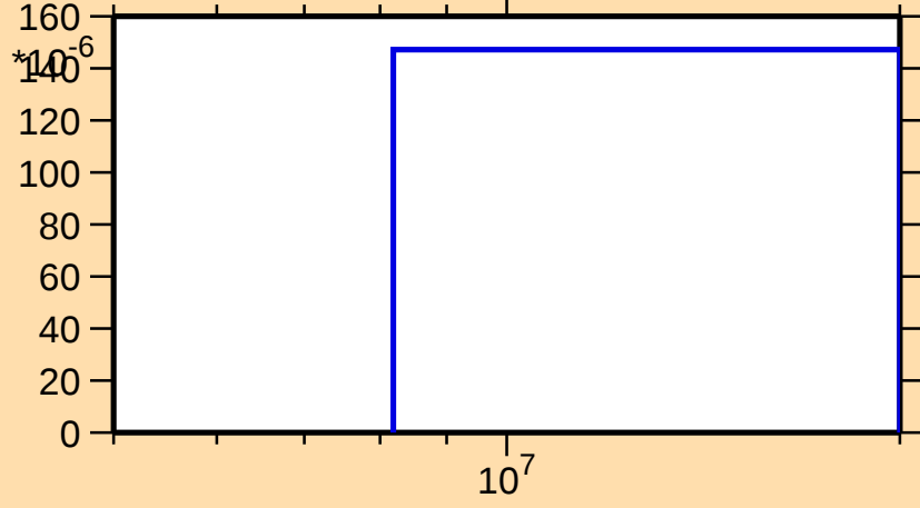
\sigma vs. E for ^{55}\text{Fe}(n,t)
