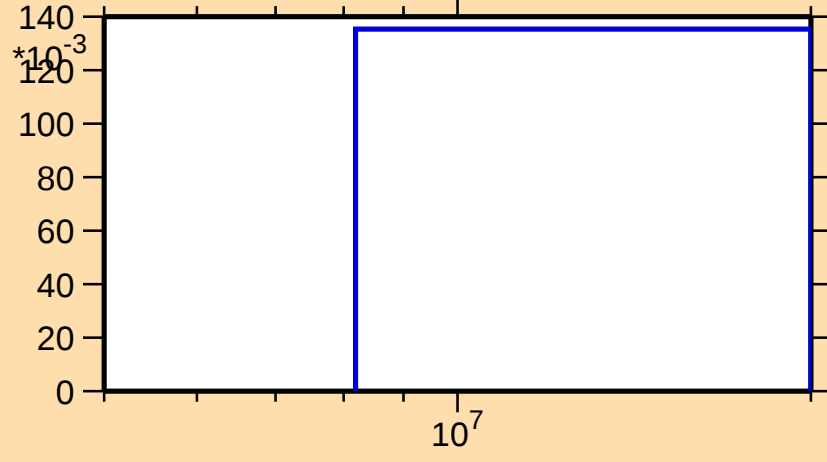
\sigma vs. E for ^{55}\text{Fe}(n,np)
