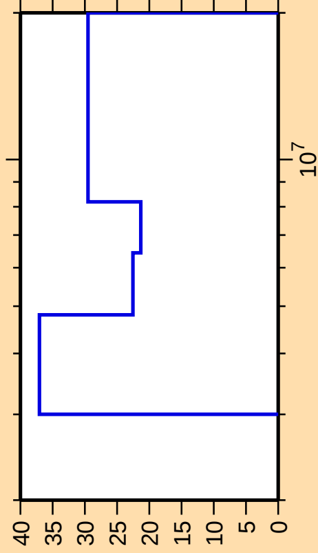
\Delta\sigma/\sigma vs. E for ^{55}\text{Fe}(n,\text{ncont.})
