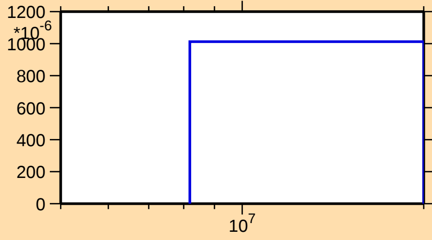
\sigma vs. E for ^{55}\text{Fe}(n,n\alpha)
