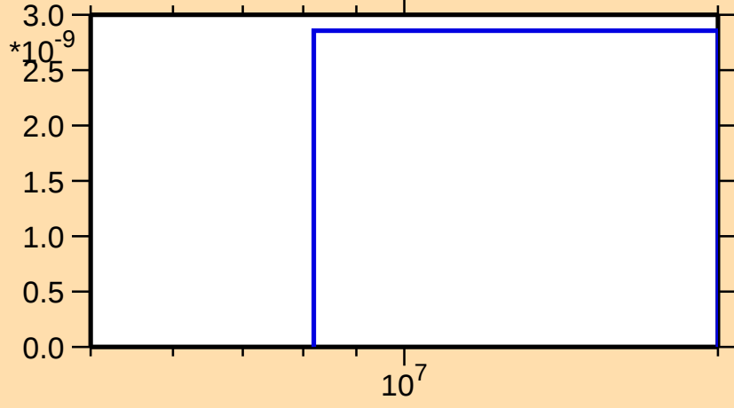
\sigma vs. E for ^{55}\text{Fe}(n,2np)
