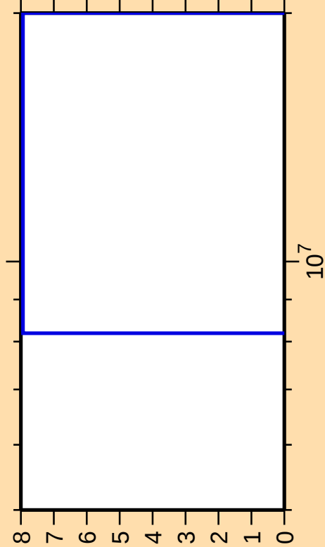
\Delta\sigma/\sigma vs. E for ^{55}\text{Fe}(\text{n},\text{pt})
