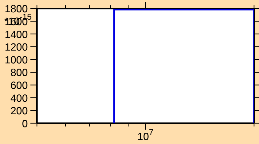
\sigma vs. E for ^{55}\text{Fe}(\text{n},\text{pt})
