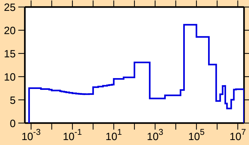
\Delta\sigma/\sigma vs. E for ^{55}\text{Fe}(\text{n,tot.})
