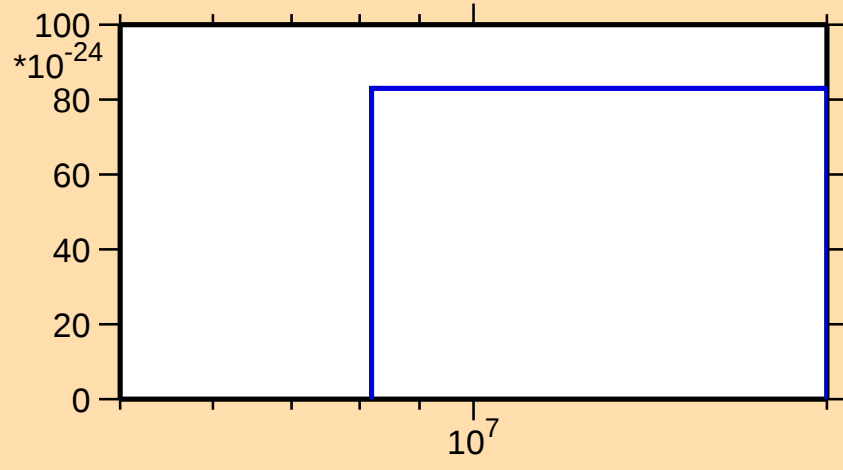
\sigma vs. E for ^{55}\text{Fe}(\text{mt } 45)
