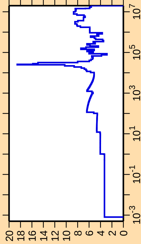
\Delta\sigma/\sigma vs. E for ^{56}\text{Fe}(\text{n,el.})
